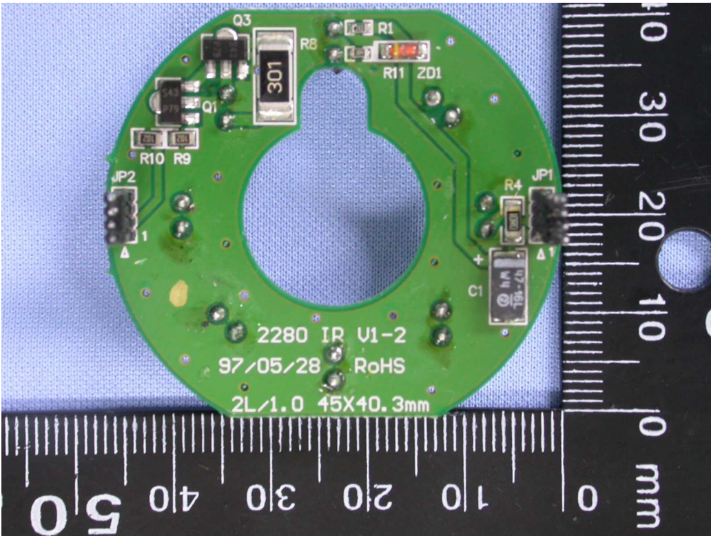
20. Rear view of PCB4
