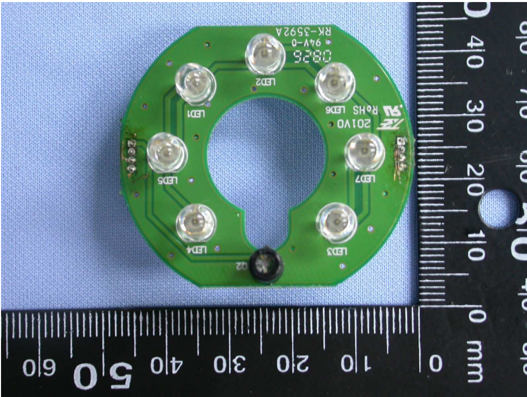
19. Front view of PCB4
