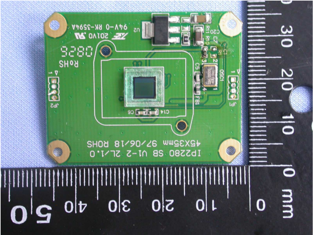
21. Front view of PCB5
