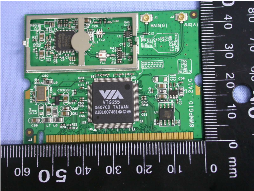
15. Front view of PCB2
