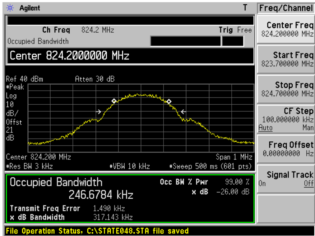
Figure Channel 128 (824.20MHz)
