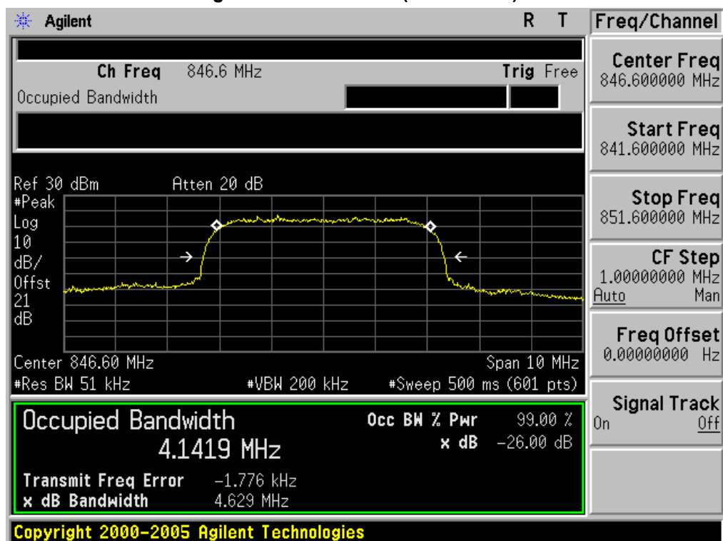
Figure Channel 4233 (846.60MHz)
