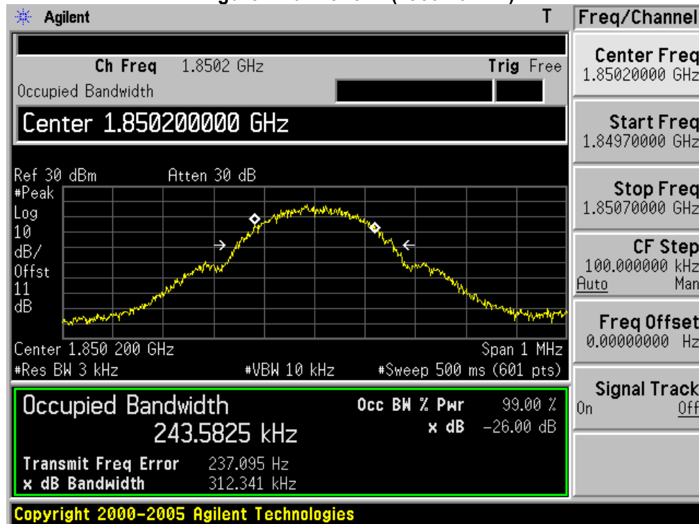
Figure Channel 512 (1850.20MHz)
