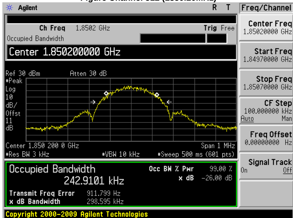
Figure Channel 512 (1850.20MHz)
