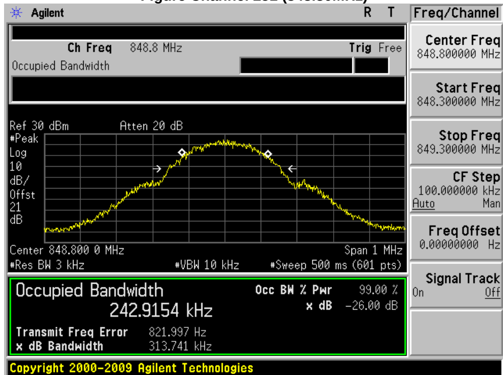
Figure Channel 251 (848.80MHz)
