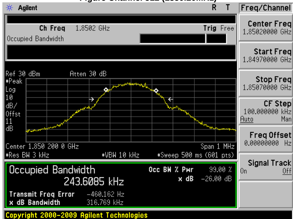
Figure Channel 512 (1850.20MHz)
