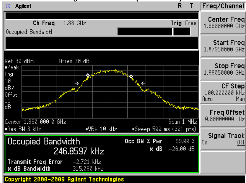
Figure Channel 661 (1880.00MHz)
