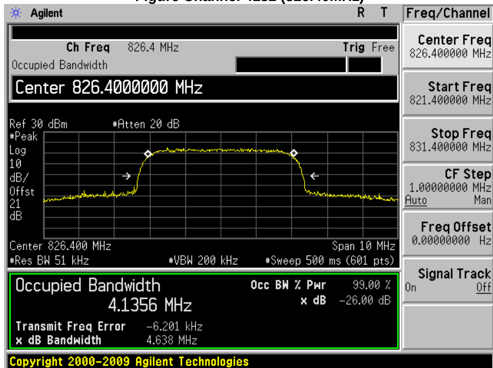
Figure Channel 4132 (826.40MHz)
