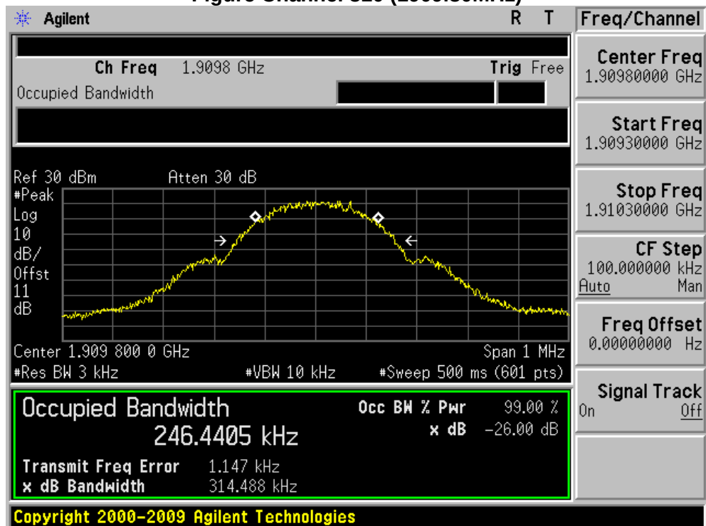
Figure Channel 810 (1909.80MHz)
