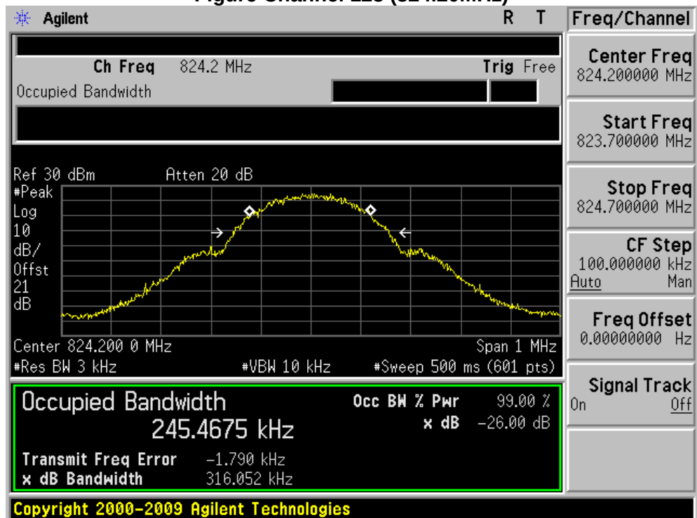
Figure Channel 128 (824.20MHz)
