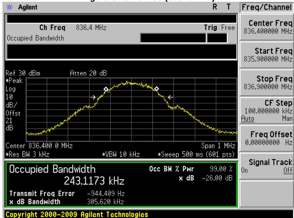
Figure Channel 189 (836.40MHz)
