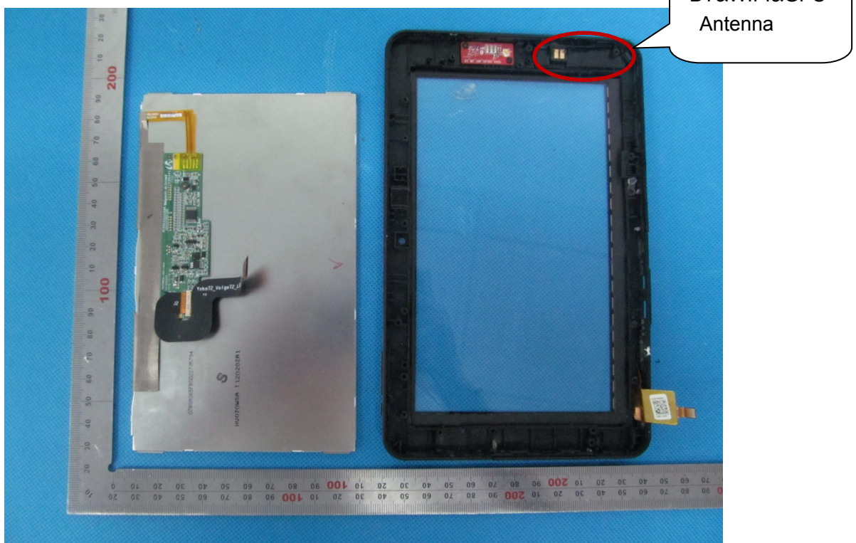
INTERNAL VIEW OF EUT-1
