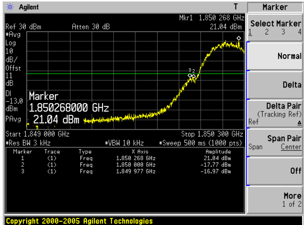
Figure Channel 512 (1850.20MHz)
