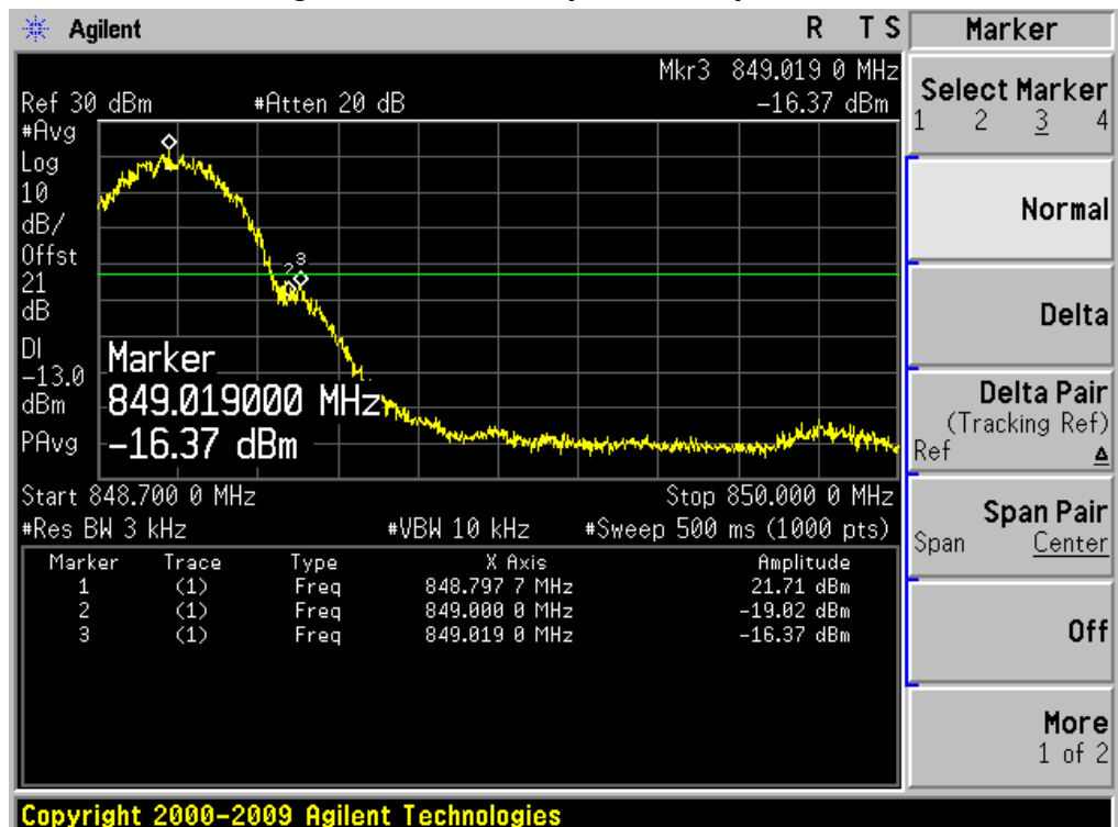
Figure Channel 251 (848.80MHz)
