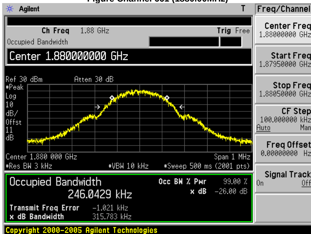
Figure Channel 661 (1880.00MHz)
