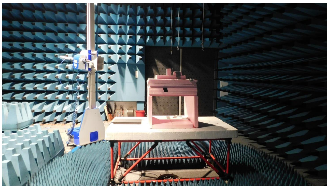
Picture 6: AC, radiated emission test 1 GHz – 18 GHz (rear view)
