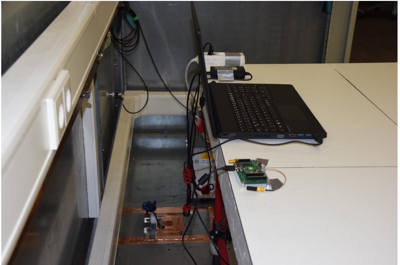
Picture 9: Test setup AC power line conducted emissions (rear view)
