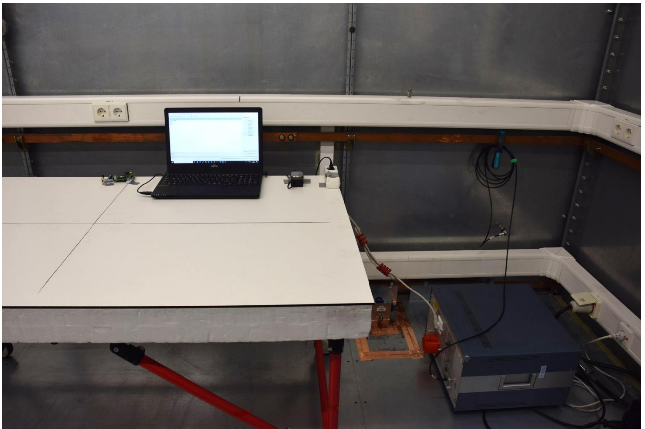
Picture 8: Test setup AC power line conducted emissions (front view)
