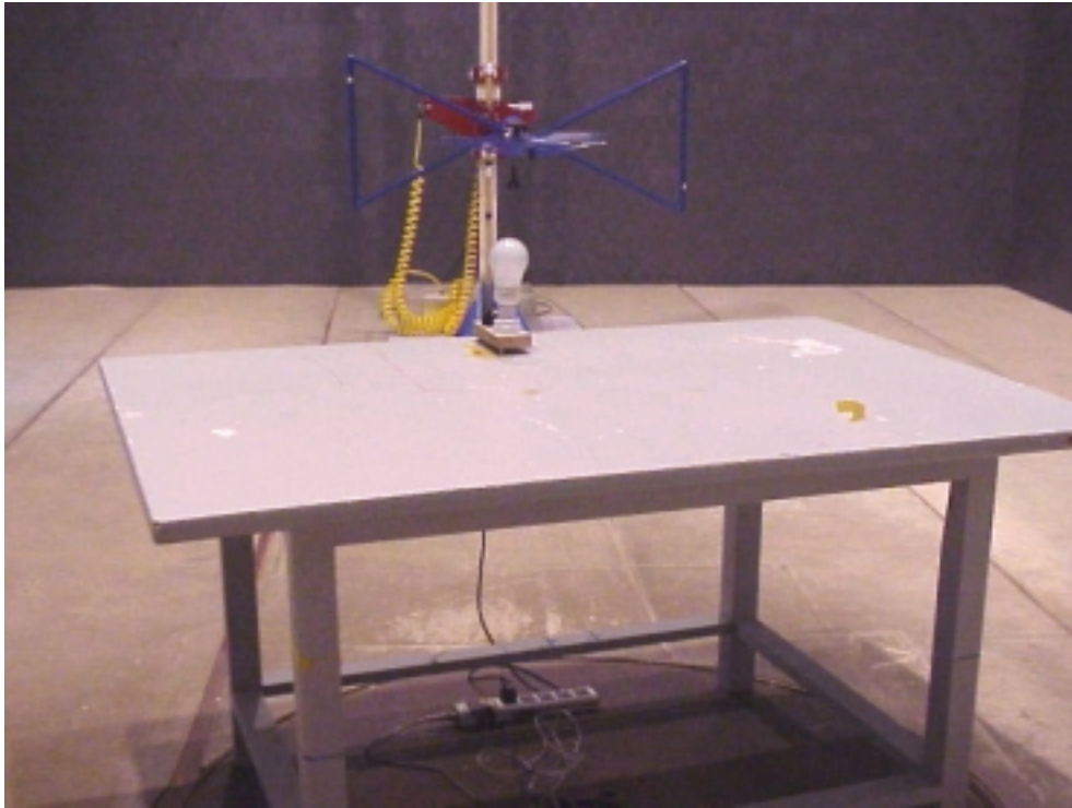
HORIZONTAL (M/N: TP120-AL SERIES)
