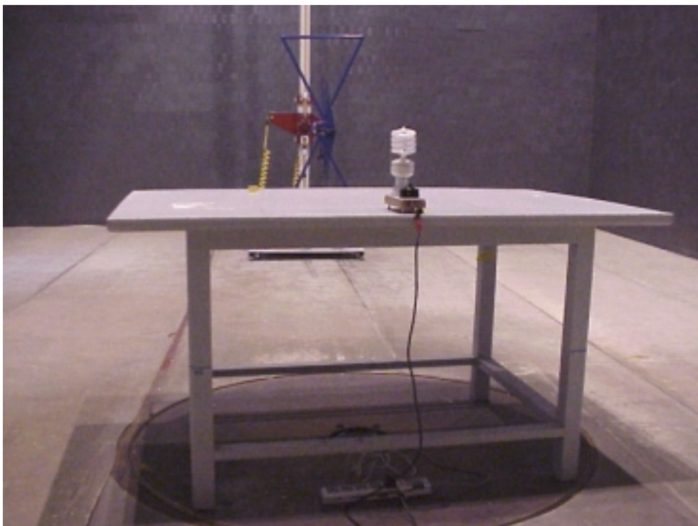
VERTICAL (M/N: TP120-SL SERIES)
