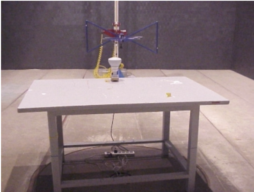
HORIZONTAL (M/N: TP120-RLF SERIES)
