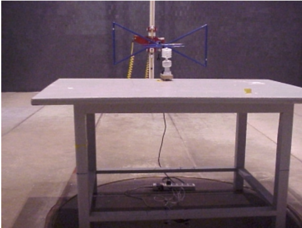
HORIZONTAL (M/N: TP120-SL SERIES)
