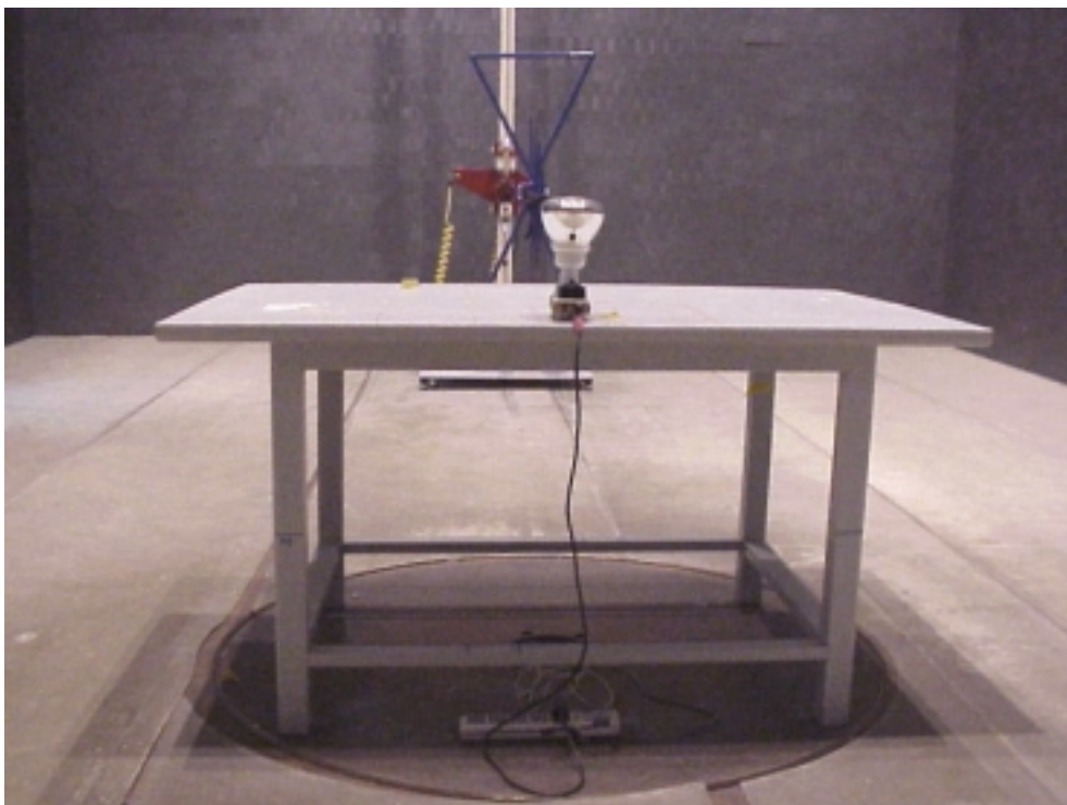
VERTICAL (M/N: TP120-RLC SERIES)
