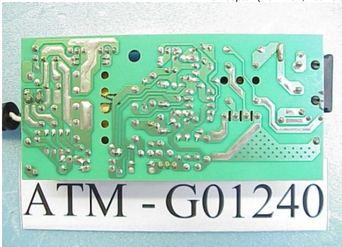
Figure 32 AC Adapter (PCB View, Back Side)
