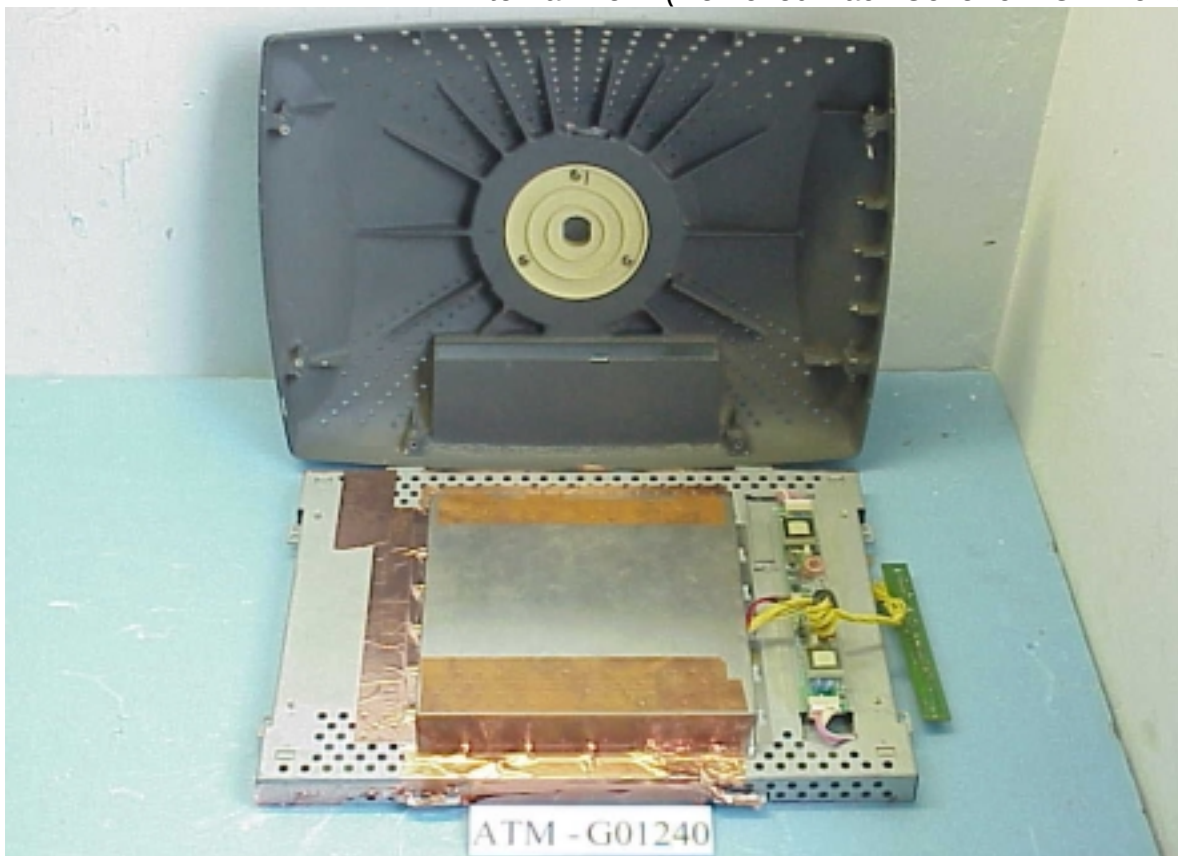
Figure 10 Internal View (Removed Back Cover of LCD Monitor)
