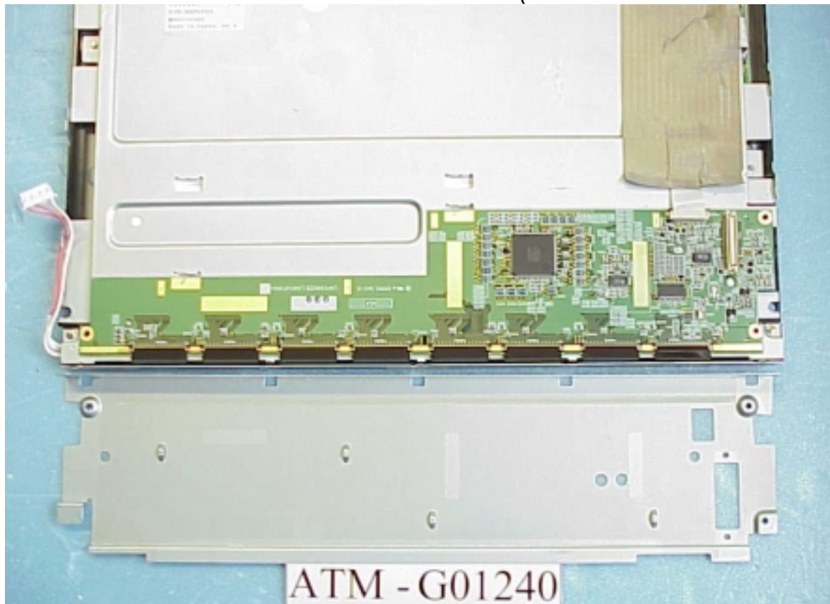
Figure 26 Internal View (LCD Panel, Back Side)
