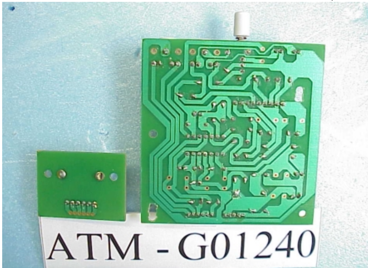
Figure 7 Audio Switch · Audio Control Board (Back Side)
