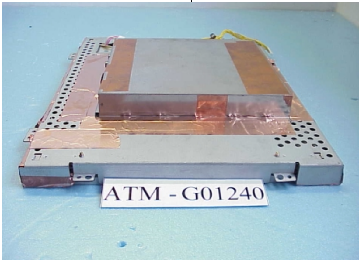
Figure 18 Internal View (Main Board & LCD Panel & Metal Cover)
