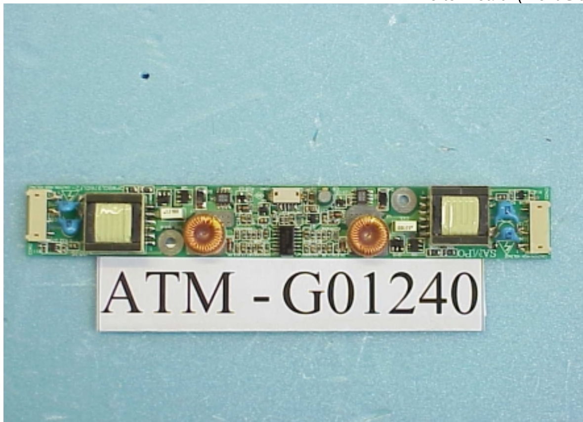
Figure 14 Inverter Board (Front Side)
