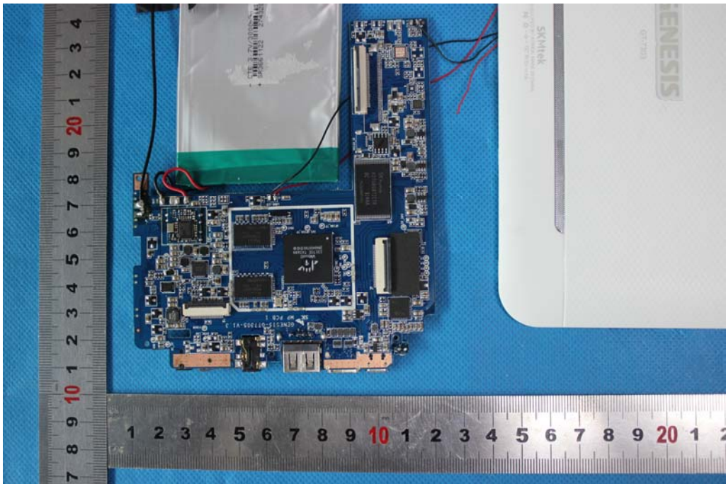
EUT – PCB View 3
