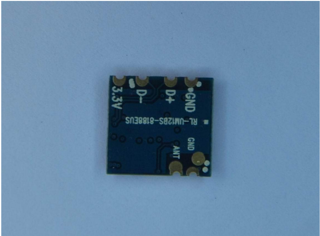
EUT – PCB View 4
