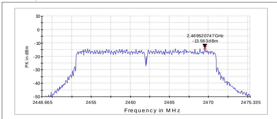
Channel 11 / 2462 MHz
