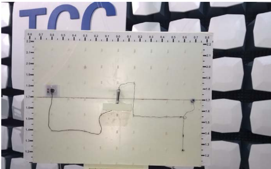
Picture 2. FCC Part 15B Radiated emissions
