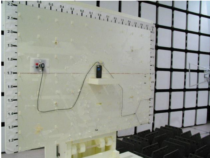
Picture 2. FCC Part 15B Radiated emissions
