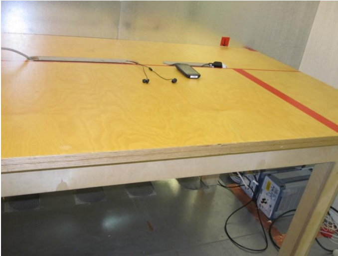
Picture 3. FCC Part 15C AC powerline conducted emissions
