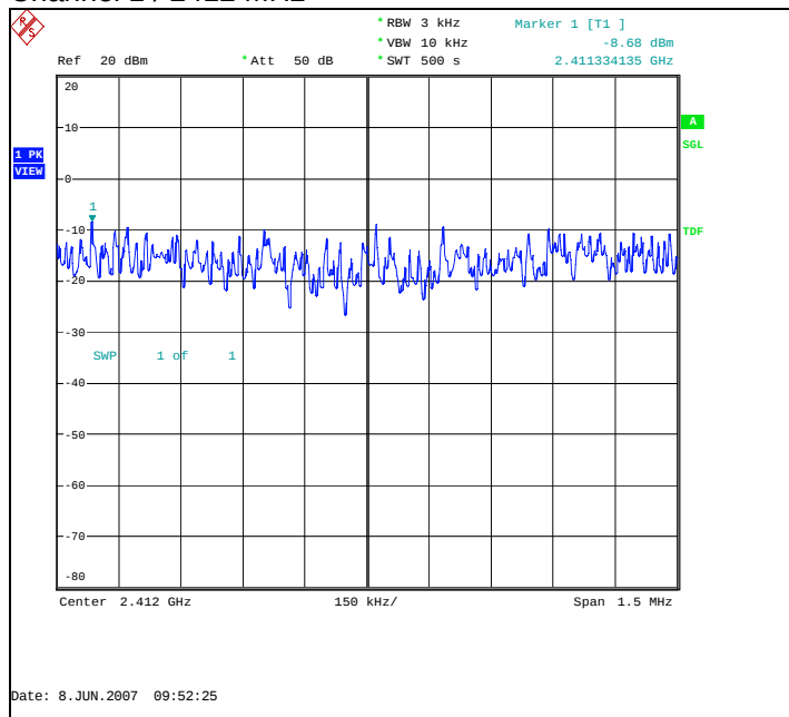
Channel 1 / 2412 MHz
