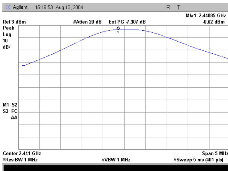
Picture 21: Peak output power, channel 39
