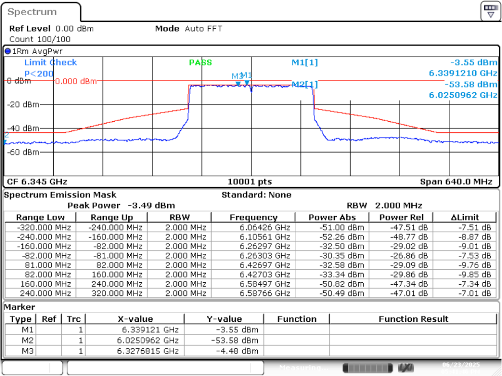
UNI5 SISO A 802.11ax160 ch79 6345MHz
