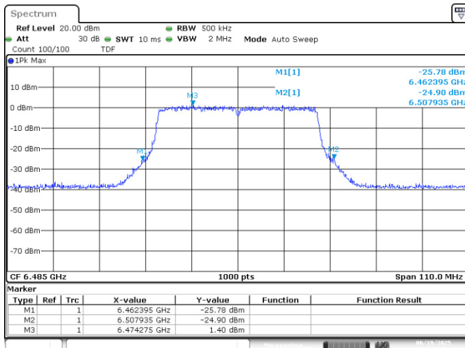
UNII6 SISO B 802.11ax40 ch107 6485MHz 26dB
