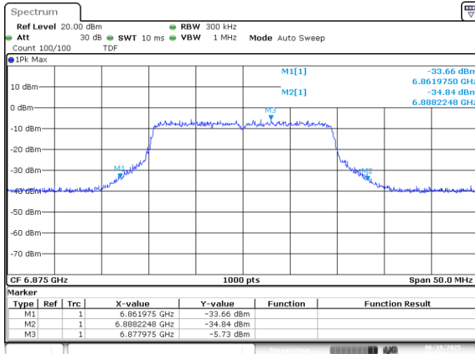
UNII8 MIMO B 802.11ax20 ch185 6875MHz 26dB
