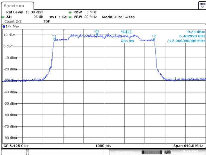
UNII5 SISO A 802.11be320 ch95 6425MHz 99%
