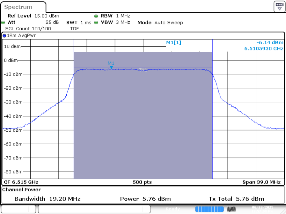
UNII6 SISO B 802.11ax20 ch113 6515MHz
