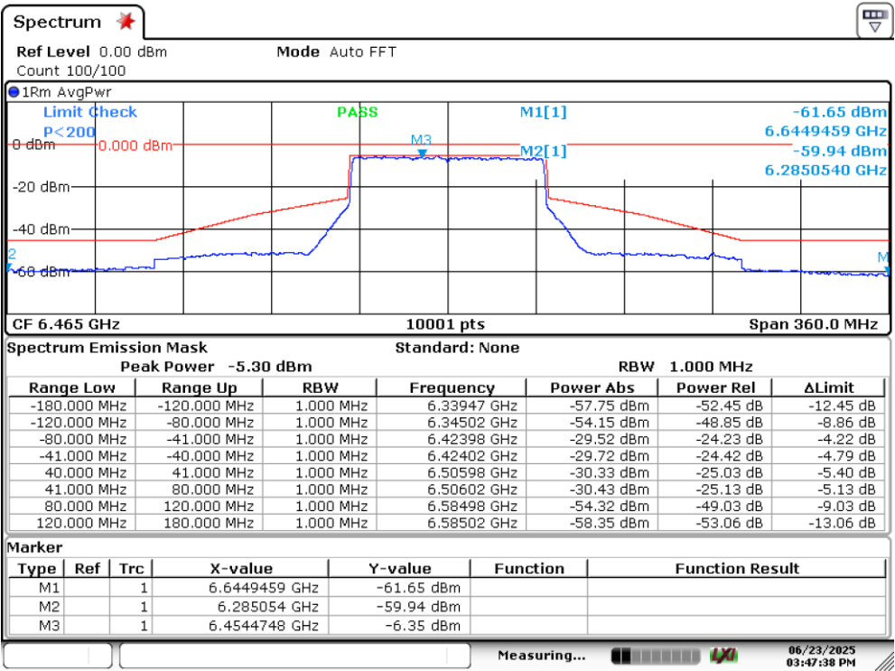
UNI6 SISO B 802.11ax80 ch103 6465MHz
