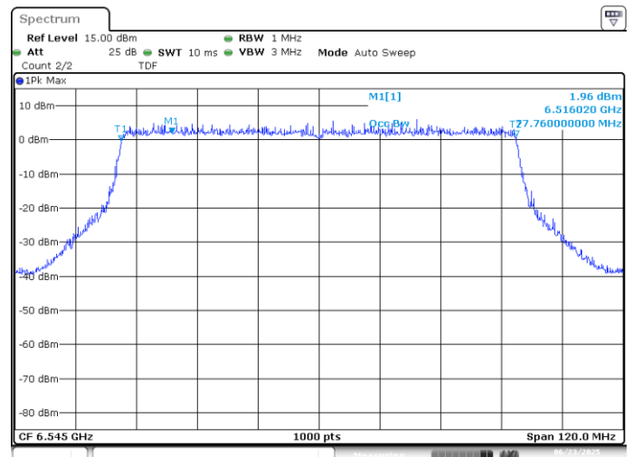
UNII6 SISO A 802.11ax80 ch119 6545MHz 99%
