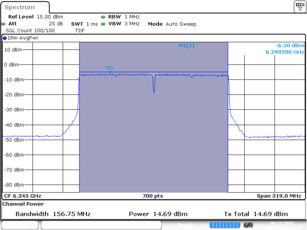
UNII5 SISO A 802.11ax160 ch79 6345MHz
