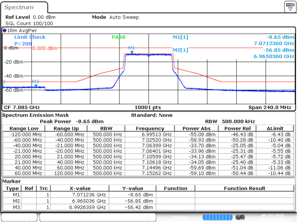
UNI8 SISO B 802.11ax40 ch227 7085MHz
