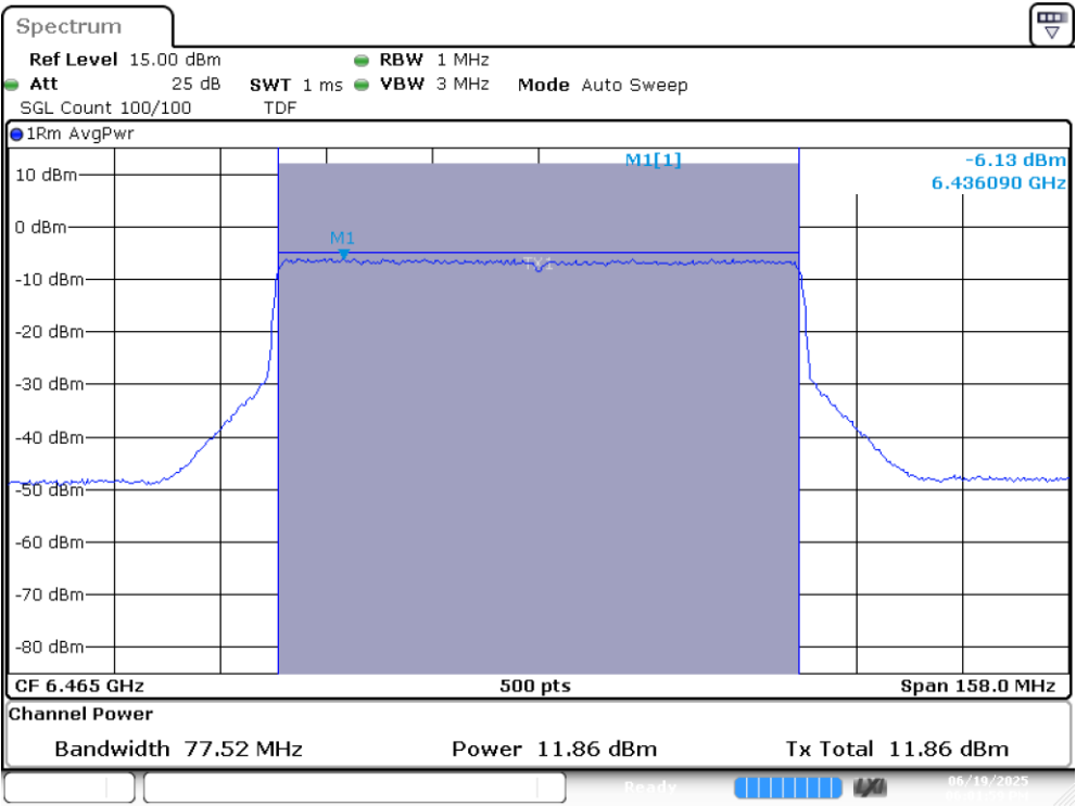
UNII6 SISO B 802.11ax80 ch103 6465MHz
