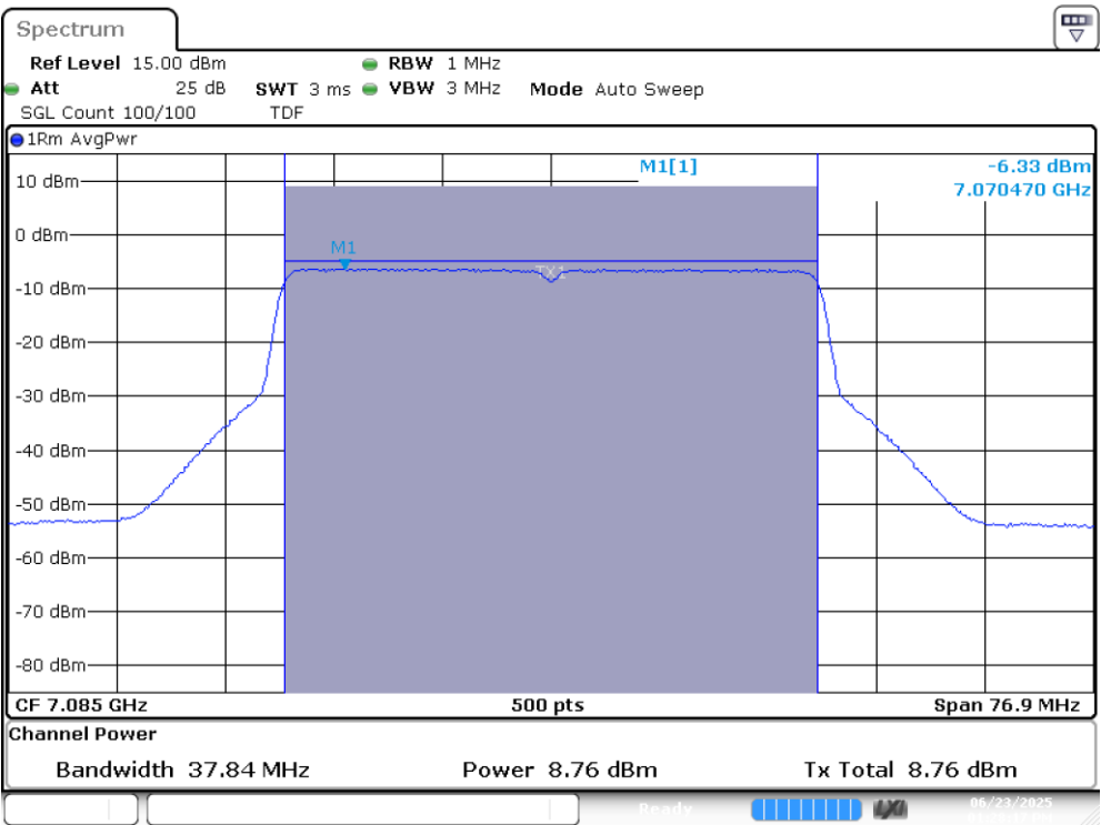
UNII8 SISO B 802.11ax40 ch227 7085MHz
