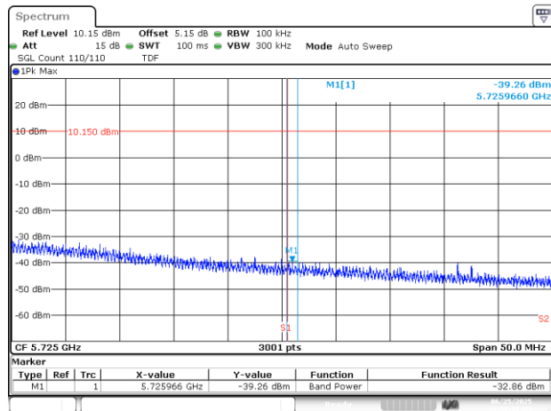
BE-NR-HIGH, MIMO-B, 802.11n40-HT0, Ch134
