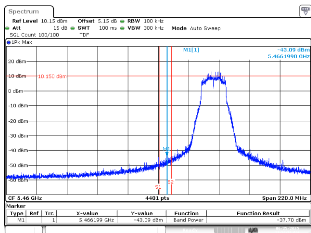
BE-NR-LOW, MIMO-B, 802.11n20-HT0, Ch100
