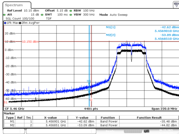
BE-R-LOW, MIMO-B, 802.11n40-HT0, Ch102
