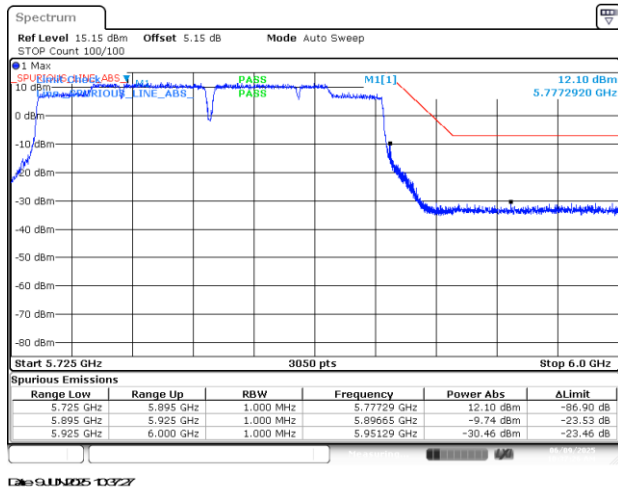
BE-NR-HIGH-PEAK, SISO-A, 802.11ac160-VHT0, Ch163
