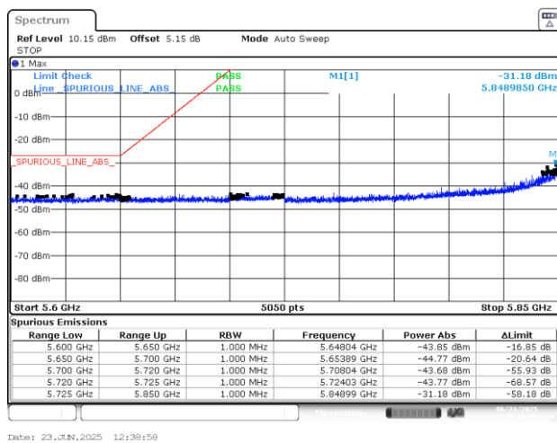
BE-NR-LOW, SISO-A, 802.11n20-HT0, Ch177
