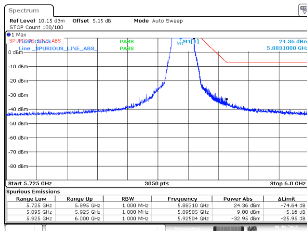
BE-NR-HIGH-PEAK, SISO-A, 802.11ax/be20-HE0, Ch177
