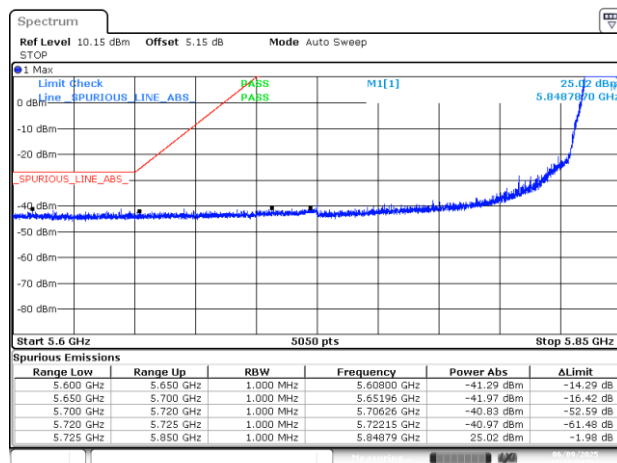
BE-NR-LOW, SISO-B, 802.11ax/be20-MCS0, Ch169
