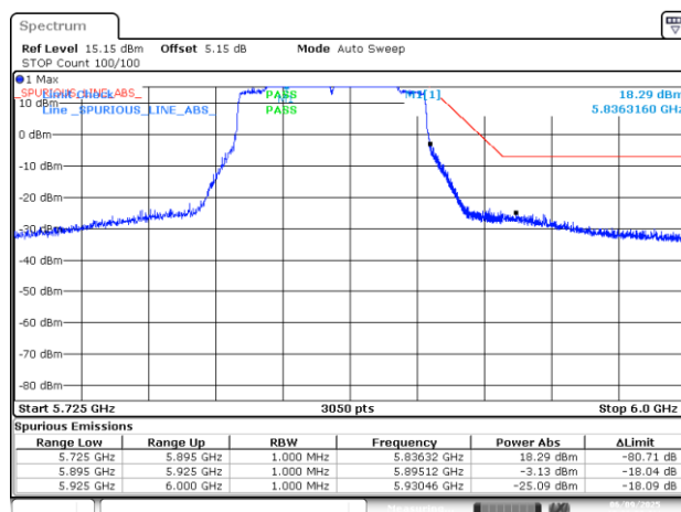
BE-NR-HIGH-PEAK, SISO-A, 802.11ac80-VHT0, Ch171
