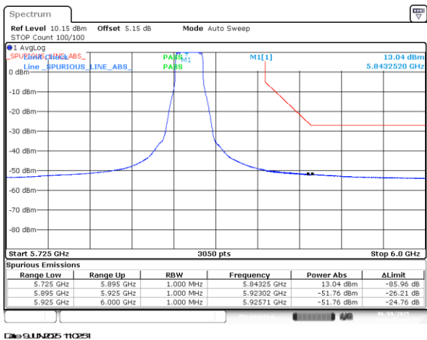
BE-NR-HIGH, SISO-A, 802.11n20-HT0, Ch169
