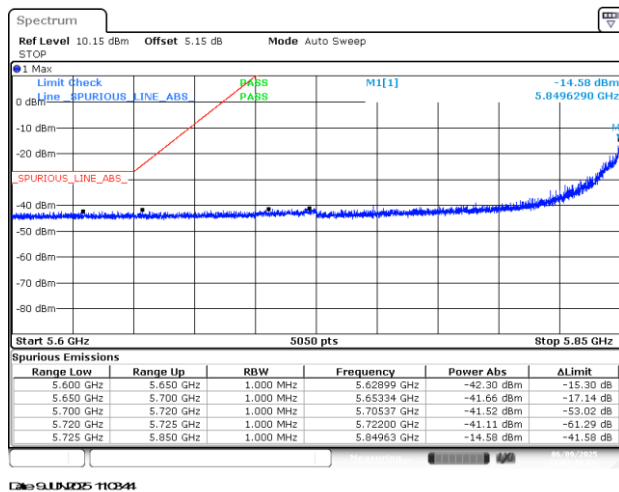
BE-NR-LOW, SISO-A, 802.11n20-HT0, Ch173
