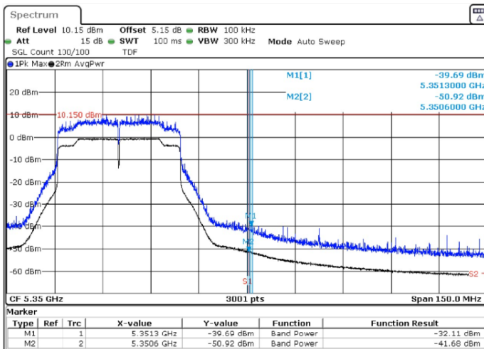
BE-R-HIGH, SISO-B, 802.11ax40-MCS0, Ch62
