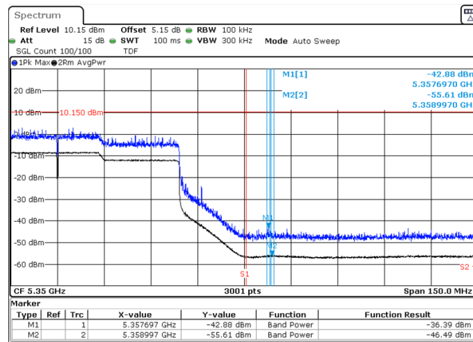
BE-R-HIGH, SISO-A, 802.11ax160-MCS0, Ch50
