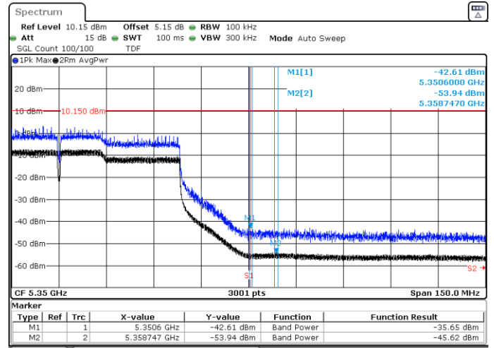
BE-R-HIGH, MIMO-B, 802.11ac160-VHT0, Ch50
