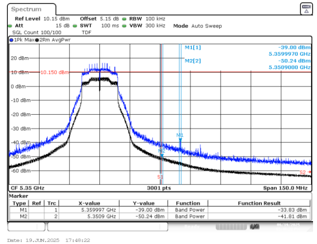
BE-R-HIGH, SISO-A, 802.11n20-HT0, Ch64
