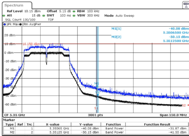
BE-R-HIGH, SISO-B, 802.11n40-HT0, Ch62
