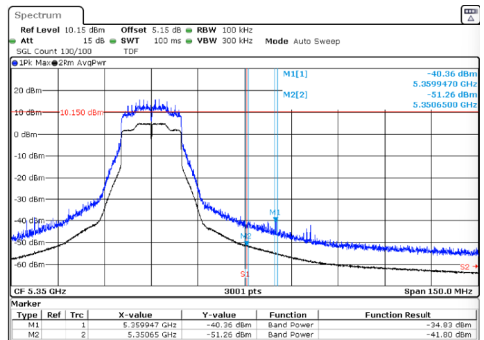
BE-R-HIGH, SISO-B, 802.11ax20-MCS0, Ch64
