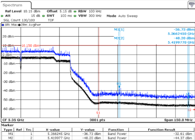
BE-R-HIGH, MIMO-A, 802.11ac80-VHT0, Ch58
