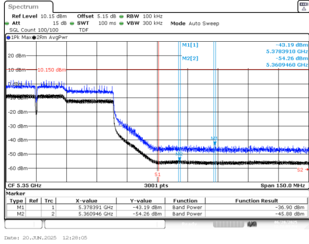
BE-R-HIGH, MIMO-A, 802.11ac160-VHT0, Ch50
