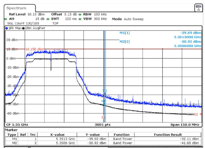
BE-R-HIGH, SISO-A, 802.11ax80-MCS0, Ch58
