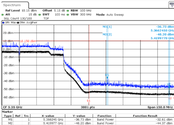
BE-R-HIGH, MIMO-B, 802.11ac80-VHT0, Ch58
