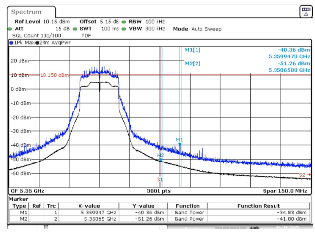
BE-R-HIGH, SISO-A, 802.11ax20-MCS0, Ch64
