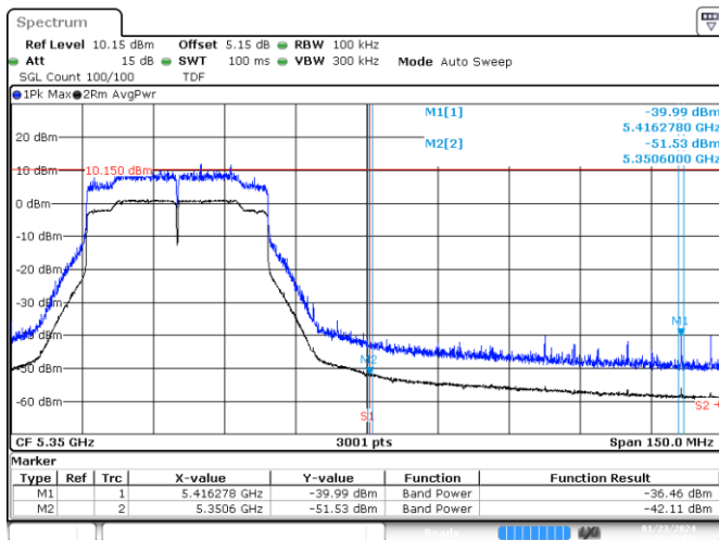
BE-R-HIGH, SISO-A, 802.11ax40-MCS0, Ch62
