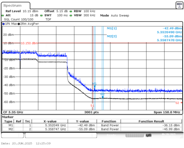
BE-R-HIGH, MIMO-A, 802.11ax/be160-MCS0, Ch50
