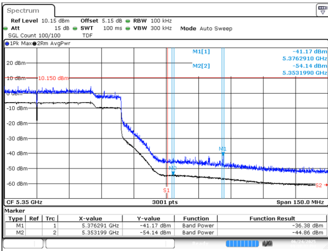
BE-R-HIGH, MIMO-A, 802.11ax/be80-MCS0, Ch58
