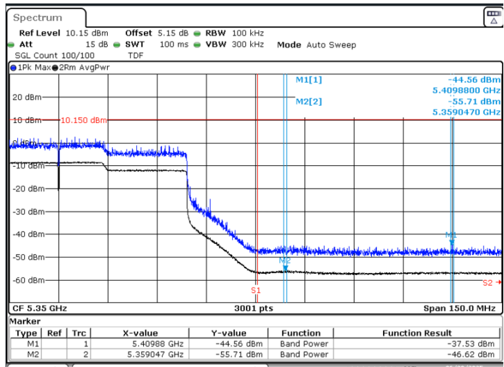
BE-R-HIGH, SISO-B, 802.11ax160-MCS0, Ch50
