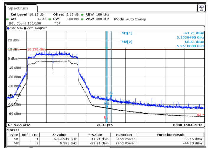
BE-R-HIGH, MIMO-B, 802.11ax/be40-MCS0, Ch62
