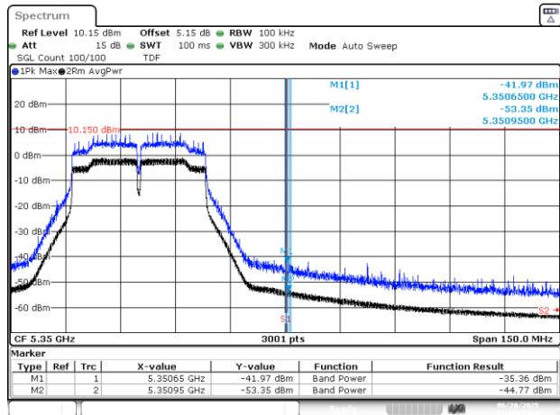
BE-R-HIGH, MIMO-A, 802.11n40-HT0, Ch62
