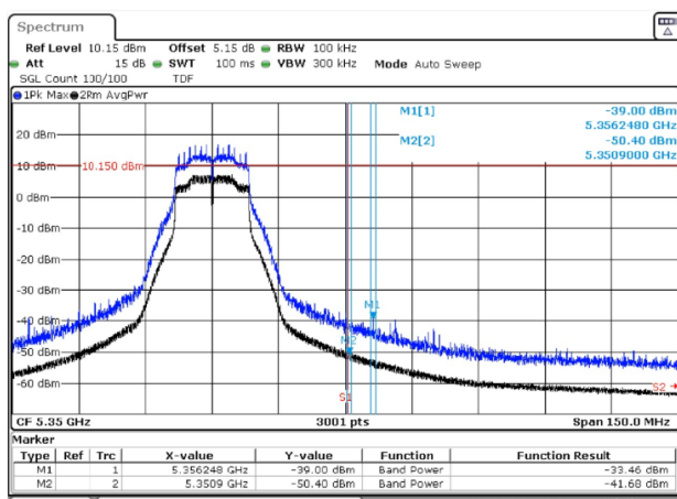
BE-R-HIGH, SISO-B, 802.11a20-6Mbps, Ch64
