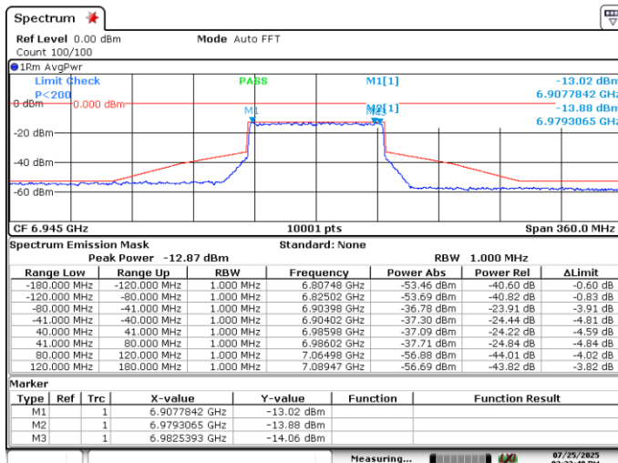
UNII8 MIMO A -802.11ax-80MHz-Ch199-6945MHz-MCS0
