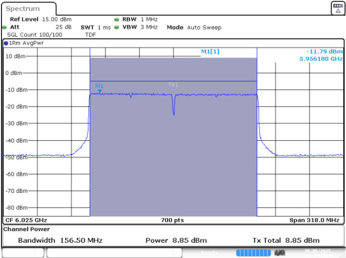
UNII5 SISO B-802.11ax-160MHz-Ch15-6025MHz-MCS0
