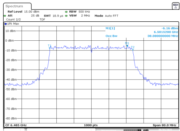
UNII6 SISO A 802.11ax40 ch107 6485MHz 99%
