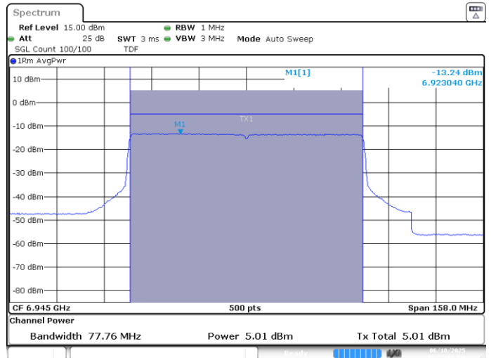
UNII8 MIMO B -802.11ax-80MHz-Ch199-6945MHz-MCS0
