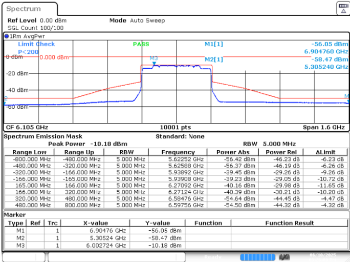
UNII5 MIMO A-802.11be-320MHz-Ch31-6105MHz-MCS0
