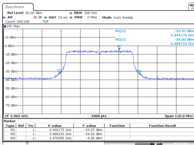
UNII5 MIMO A 802.11ax40 ch3 5965MHz 26dB
