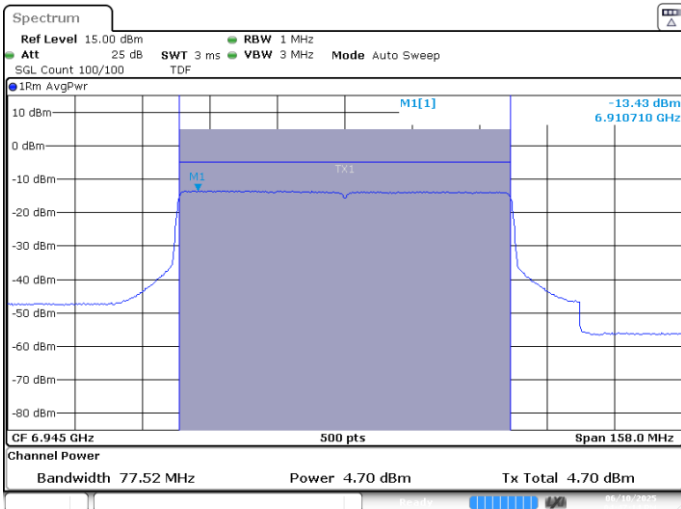
UNII8 MIMO A -802.11ax-80MHz-Ch199-6945MHz-MCS0
