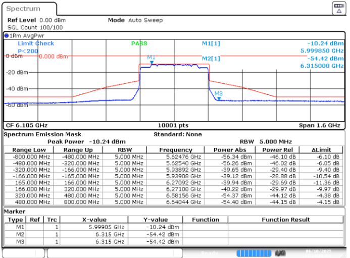
UNII5 MIMO A-802.11be-320MHz-Ch31-6105MHz-MCS0
