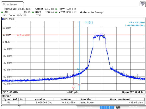
BE-NR-LOW, MIMO-B, 802.11ax/be20-MCS0, Ch100
