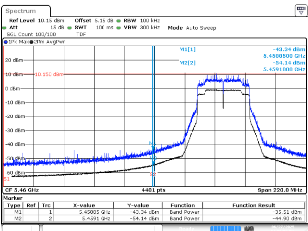
BE-NR-HIGH, MIMO-B, 802.11ax/be40-MCS0, Ch102
