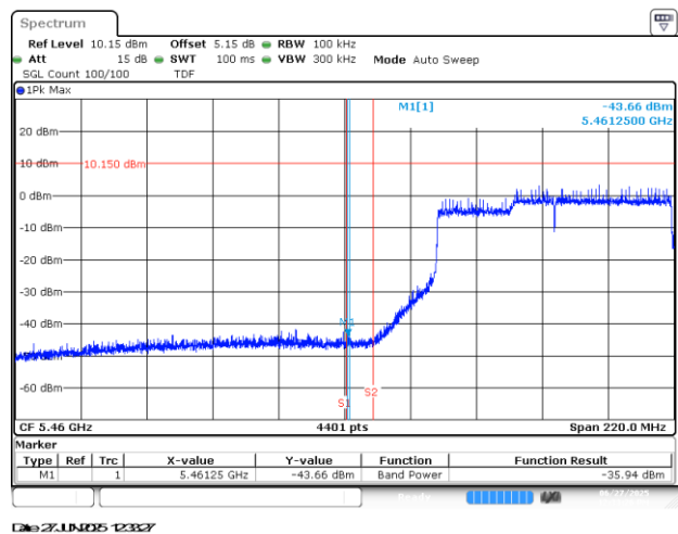
BE-NR-LOW, MIMO-B, 802.11ax/be160-MCS0, Ch114
