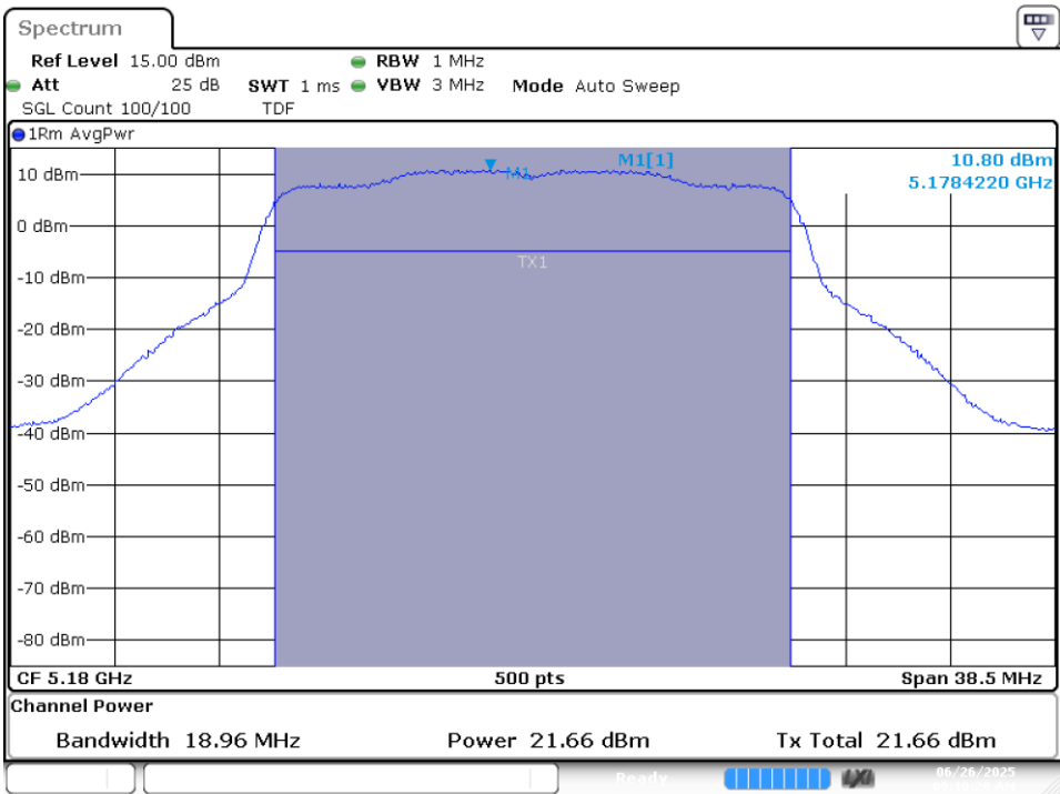
SISO B-802.11ax/be20-Ch36-5180MHz-MCS0
