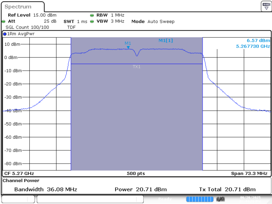
MIMO B-802.11n40-Ch54-5270MHz-HT8
