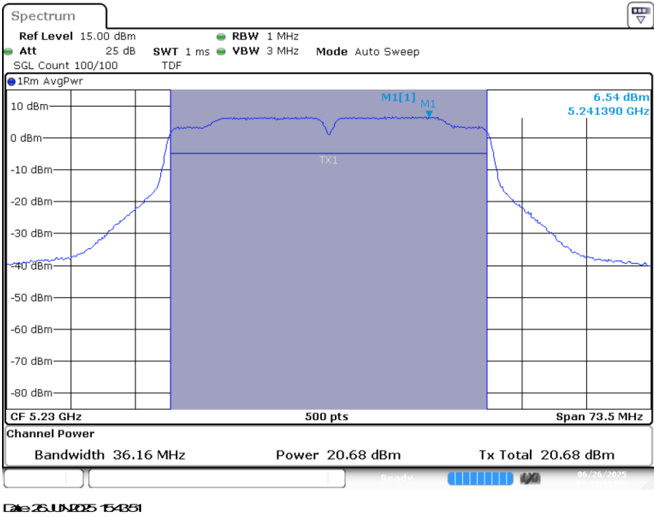
MIMO B-802.11n40-Ch46-5230MHz-HT8
