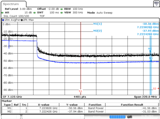
BE-NR-HIGH, SISO-A, 802.11be320-MCS0, Ch191
