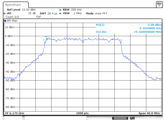
UNII5 MIMO A 802.11ax/be20 ch45 6175MHz 99%
