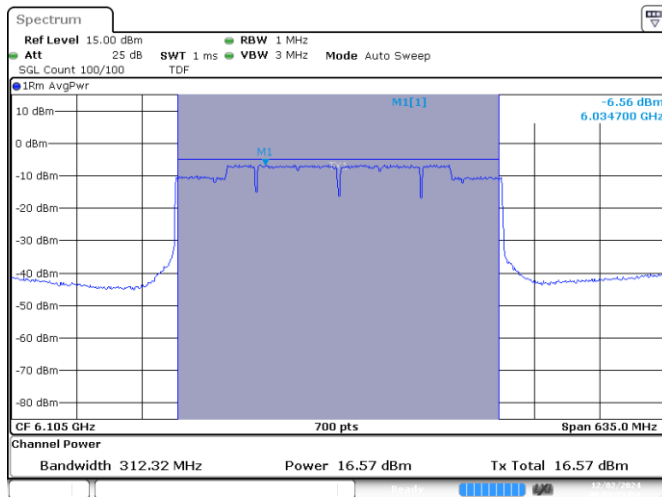
MIMO A-802.11ax/be-320MHz-Ch31-6105MHz-MCS0
