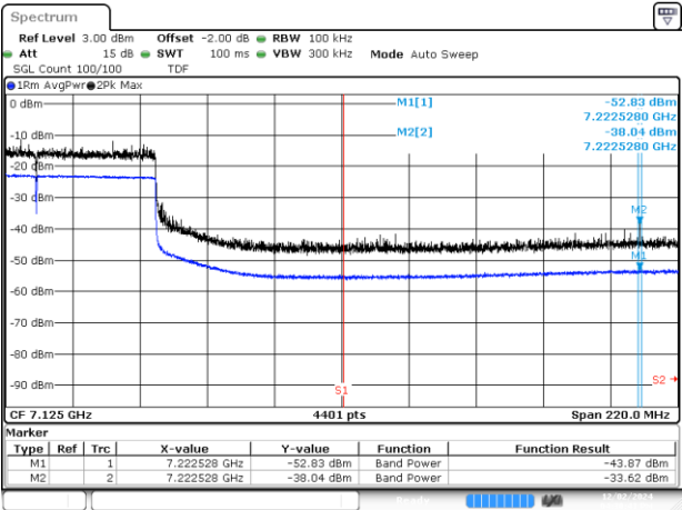
BE-NR-HIGH, MIMO-A, 802.11be320-MCS0, Ch191
