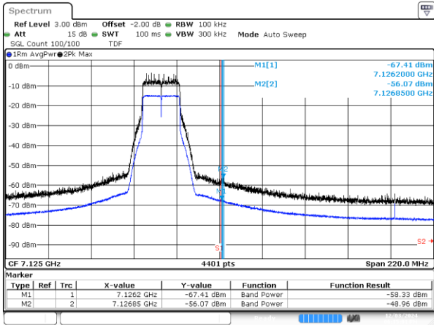
BE-NR-HIGH, MIMO-B, 802.11ax/be20-MCS0, Ch229
