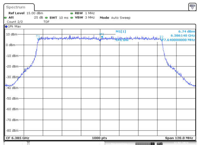
UNII5 MIMO A 802.11ax/be80 ch87 6385MHz 99%
