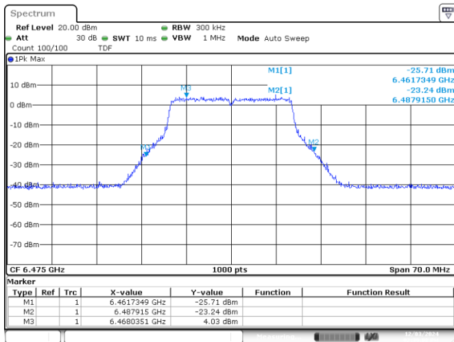
UNII6 SISO B 802.11ax/be20 ch105 6475MHz 26dB
