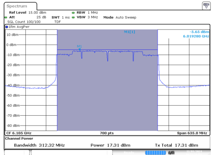
MIMO B-802.11ax/be-320MHz-Ch31-6105MHz-MCS0
