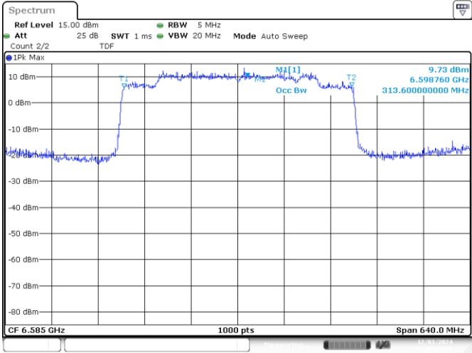
UNII7 SISO B 802.11ax/be320 ch127 6585MHz 99%
