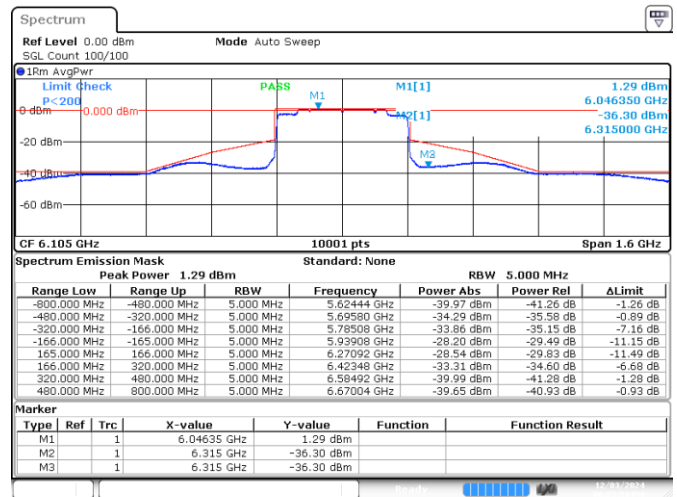
MIMO B-802.11ax/be-320MHz-Ch31-6105MHz-MCS0
