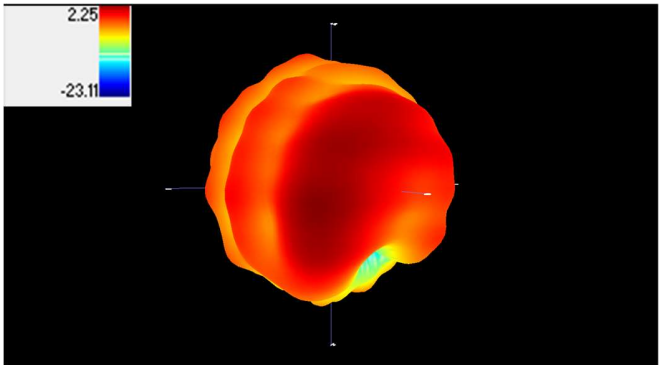
Max Antenna 3D Radiation Pattern 5150-5250 MHz
