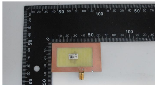
Aux antenna
