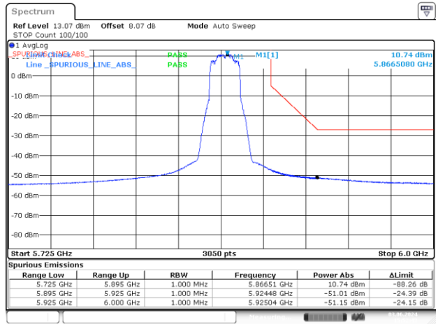
BE-NR-HIGH, MIMO-A, 802.11ax/be20-MCS0, Ch173
