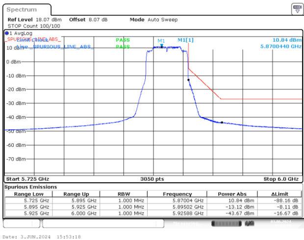
BE-NR-HIGH, MIMO-A, 802.11ax/be40-MCS0, Ch175
