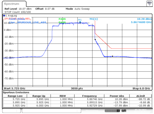
BE-NR-HIGH, MIMO-A, 802.11ax/be80-MCS0, Ch171
