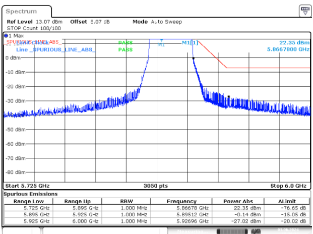
BE-NR-HIGH-PEAK, MIMO-B, 802.11ax/be40-MCS0, Ch175
