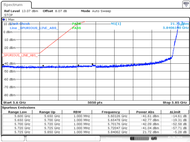
BE-NR-LOW, MIMO-A, 802.11ax/be20-MCS0, Ch169
