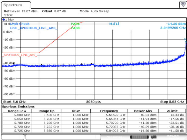
BE-NR-LOW, MIMO-A, 802.11ax/be20-MCS0, Ch173
