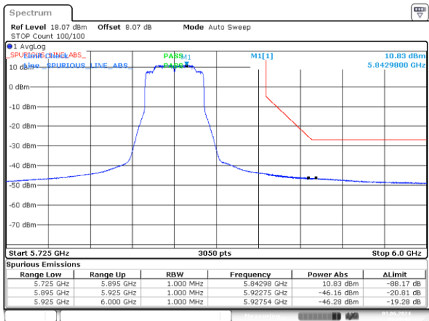
BE-NR-HIGH, MIMO-B, 802.11ax/be40-MCS0, Ch167
