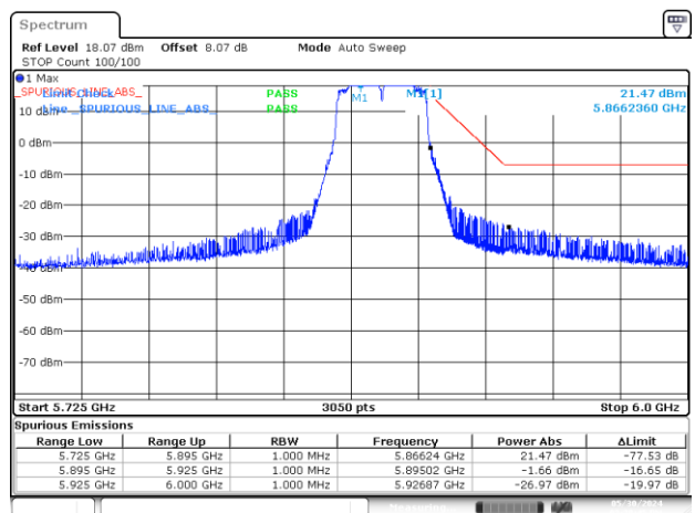
BE-NR-HIGH-PEAK, MIMO-B, 802.11n-HT8, Ch175
