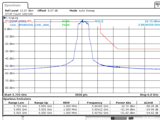
BE-NR-HIGH, MIMO-B, 802.11ax/be20-MCS0, Ch173
