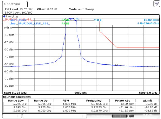
BE-NR-HIGH, MIMO-A, 802.11ax/be20-MCS0, Ch169
