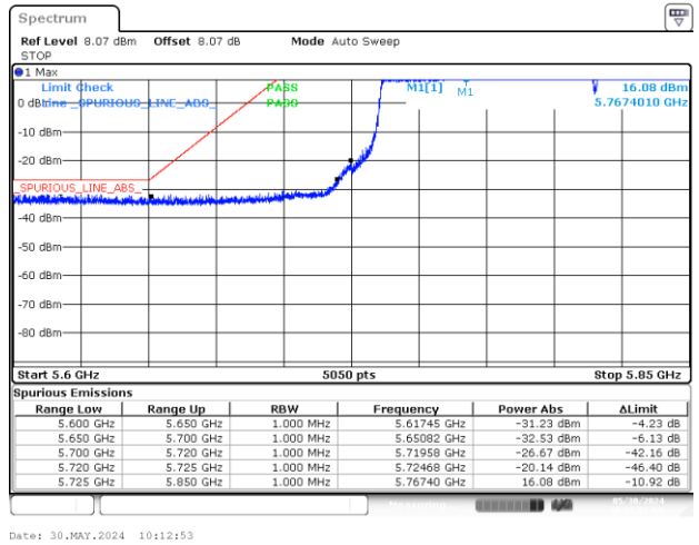
BE-NR-LOW, MIMO-A, 802.11ax/be160-MCS0, Ch163
