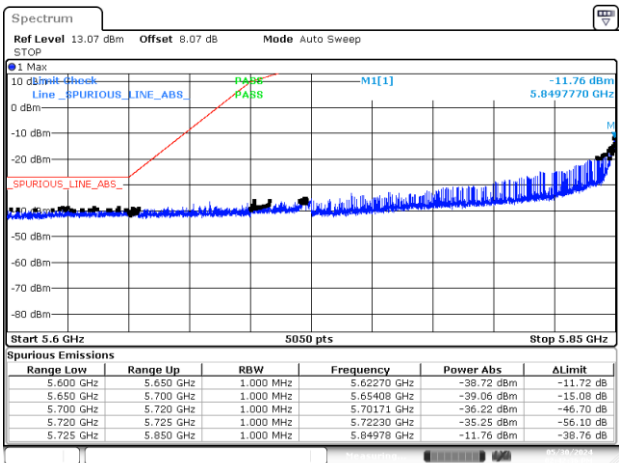
BE-NR-LOW, MIMO-B, 802.11ax/be40-MCS0, Ch175
