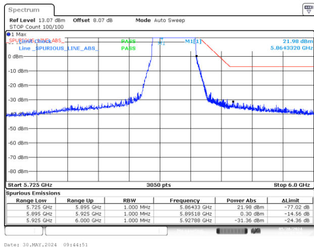
BE-NR-HIGH-PEAK, MIMO-A, 802.11ax/be40-MCS0, Ch175
