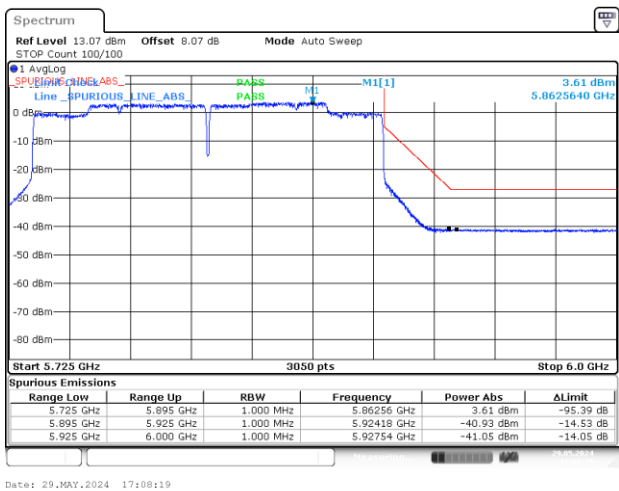
BE-NR-HIGH, MIMO-A, 802.11ax/be160-MCS0, Ch163
