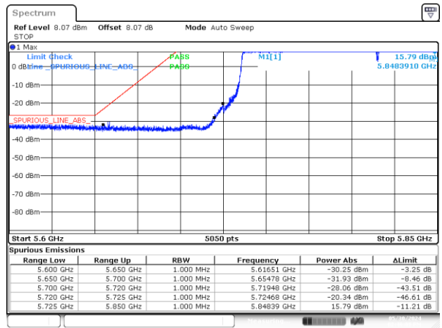
BE-NR-LOW, MIMO-B, 802.11ax/be160-MCS0, Ch163
