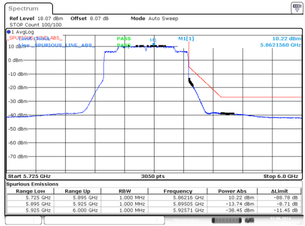
BE-NR-HIGH, MIMO-B, 802.11ax/be80-MCS0, Ch171
