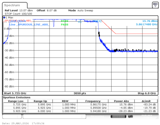
BE-NR-HIGH-PEAK, MIMO-A, 802.11ax/be160-MCS0, Ch163
