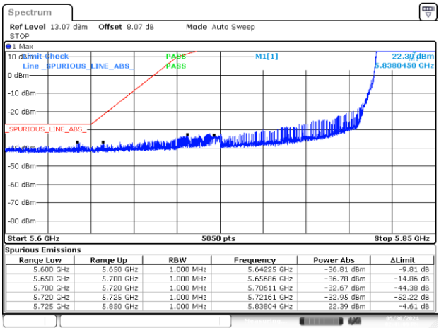
BE-NR-LOW, MIMO-B, 802.11ax/be40-MCS0, Ch167
