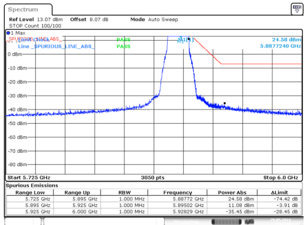
BE-NR-HIGH-PEAK, MIMO-A, 802.11ax/be20-MCS0, Ch177
