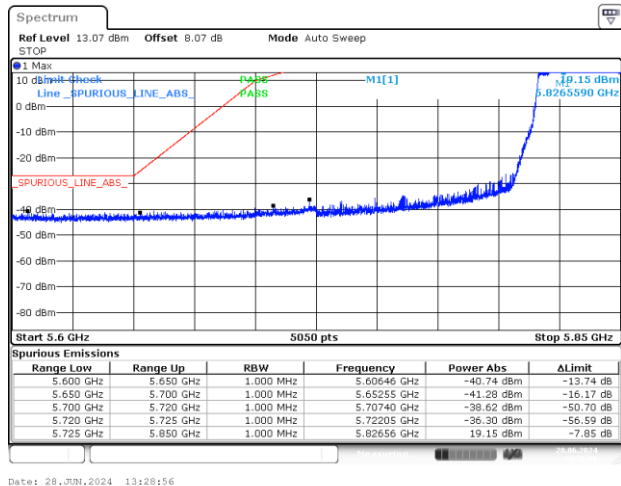
BE-NR-LOW, MIMO-A, 802.11ax/be40-MCS0, Ch167
