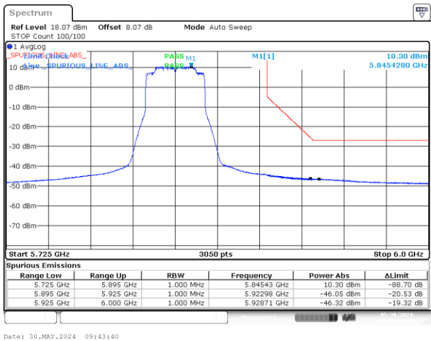
BE-NR-HIGH, MIMO-A, 802.11ax/be40-MCS0, Ch167
