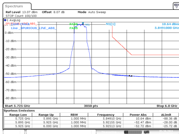
BE-NR-HIGH, MIMO-B, 802.11ax/be20-MCS0, Ch169
