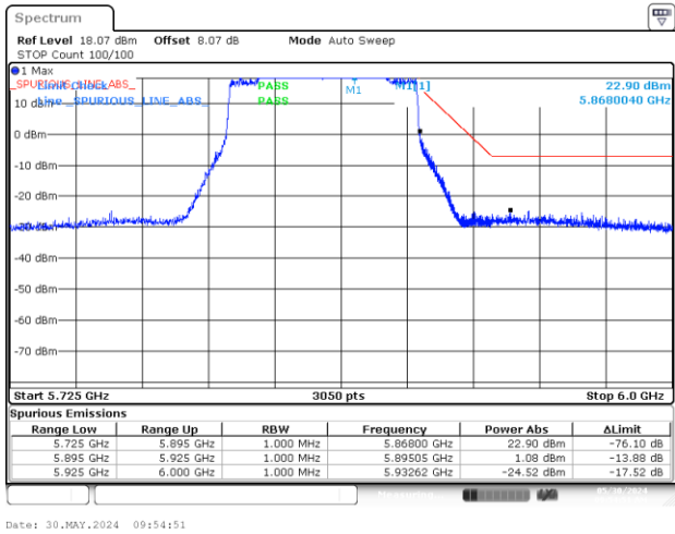
BE-NR-HIGH-PEAK, MIMO-A, 802.11ax/be80-MCS0, Ch171
