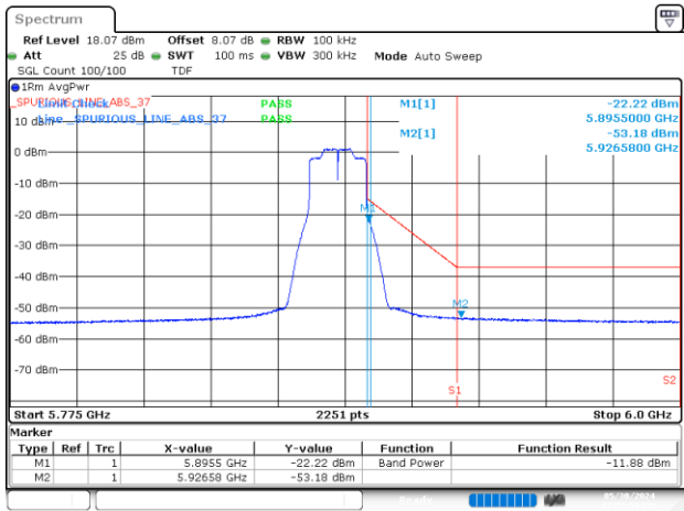
BE-NR-HIGH, MIMO-B, 802.11ax/be20-MCS0, Ch177
