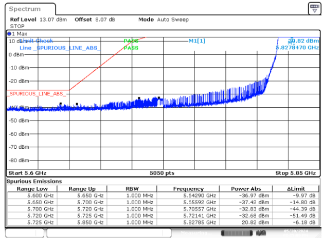
BE-NR-LOW, MIMO-B, 802.11n40-HT8, Ch167
