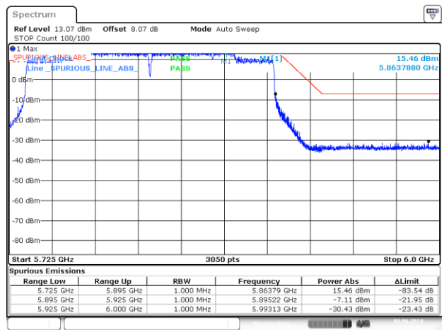
BE-NR-HIGH-PEAK, MIMO-B, 802.11ax/be160-MCS0, Ch163
