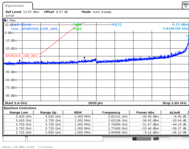
BE-NR-LOW, MIMO-A, 802.11ax/be40-MCS0, Ch175
