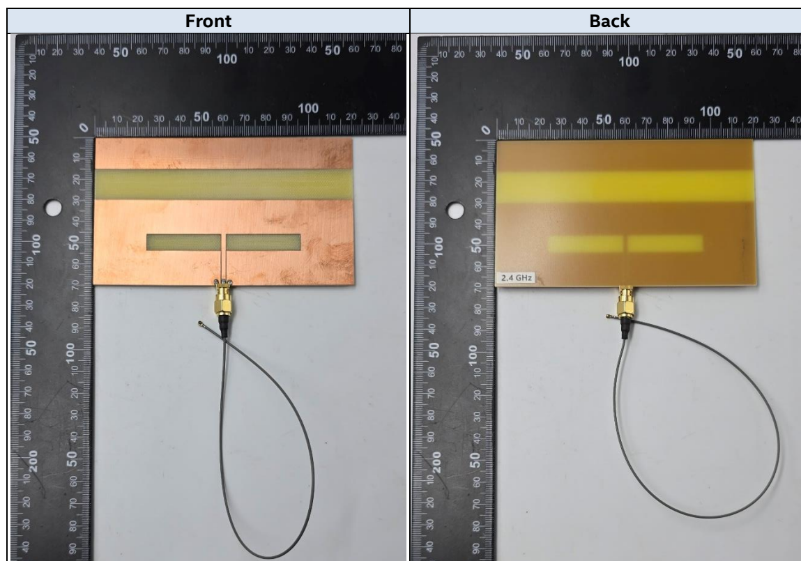
Antenna cable length = 28 cm.
