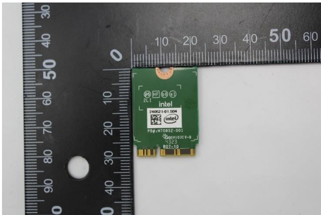
Adaptor Back
