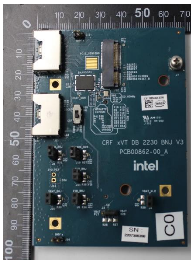
Extender board
