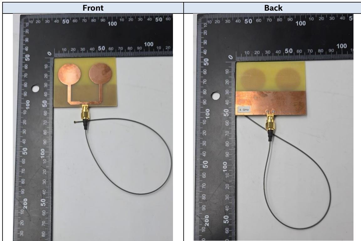
Antenna cable length = 28 cm.
