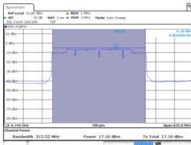
SISO B-802.11ax/be-320MHz-Ch159-MCS0
