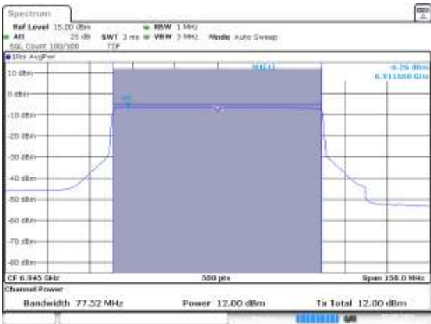
SISO A-802.11ax/be-80MHz-Ch199-MCS0
