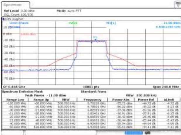
MIMO B-802.11ax/be-40MHz-Ch179-MCS0
