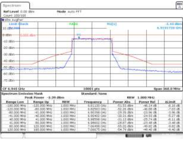
SISO A-802.11ax/be-80MHz-Ch199-MCS0
