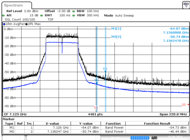
BE-NR-HIGH, MIMO-B, 802.11ax/be40-MCS0, Ch227
