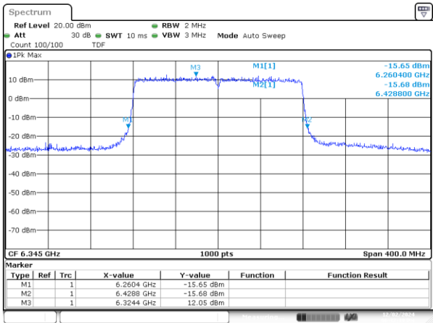
UNII5 SISO B 802.11ax/be160 ch79 6345MHz 26dB
