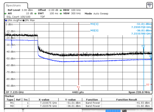
BE-NR-HIGH, MIMO-A, 802.11be320-MCS0, Ch191
