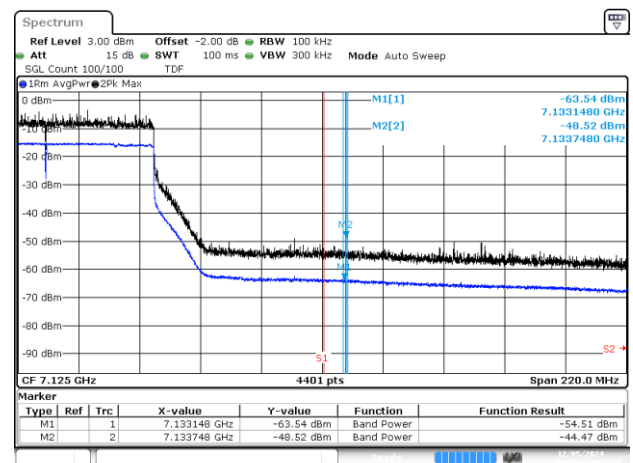
BE-NR-HIGH, MIMO-A, 802.11ax/be80-MCS0, Ch215
