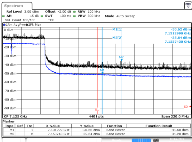
BE-NR-HIGH, MIMO-B, 802.11ax/be160-MCS0, Ch207
