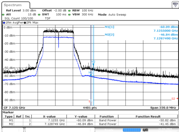
BE-NR-HIGH, SISO-A, 802.11ax/be40-MCS0, Ch227
