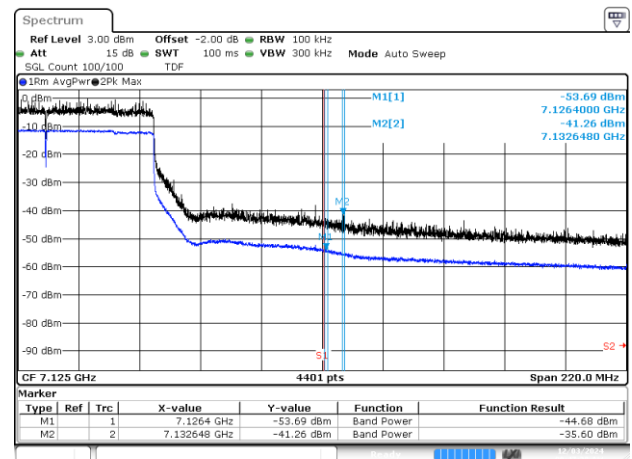
BE-NR-HIGH, SISO-B, 802.11ax/be80-MCS0, Ch215
