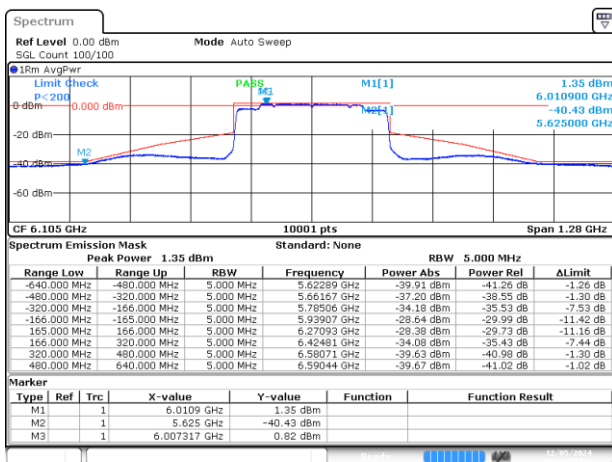
MIMO A-802.11ax/be-320MHz-Ch31-6105MHz-MCS0
