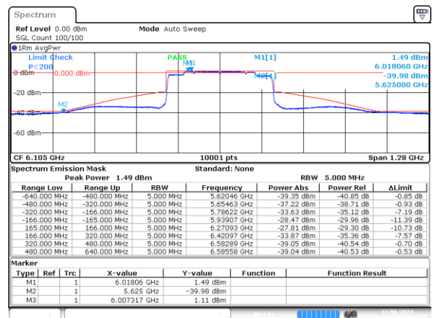
MIMO B-802.11ax/be-320MHz-Ch31-6105MHz-MCS0
