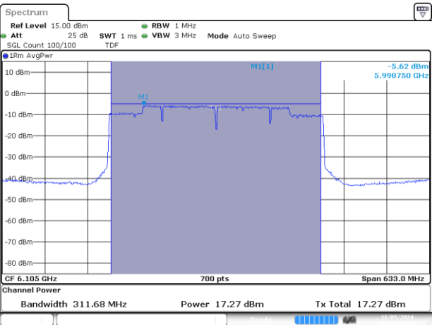
MIMO A-802.11ax/be-320MHz-Ch31-6105MHz-MCS0
