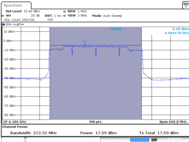
MIMO B-802.11ax/be-320MHz-Ch31-6105MHz-MCS0
