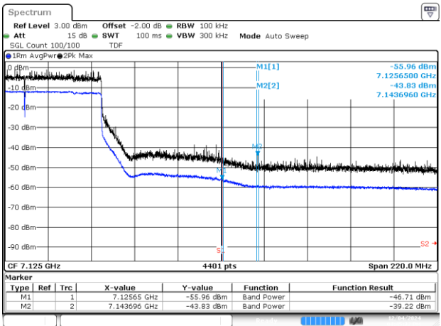
BE-NR-HIGH, SISO-A, 802.11ax/be80-MCS0, Ch215
