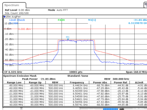
SISO A-802.11ax/be-40MHz-Ch115-6525MHz-MCS0
