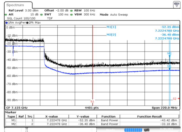
BE-NR-HIGH, SISO-B, 802.11be320-MCS0, Ch191
