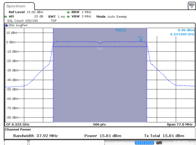
SISO A-802.11ax/be-40MHz-Ch115-6525MHz-MCS0
