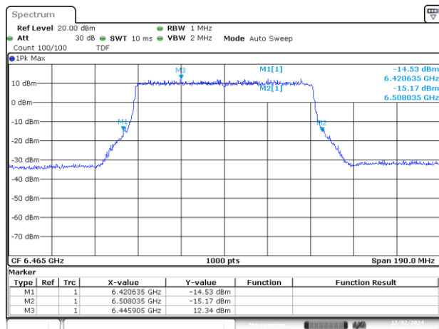
UNII6 SISO B 802.11ax/be80 ch103 6465MHz 26dB
