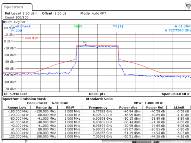
MIMO A-802.11ax/be-80MHz-Ch199-6945MHz-MCS0
