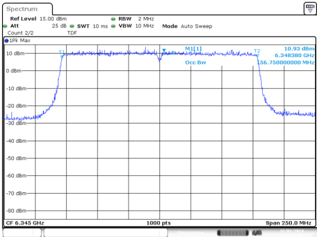
UNII5 SISO B 802.11ax/be160 ch79 6345MHz 99%
