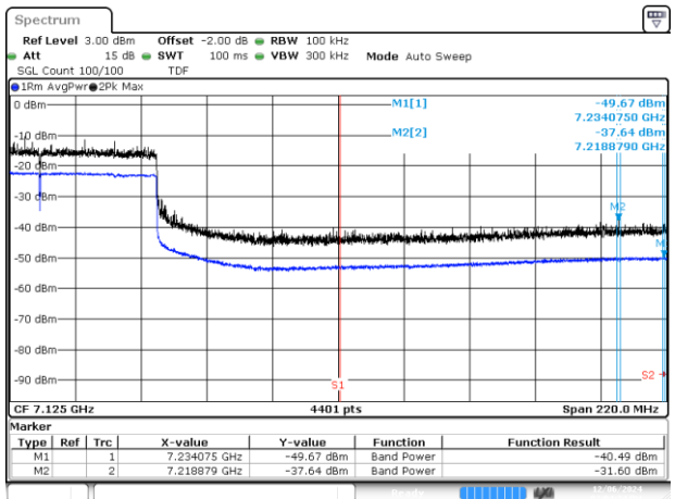
BE-NR-HIGH, MIMO-B, 802.11be320-MCS0, Ch191
