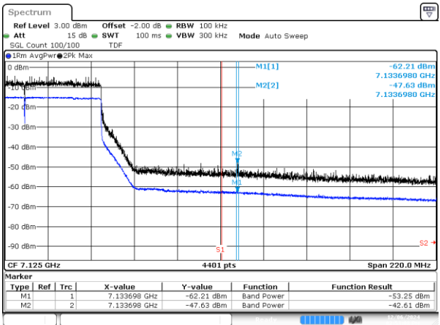
BE-NR-HIGH, MIMO-B, 802.11ax/be80-MCS0, Ch215
