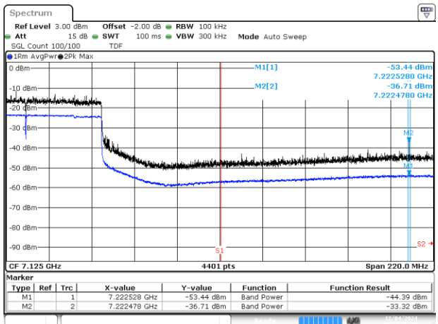
BE-NR-HIGH, SISO-A, 802.11be320-MCS0, Ch191
