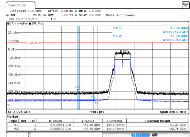
BE-NR-LOW, SISO-B, 802.11ax/be20-MCS0, Ch1
