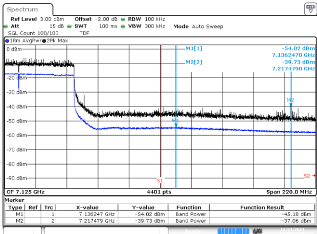
BE-NR-HIGH, SISO-A, 802.11ax/be160-MCS0, Ch207
