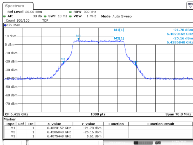
UNII5 SISO A 802.11ax/be20 ch93 6415MHz 26dB
