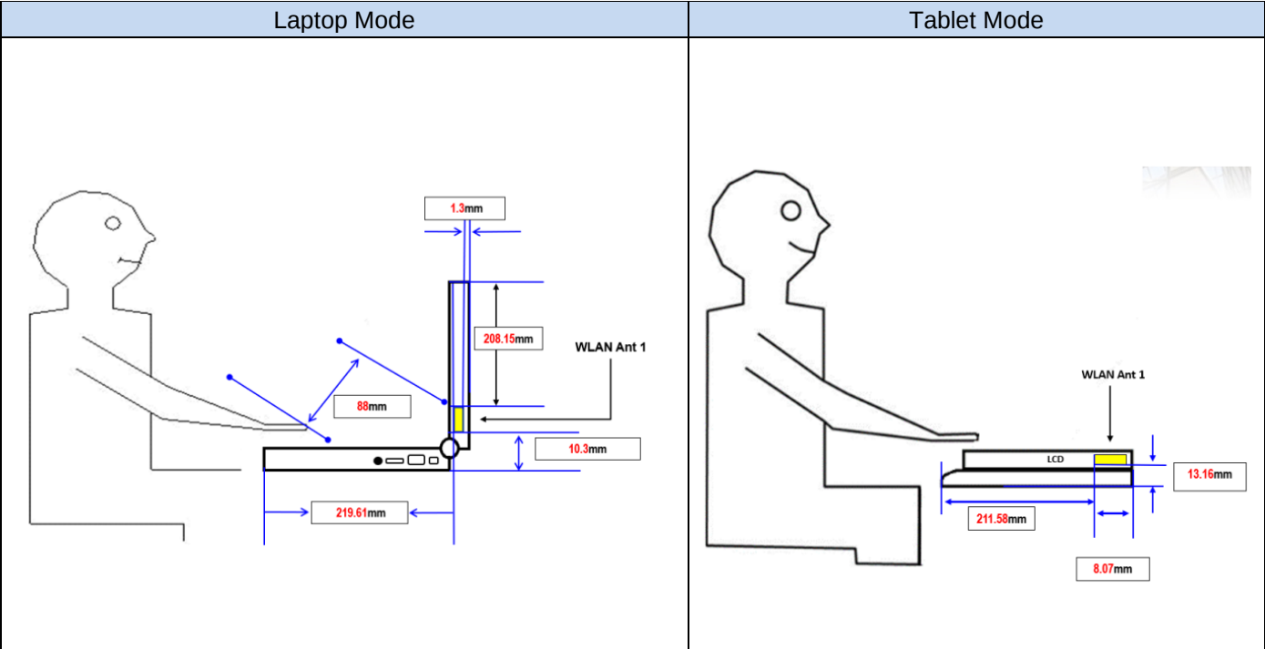
Antenna positions
