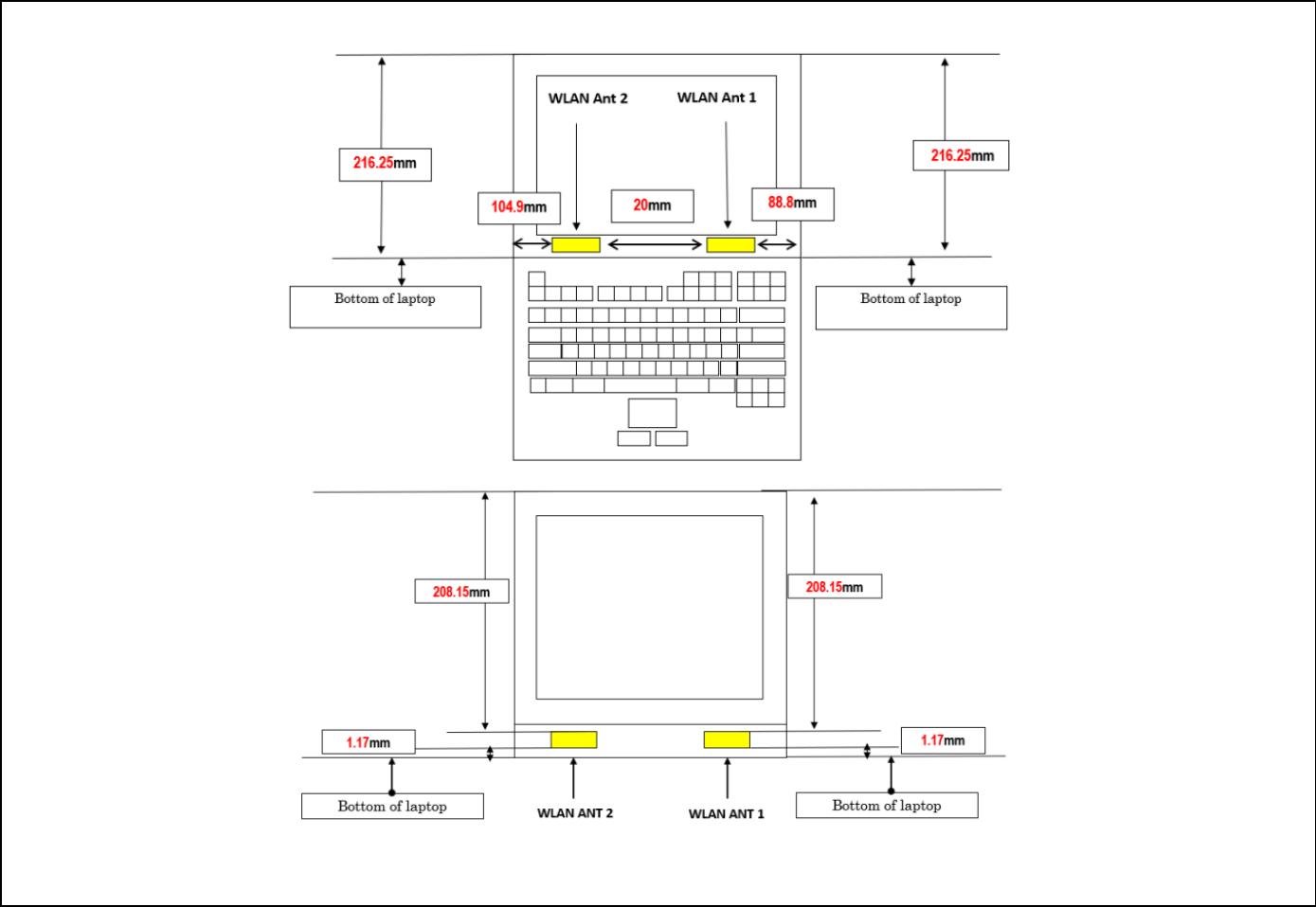
Antenna positions
