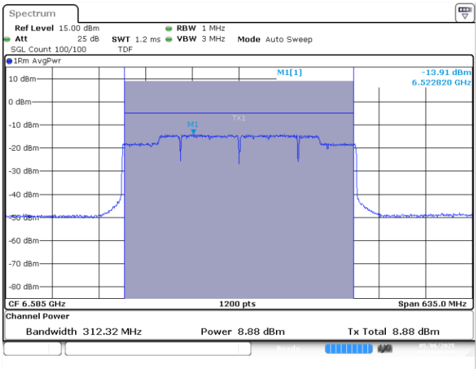
SISO A-802.11ax/be-320MHz-Ch127-6585MHz-MCS0
