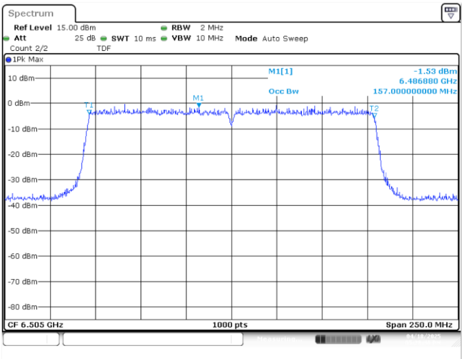
UNII6 MIMO A 802.11ax/be160 ch111 6505MHz 99%
