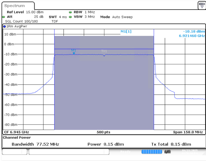
SISO A-802.11ax/be-80MHz-Ch199-6945MHz-MCS0
