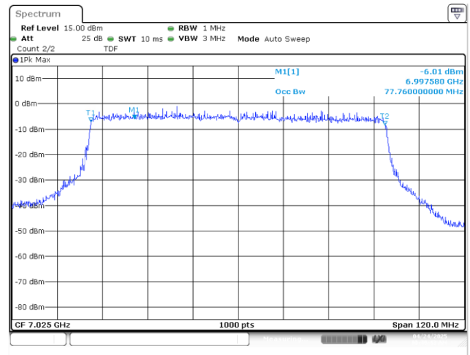
UNII7 MIMO A 802.11ax/be80 ch215 7025MHz 99%
