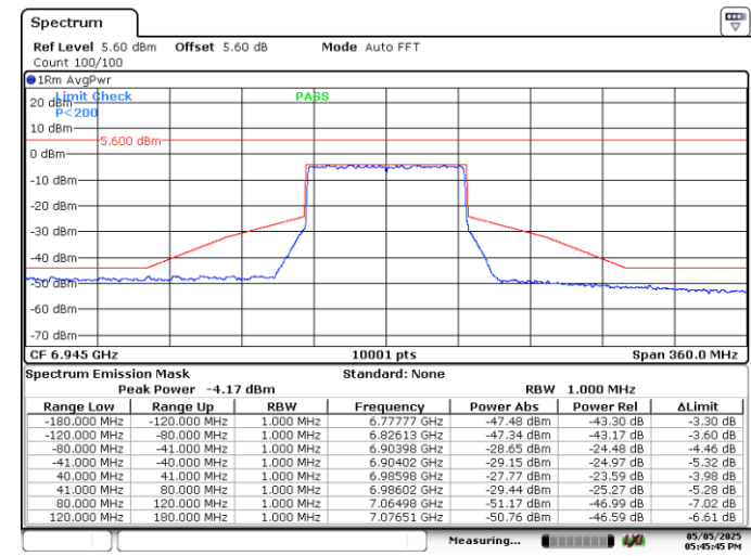
SISO A-802.11ax/be-80MHz-Ch199-6945MHz-MCS0
