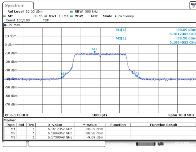
UNII5 MIMO A 802.11ax/be20 ch45 6175MHz 26dB
