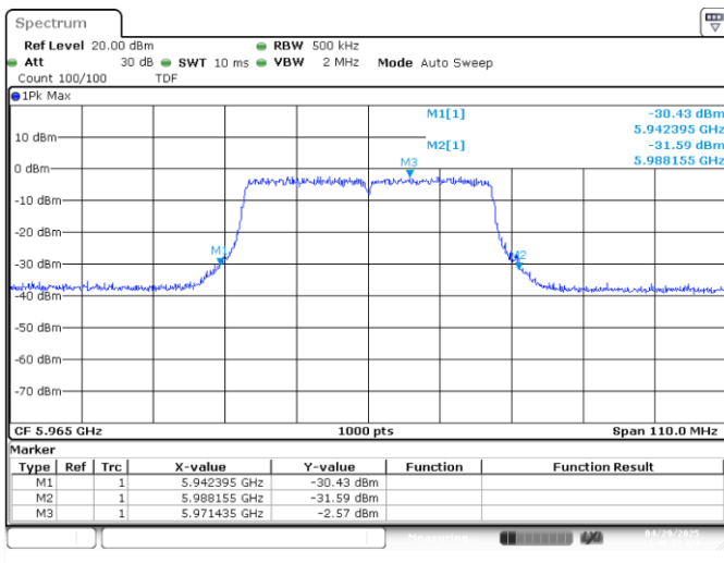
UNII5 SISO B 802.11ax/be40 ch3 5965MHz 26dB
