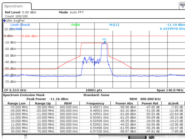
SISO-A, 802.11ax/be20-MCS0, Ch113-4m-37
