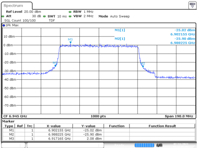
UNI18 MIMO B 802.11ax/be80 ch199 6945MHz 26dB
