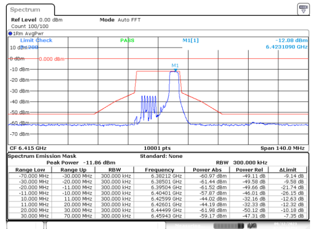
SISO-A, 802.11ax/be20-MCS0, Ch93-4m-37
