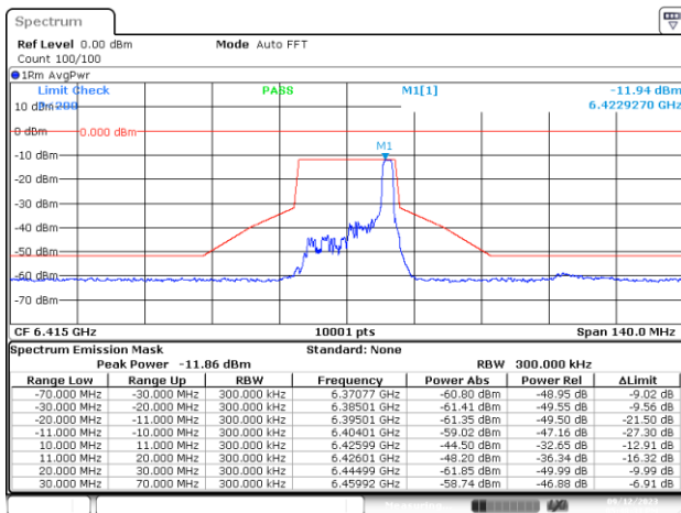
SISO-A, 802.11ax/be20-MCS0, Ch93-2m-0
