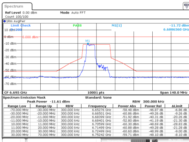
SISO-A, 802.11ax/be20-MCS0, Ch149-6m-70
