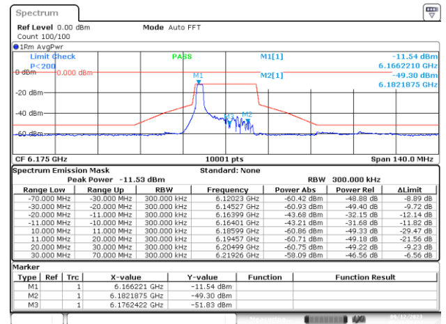
SISO-A, 802.11ax/be20-MCS0, Ch45-2m-0
