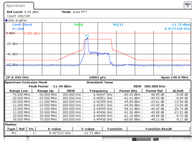
SISO-A, 802.11ax/be20-MCS0, Ch97-2m-0
