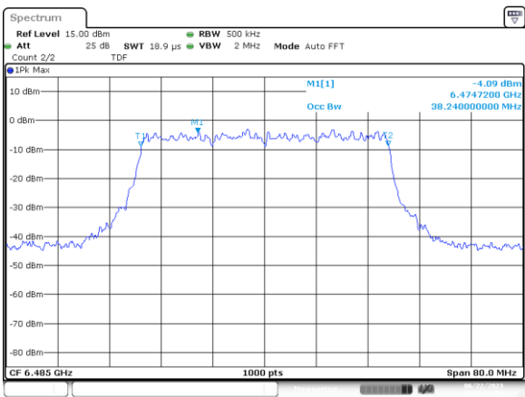
UNII6 MIMO A 802.11ax/be40 ch107 6485MHz 99%
