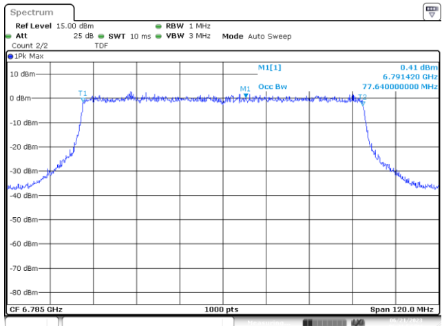
UNI17 MIMO B 802.11ax/be80 ch167 6785MHz 99%
