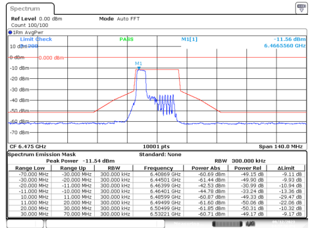
SISO-A, 802.11ax/be20-MCS0, Ch105-4m-37
