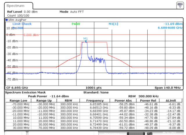
SISO-A, 802.11ax/be20-MCS0, Ch149-4m-37
