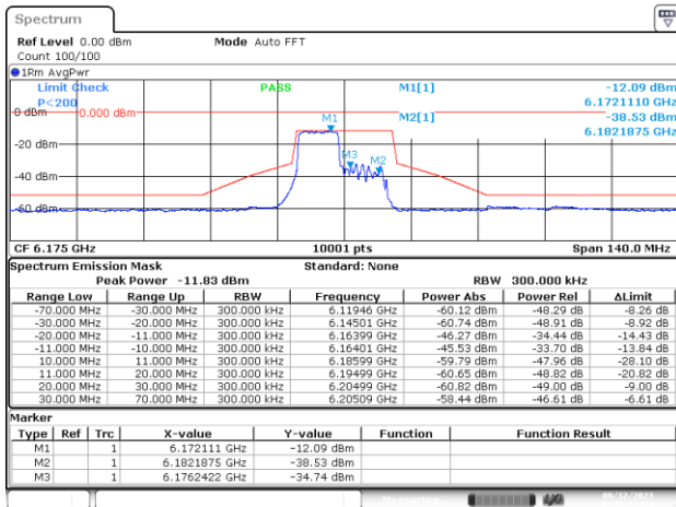
SISO-A, 802.11ax/be20-MCS0, Ch45-8m-53
