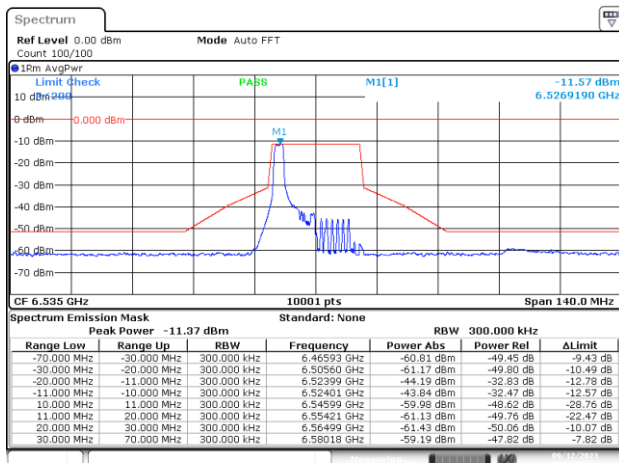
SISO-A, 802.11ax/be20-MCS0, Ch117-2m-0
