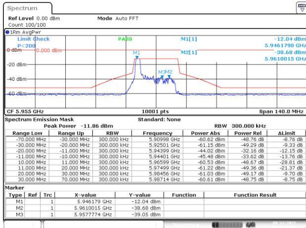
SISO-A, 802.11ax/be20-MCS0, Ch1-2m-0
