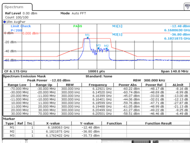
SISO-A, 802.11ax/be20-MCS0, Ch45-4m-37
