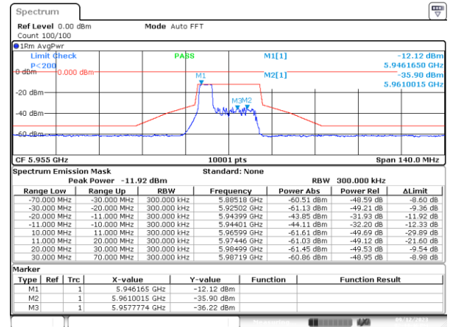
SISO-A, 802.11ax/be20-MCS0, Ch1-4m-37
