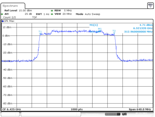
UNI15 MIMO A 802.11be320 ch95 6425MHz 99%
