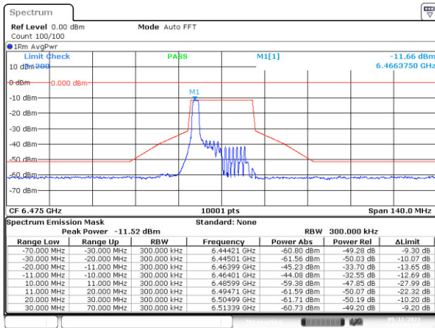
SISO-A, 802.11ax/be20-MCS0, Ch105-2m-0
