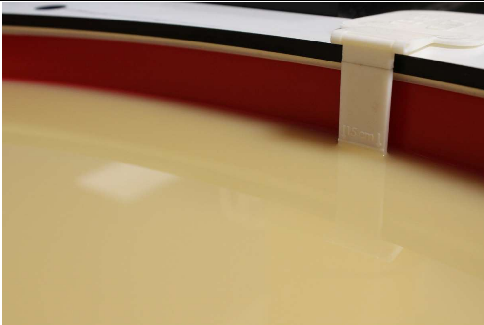
ELI phantom Head liquid SAR SPEAG HBBL600-6000V6 Batch - 210331-1
