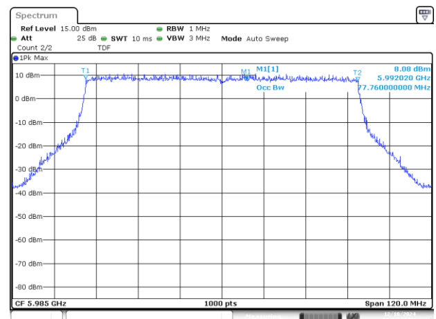
UNII5 SISO A 802.11ax/be80 ch7 5985MHz 99%
