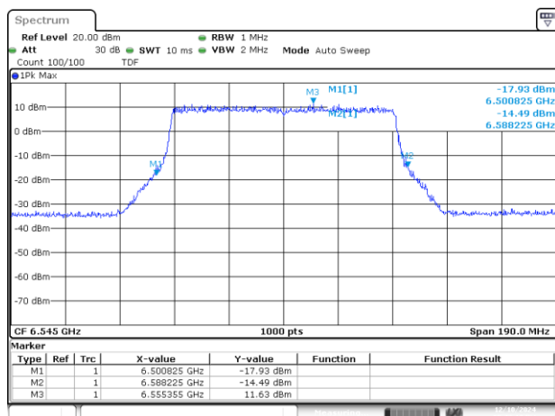
UNII6 SISO A 802.11ax/be80 ch119 6545MHz 26dB
