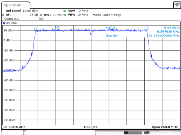
UNII5 SISO A 802.11ax/be160 ch79 6345MHz 99%
