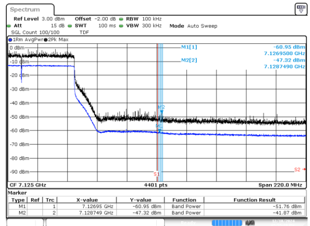
BE-NR-HIGH, SISO-A, 802.11ax/be80-MCS0, Ch215
