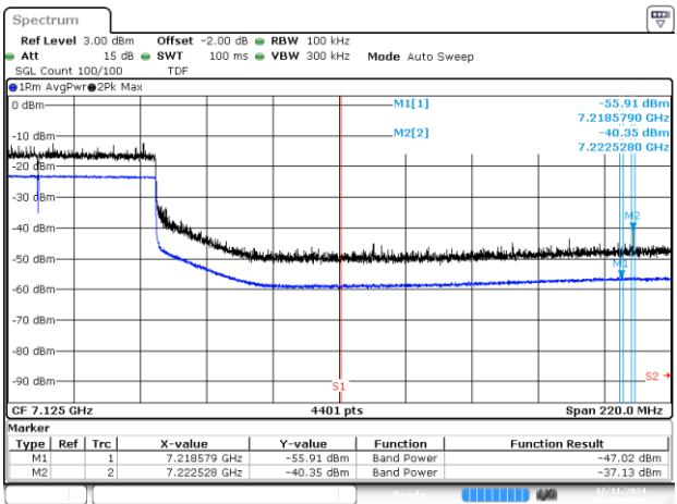
BE-NR-HIGH, MIMO-B, 802.11be320-MCS0, Ch191
