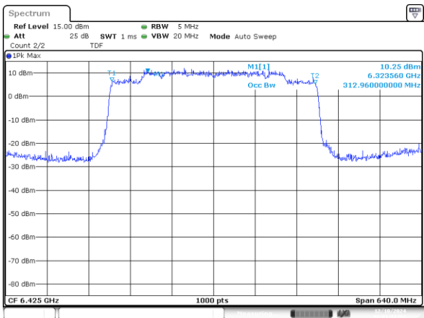
UNII5 SISO A 802.11ax/be320 ch95 6425MHz 99%
