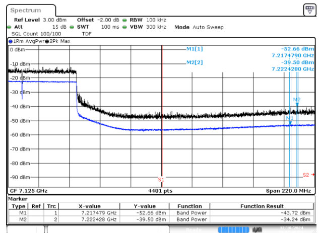
BE-NR-HIGH, SISO-A, 802.11be320-MCS0, Ch191
