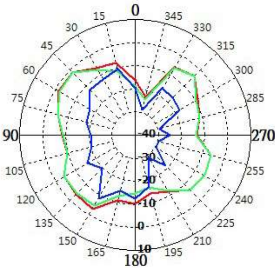
Max Antenna 2D Radiation Pattern 6875-7125 MHz
