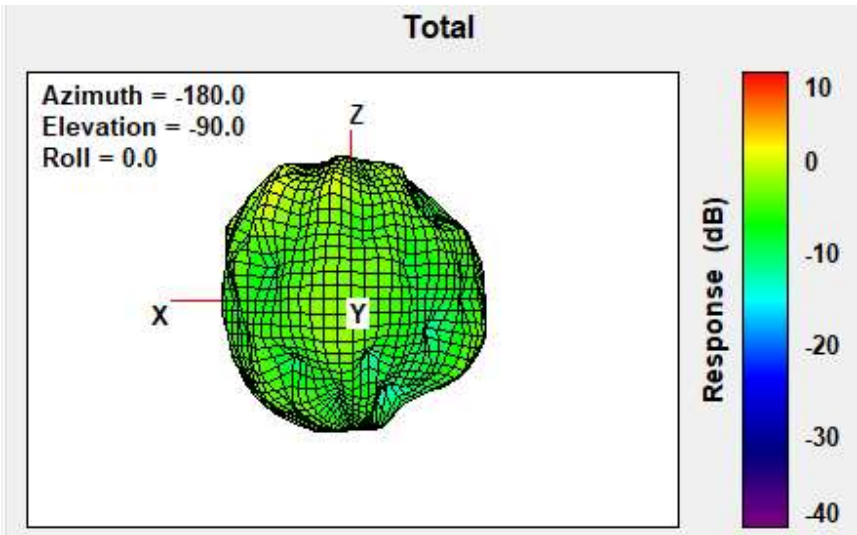
Max Antenna 3D Radiation Pattern 5150-5250 MHz
