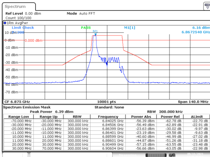
SISO-B, 802.11ax/be20-MCS0, Ch185-2m-0
