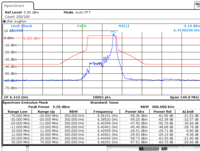
MIMO-B, 802.11ax/be20-MCS0, Ch93-2m-0
