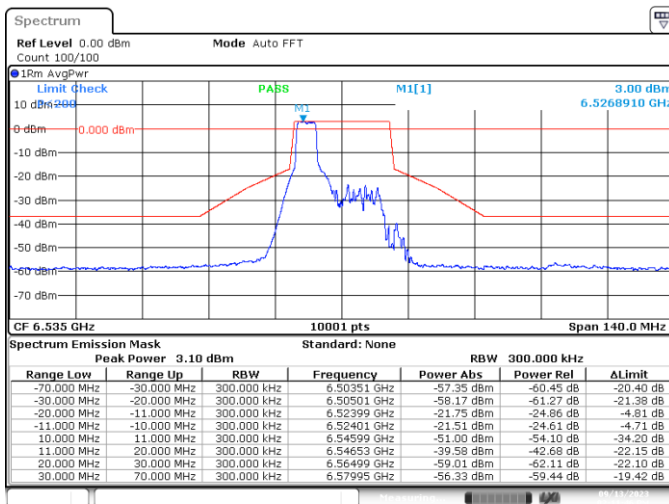
MIMO-B, 802.11ax/be20-MCS0, Ch117-4m-37
