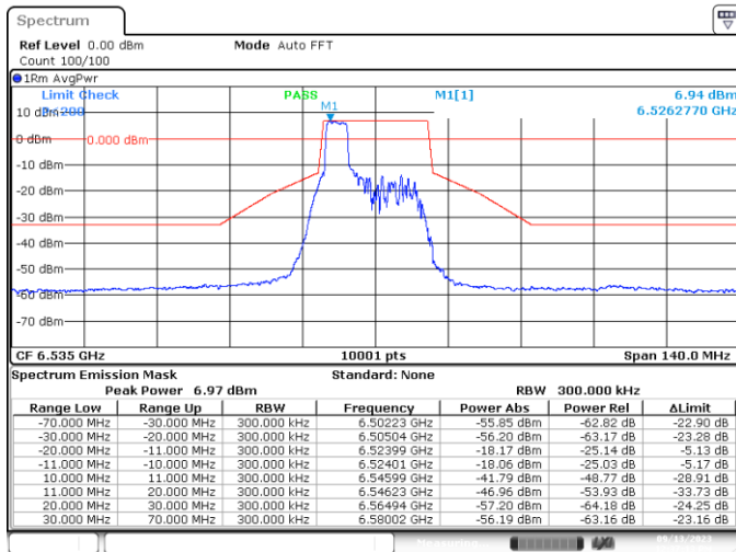
SISO-B, 802.11ax/be20-MCS0, Ch117-4m-37
