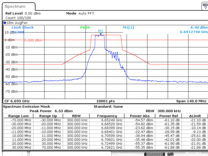
SISO-B, 802.11ax/be20-MCS0, Ch149-6m-70
