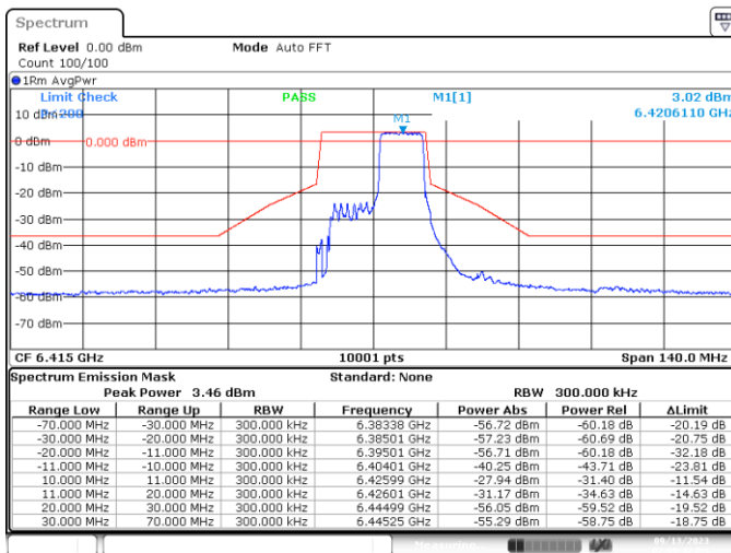
MIMO-B, 802.11ax/be20-MCS0, Ch93-8m-53
