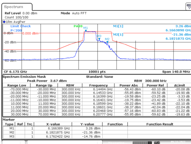
MIMO-B, 802.11ax/be20-MCS0, Ch45-8m-53
