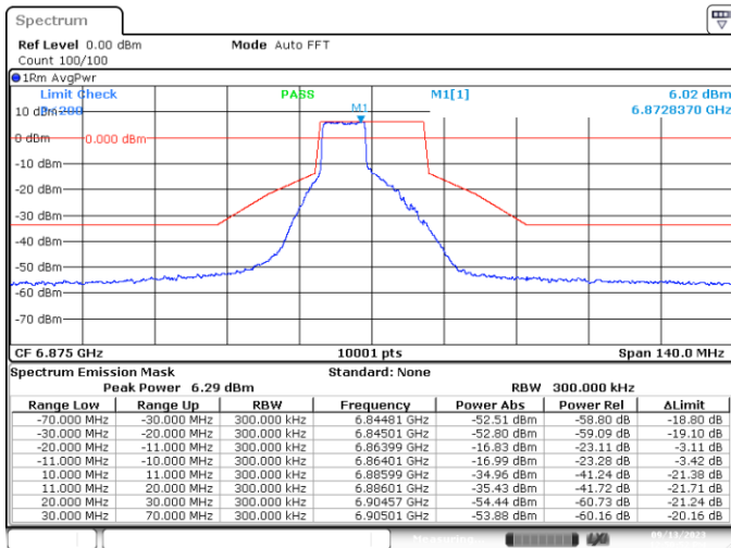
SISO-B, 802.11ax/be20-MCS0, Ch185-8m-53
