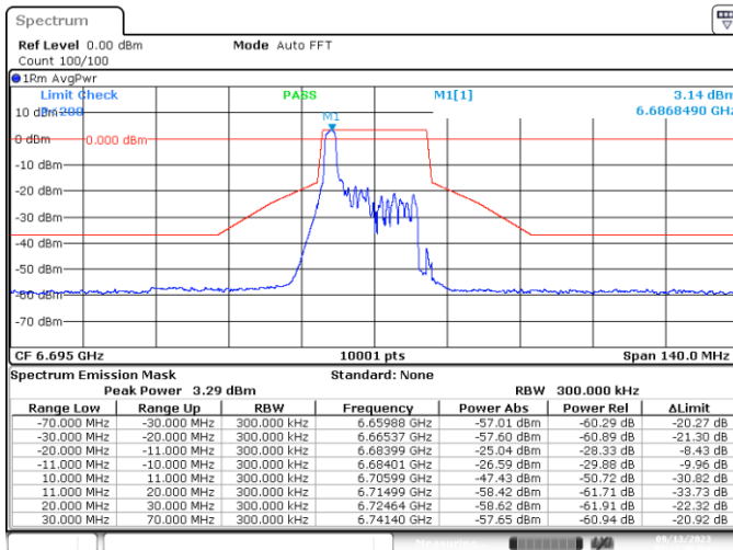
MIMO-B, 802.11ax/be20-MCS0, Ch149-2m-0
