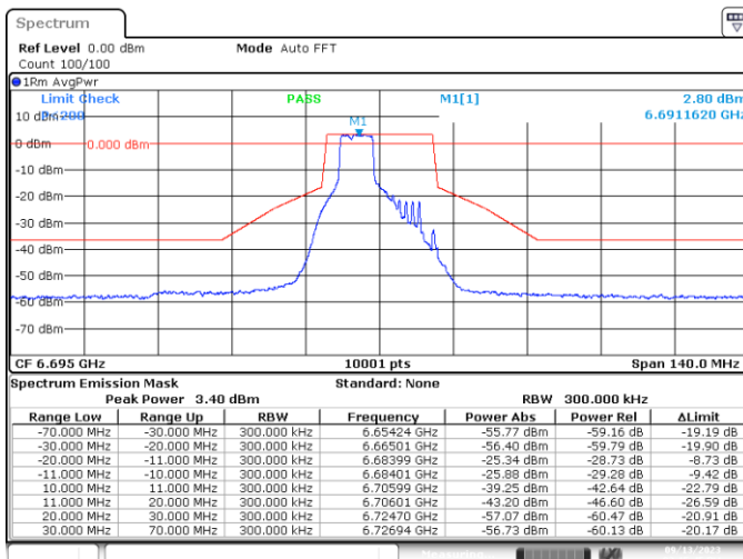
MIMO-B, 802.11ax/be20-MCS0, Ch149-6m-70
