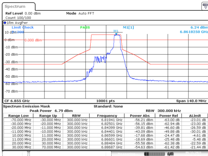
SISO-B, 802.11ax/be20-MCS0, Ch181-4m-37
