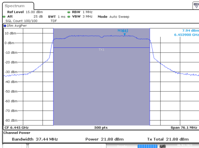
MIMO A-802.11ax/be-40MHz-Ch99-6445MHz-MCS0
