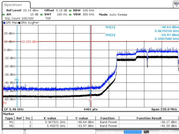
BE-R-LOW, MIMO-A, 802.11ac160-VHT8, Ch114
