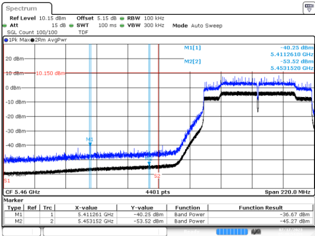
BE-R-LOW, MIMO-A, 802.11ac80-VHT8, Ch106
