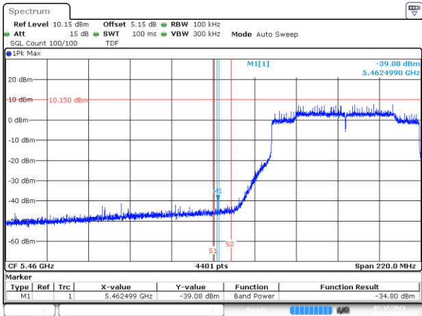
BE-NR-LOW, MIMO-A, 802.11ax/be80-MCS0, Ch106
