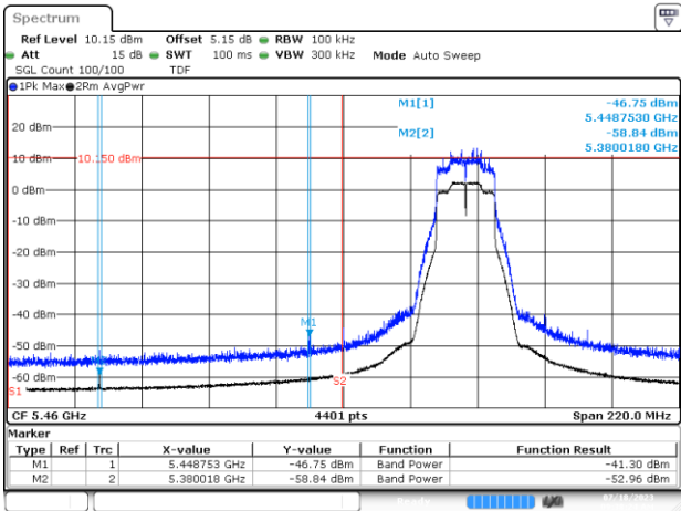
BE-R-LOW, MIMO-A, 802.11ax/be20-MCS0, Ch100
