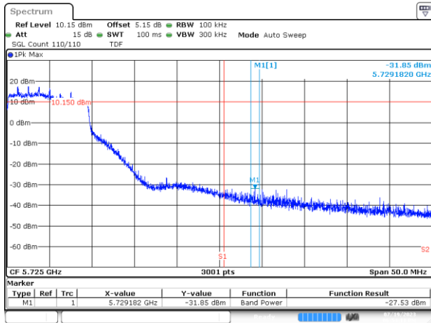
BE-NR-HIGH, SISO-B, 802.11ax/be20-MCS0, Ch140
