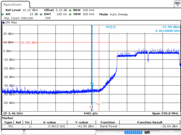
BE-NR-LOW, MIMO-A, 802.11ac160-VHT8, Ch114
