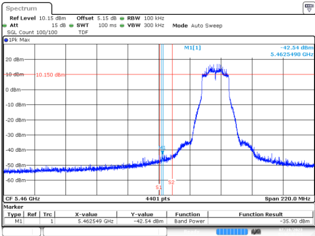
BE-NR-LOW, SISO-B, 802.11ax/be20-MCS0, Ch100
