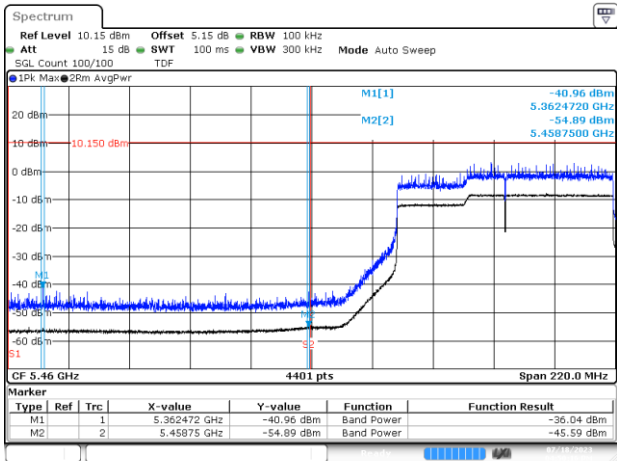
BE-R-LOW, MIMO-B, 802.11ax/be160-MCS0, Ch114
