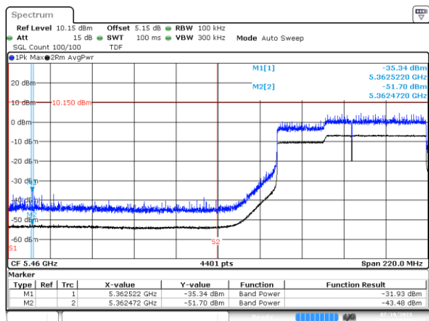
BE-R-LOW, SISO-B, 802.11ax/be160-MCS0, Ch114
