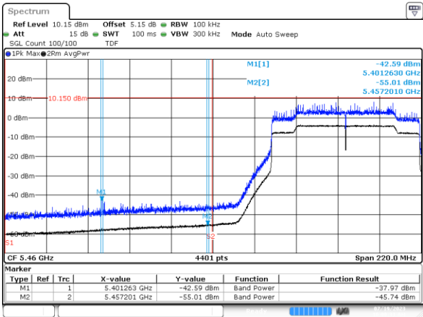
BE-R-LOW, MIMO-B, 802.11ax/be80-MCS0, Ch106
