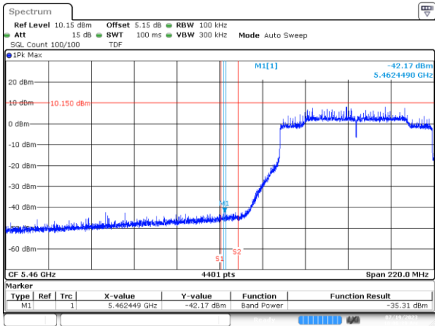
BE-NR-LOW, MIMO-B, 802.11ax/be80-MCS0, Ch106
