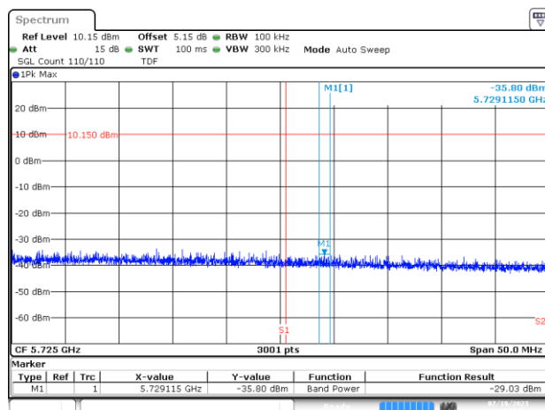
BE-NR-HIGH, SISO-B, 802.11ax/be80-MCS0, Ch122
