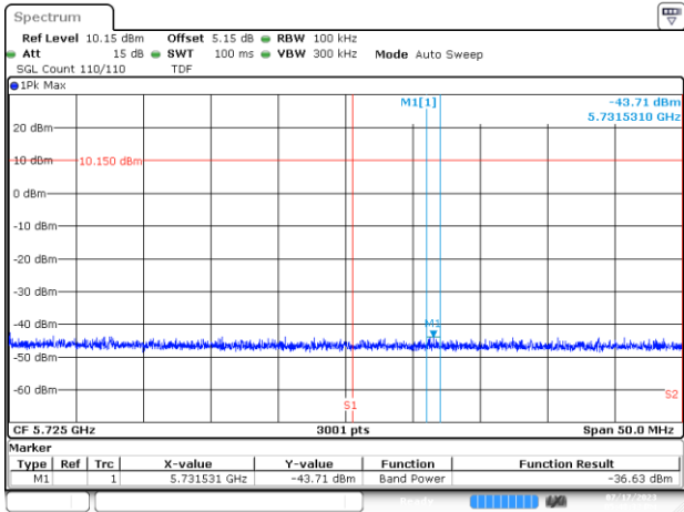
BE-NR-HIGH, MIMO-A, 802.11ax/be160-MCS0, Ch114
