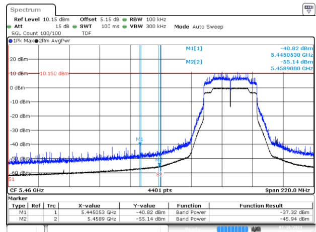
BE-R-LOW, MIMO-B, 802.11ax/be40-MCS0, Ch102
