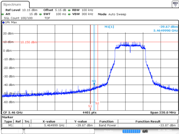
BE-NR-LOW, MIMO-B, 802.11ax/be40-MCS0, Ch102
