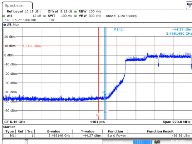
BE-NR-LOW, MIMO-B, 802.11ac160-VHT8, Ch114
