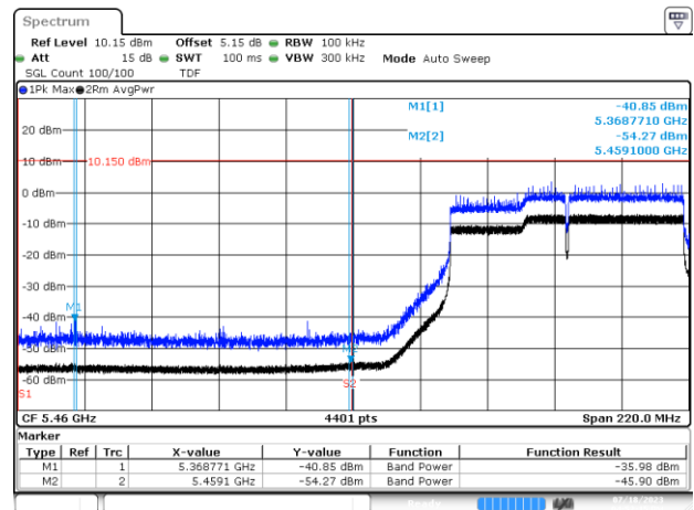
BE-R-LOW, MIMO-B, 802.11ac160-VHT8, Ch114
