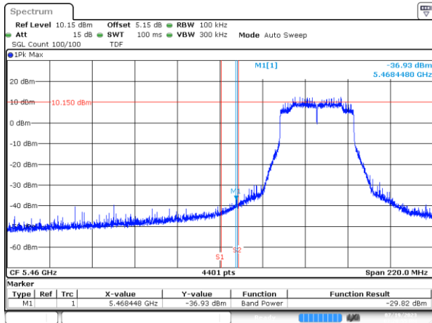
BE-NR-LOW, SISO-B, 802.11ax/be40-MCS0, Ch102
