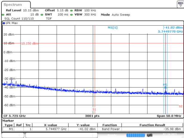
BE-NR-HIGH, MIMO-B, 802.11ax/be40-MCS0, Ch134
