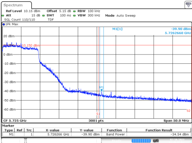
BE-NR-HIGH, MIMO-A, 802.11ax/be20-MCS0, Ch140
