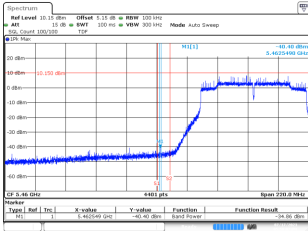
BE-NR-LOW, MIMO-A, 802.11ac80-VHT8, Ch106
