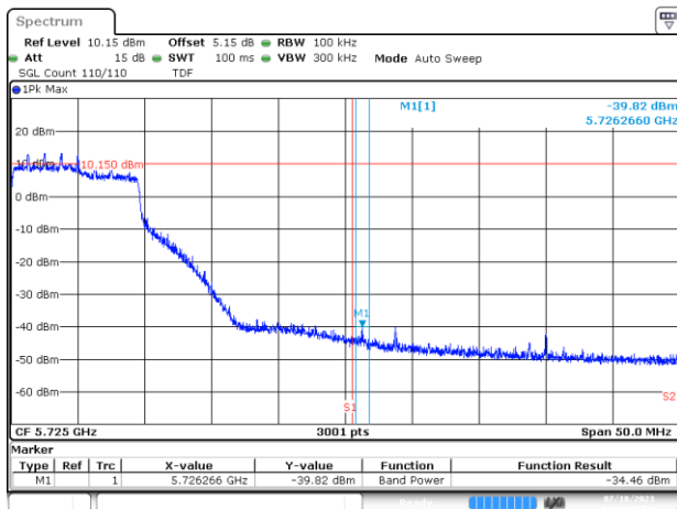
BE-NR-HIGH, MIMO-B, 802.11ax/be20-MCS0, Ch140
