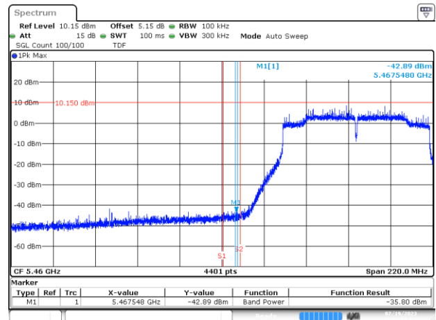
BE-NR-LOW, MIMO-B, 802.11ac80-VHT8, Ch106
