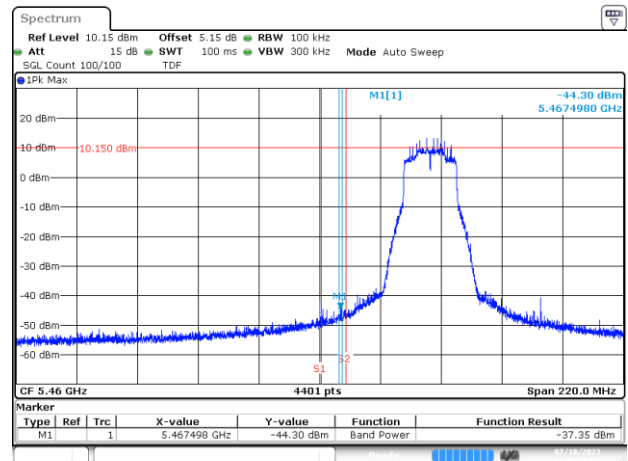
BE-NR-LOW, MIMO-B, 802.11ax/be20-MCS0, Ch100
