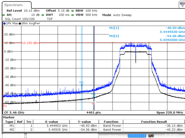
BE-R-LOW, MIMO-A, 802.11ax/be40-MCS0, Ch102
