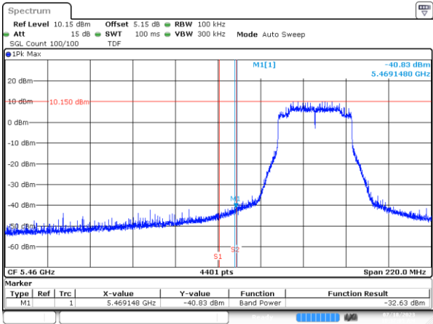
BE-NR-LOW, MIMO-A, 802.11ax/be40-MCS0, Ch102
