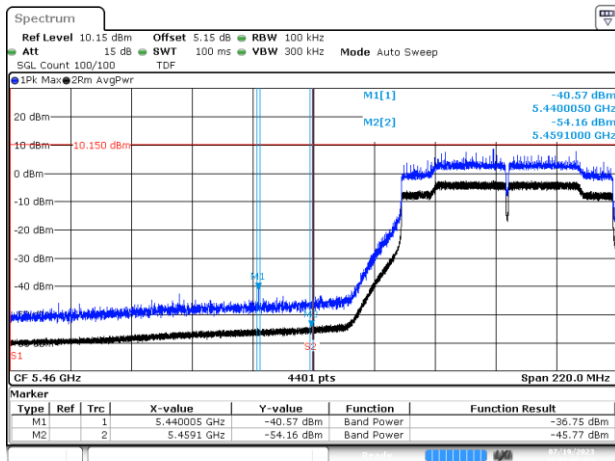
BE-R-LOW, MIMO-B, 802.11ac80-VHT8, Ch106
