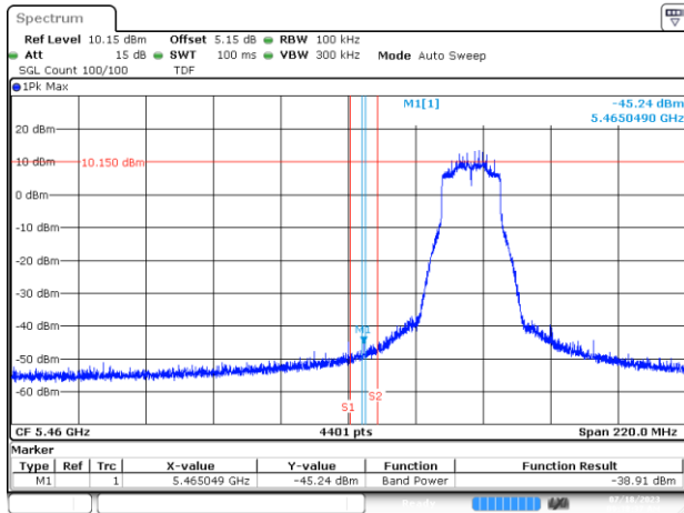
BE-NR-LOW, MIMO-A, 802.11ax/be20-MCS0, Ch100
