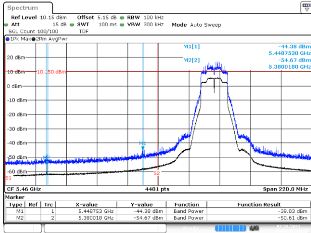
BE-R-LOW, SISO-B, 802.11ax/be20-MCS0, Ch100
