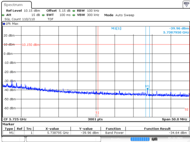
BE-NR-HIGH, MIMO-A, 802.11ax/be40-MCS0, Ch134
