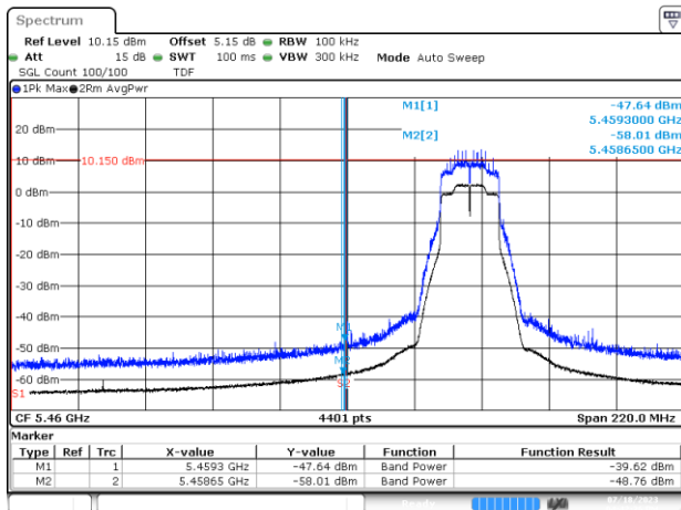
BE-R-LOW, MIMO-B, 802.11ax/be20-MCS0, Ch100
