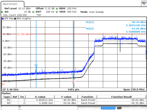
BE-R-LOW, MIMO-A, 802.11ax/be80-MCS0, Ch106
