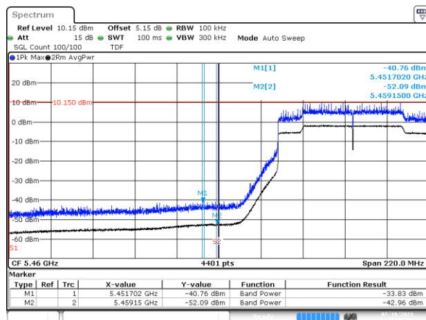
BE-R-LOW, SISO-B, 802.11ax/be80-MCS0, Ch106
