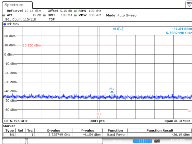
BE-NR-HIGH, MIMO-A, 802.11ac160-VHT8, Ch114
