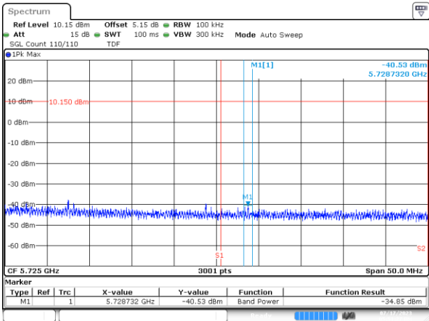
BE-NR-HIGH, MIMO-A, 802.11ac80-VHT8, Ch122
