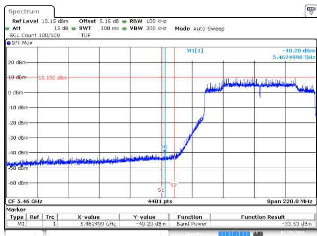
BE-NR-LOW, SISO-B, 802.11ax/be80-MCS0, Ch106
