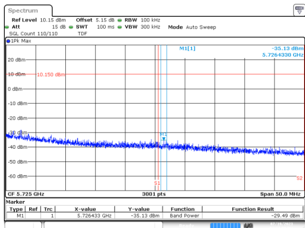
BE-NR-HIGH, SISO-B, 802.11ax/be40-MCS0, Ch134
