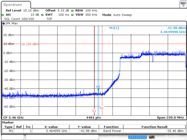
BE-NR-LOW, MIMO-A, 802.11ax/be160-MCS0, Ch114
