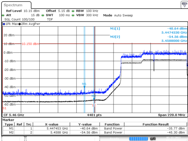
BE-R-LOW, MIMO-A, 802.11ax/be160-MCS0, Ch114
