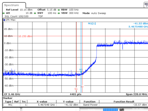
BE-NR-LOW, SISO-B, 802.11ax/be160-MCS0, Ch114
