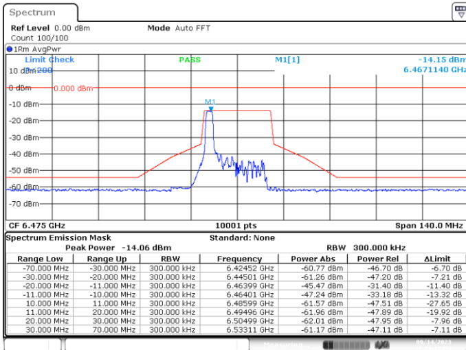
MIMO-A, 802.11ax/be20-MCS0, Ch105-2m-0
