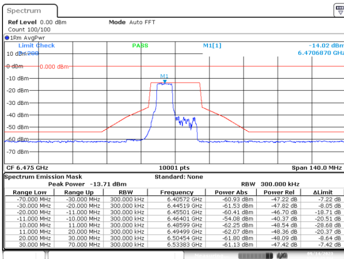
MIMO-A, 802.11ax/be20-MCS0, Ch105-6m-70
