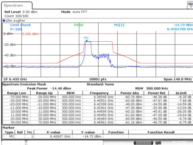
MIMO-A, 802.11ax/be20-MCS0, Ch97-4m-37
