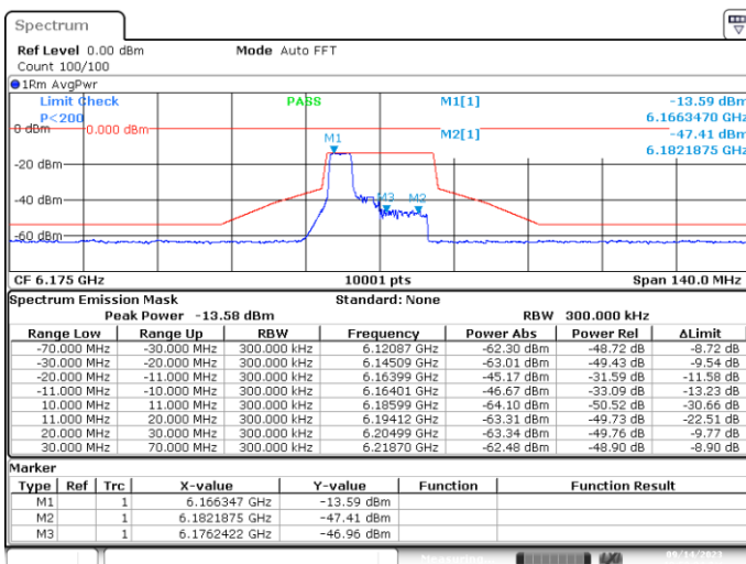
MIMO-B, 802.11ax/be20-MCS0, Ch45-4m-37
