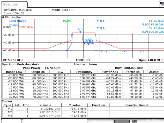
MIMO-A, 802.11ax/be20-MCS0, Ch1-8m-53
