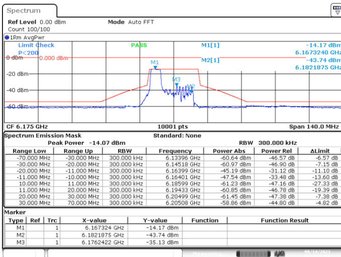
MIMO-A, 802.11ax/be20-MCS0, Ch45-4m-37
