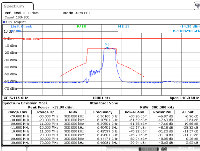
MIMO-A, 802.11ax/be20-MCS0, Ch93-8m-53
