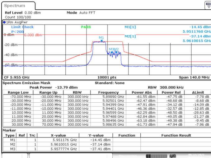
MIMO-B, 802.11ax/be20-MCS0, Ch1-8m-53
