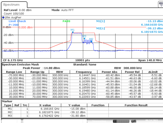
MIMO-A, 802.11ax/be20-MCS0, Ch45-8m-53
