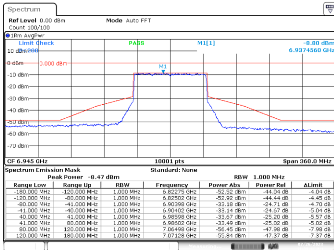
MIMO A-802.11ax/be-80MHz-Ch199-6945MHz-MCS0
