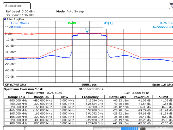
SISO B-802.11be-320MHz-Ch159-6745MHz-MCS0
