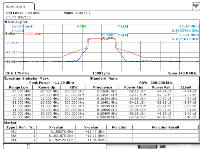
SISO A-802.11ax/be-20MHz-Ch45-6175MHz-MCS0
