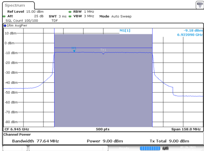
MIMO A-802.11ax/be-80MHz-Ch199-6945MHz-MCS0
