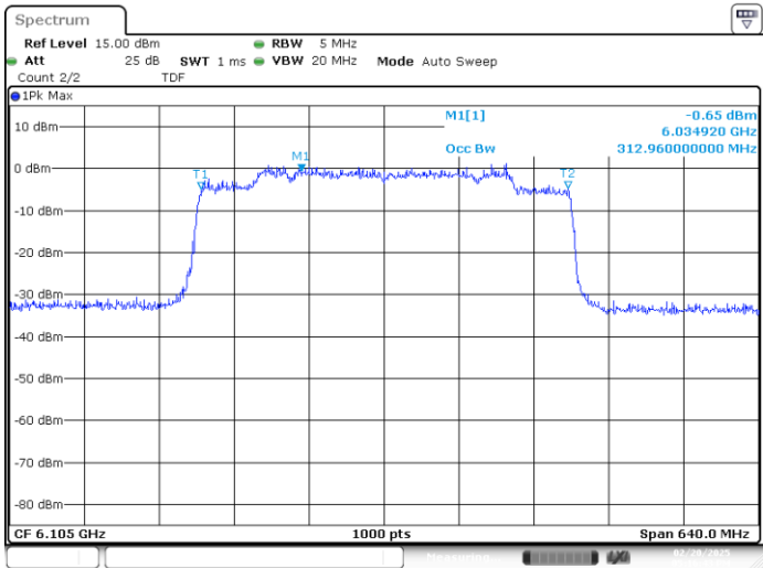
UNII5 MIMO A 802.11be320 ch31 6105MHz 99%
