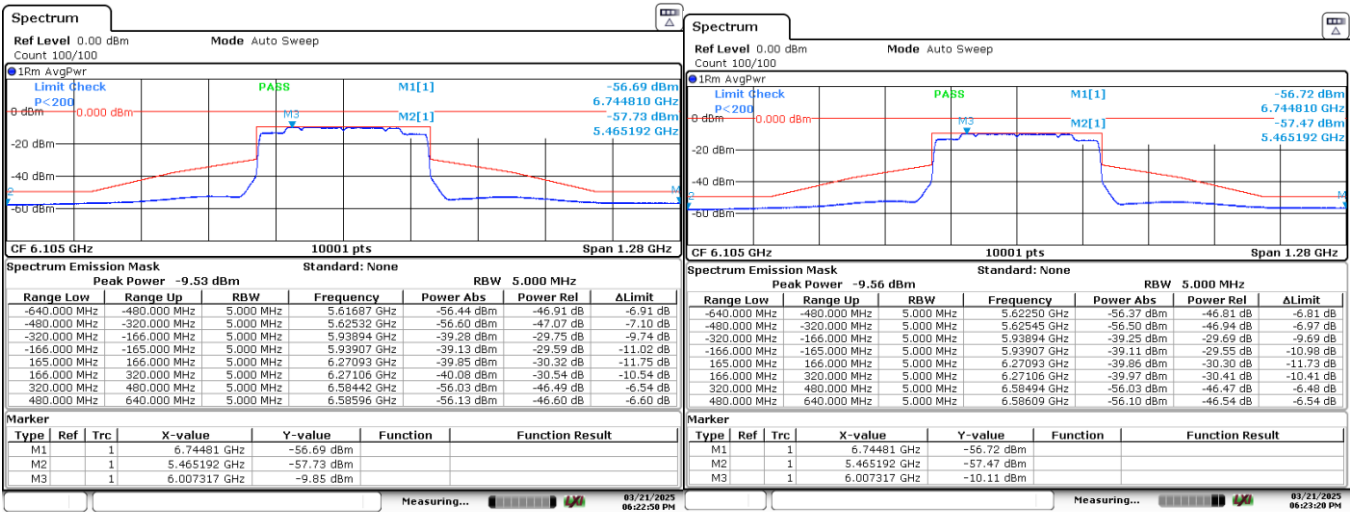
MIMO B-802.11ax/be-320MHz-Ch31-6105MHz-MCS0
