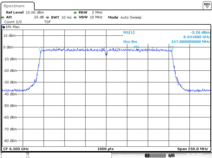
UNII6 MIMO A 802.11ax/be160 ch111 6505MHz 99%
