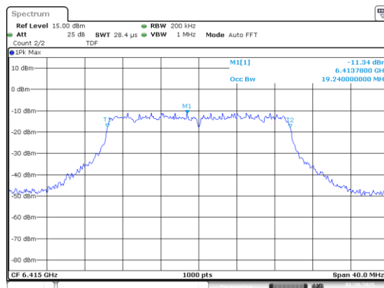
UNII-6 MIMO A 802.11ax/be20 ch93 6415MHz 99%
