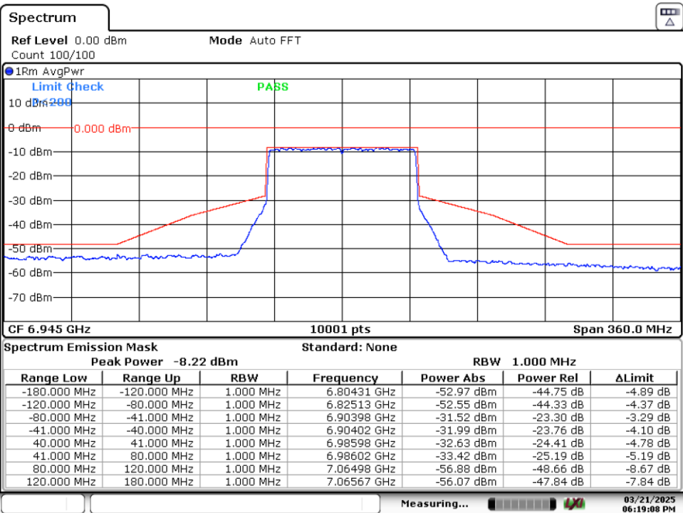
SISO A-802.11ax/be-80MHz-Ch199-6945MHz-MCS0
