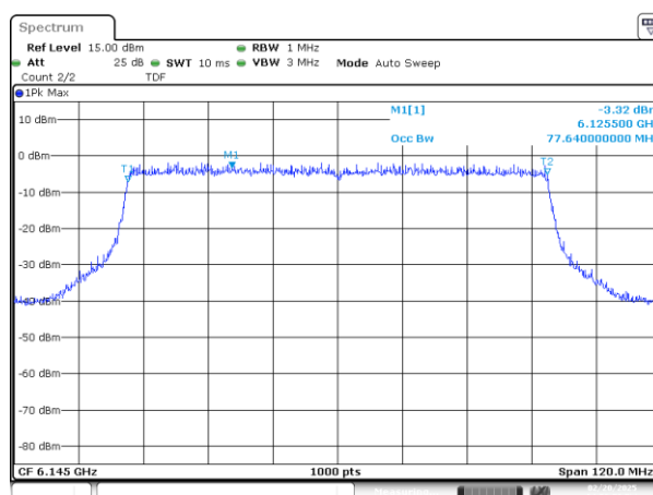
UNII-5 MIMO A 802.11ax/be80 ch39 6145MHz 99%
