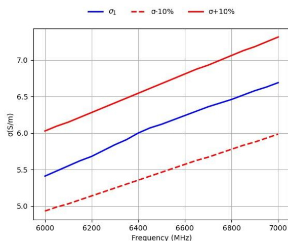
Conductivity 2024-01-19
