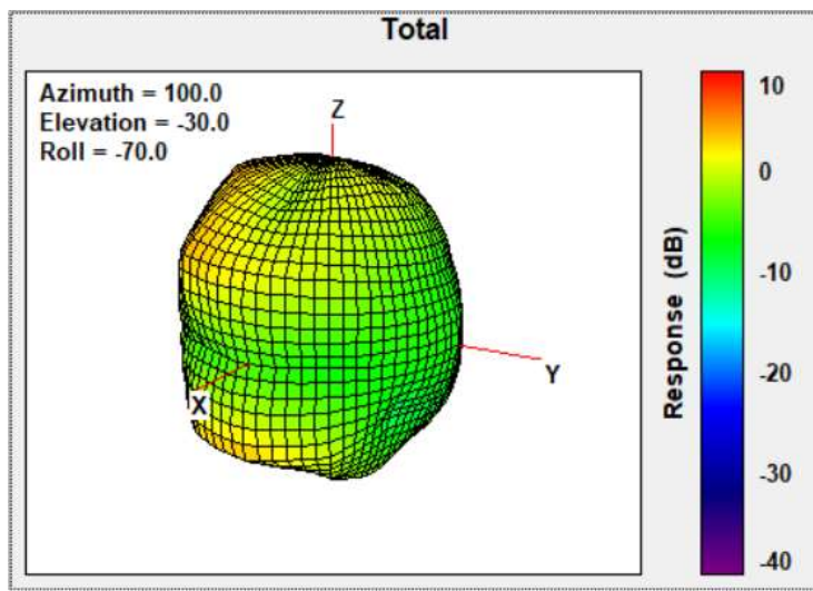
Max Antenna 3D Radiation Pattern 5150-5250 MHz
