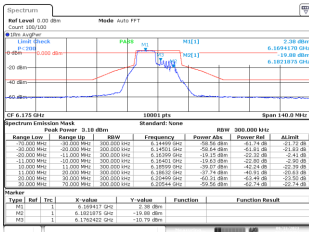
MIMO-A, 802.11ax/be20-MCS0, Ch45-8m-53
