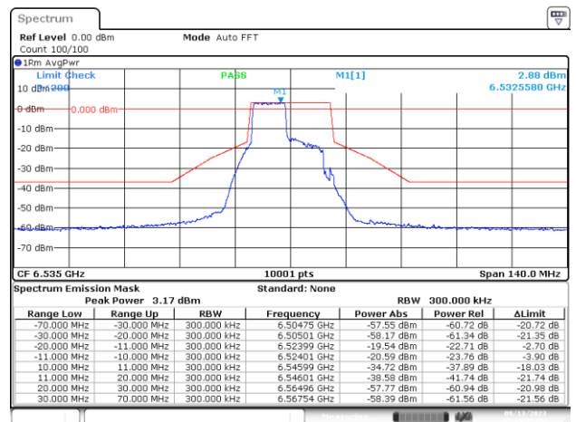
MIMO-A, 802.11ax/be20-MCS0, Ch117-8m-53
