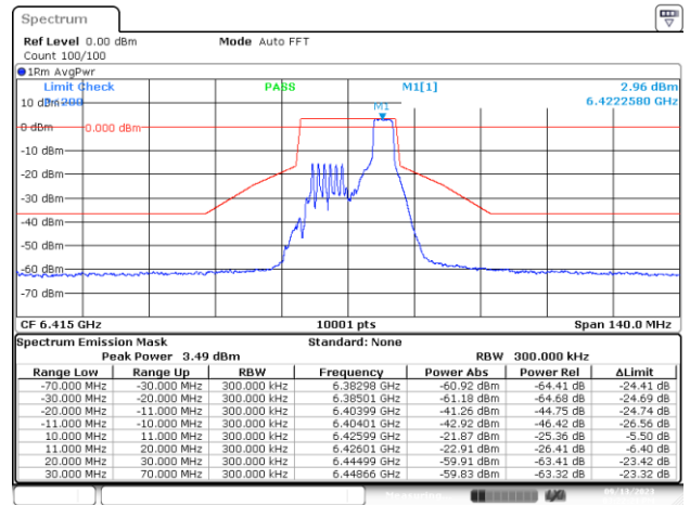
MIMO-A, 802.11ax/be20-MCS0, Ch93-4m-37
