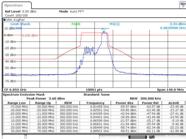
MIMO-A, 802.11ax/be20-MCS0, Ch181-4m-37
