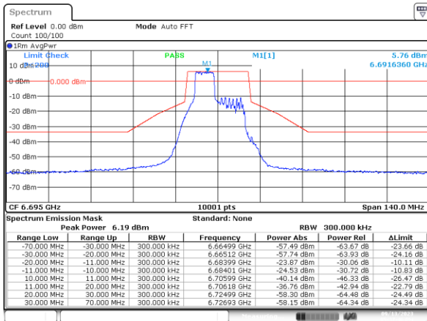
SISO-B, 802.11ax/be20-MCS0, Ch149-6m-70
