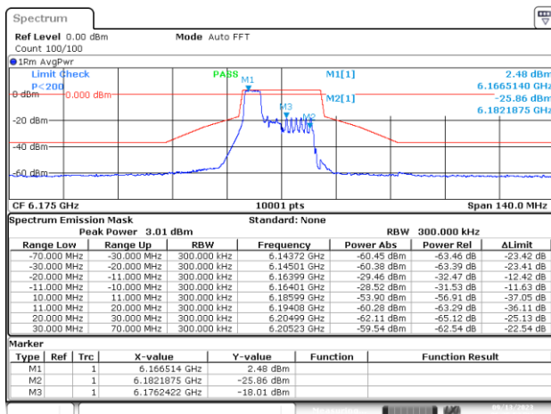
MIMO-B, 802.11ax/be20-MCS0, Ch45-4m-37
