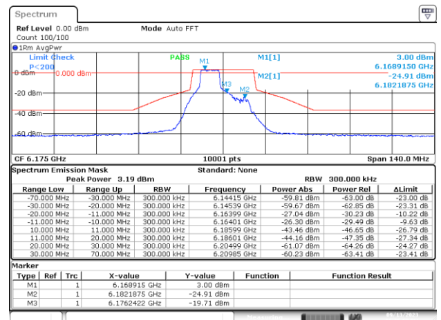
MIMO-B, 802.11ax/be20-MCS0, Ch45-6m-70
