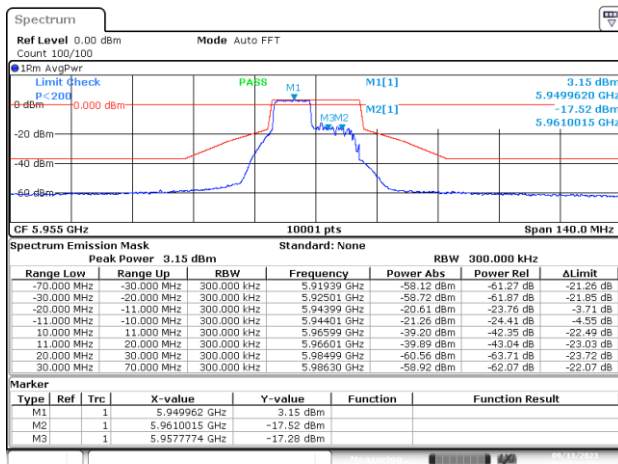
MIMO-B, 802.11ax/be20-MCS0, Ch1-8m-53
