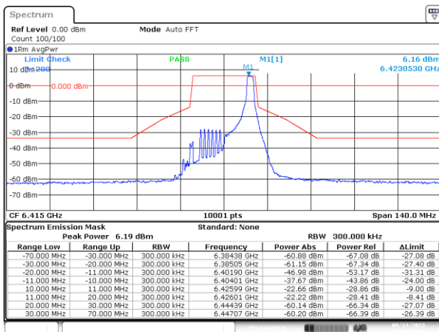
SISO-B, 802.11ax/be20-MCS0, Ch93-2m-0
