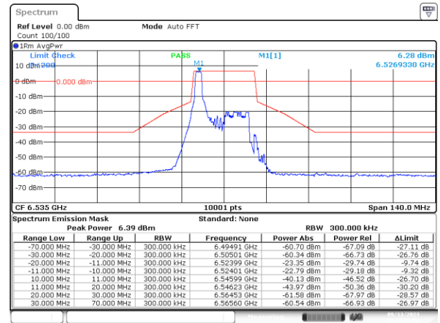
SISO-B, 802.11ax/be20-MCS0, Ch117-2m-0
