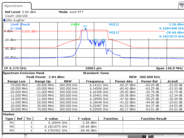
MIMO-A, 802.11ax/be20-MCS0, Ch45-4m-37
