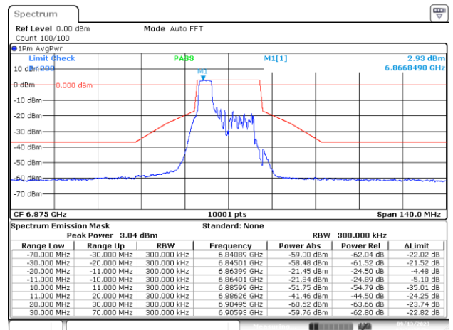
MIMO-A, 802.11ax/be20-MCS0, Ch185-4m-37
