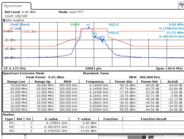
SISO-B, 802.11ax/be20-MCS0, Ch45-8m-53
