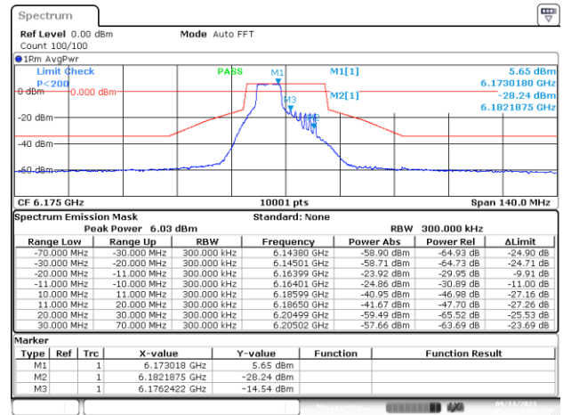
SISO-B, 802.11ax/be20-MCS0, Ch45-6m-70
