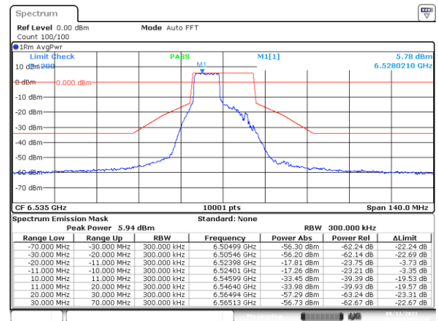
SISO-B, 802.11ax/be20-MCS0, Ch117-8m-53
