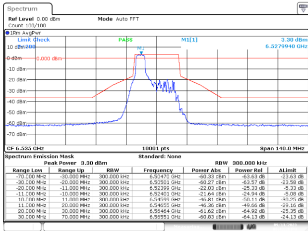
MIMO-B, 802.11ax/be20-MCS0, Ch117-4m-37
