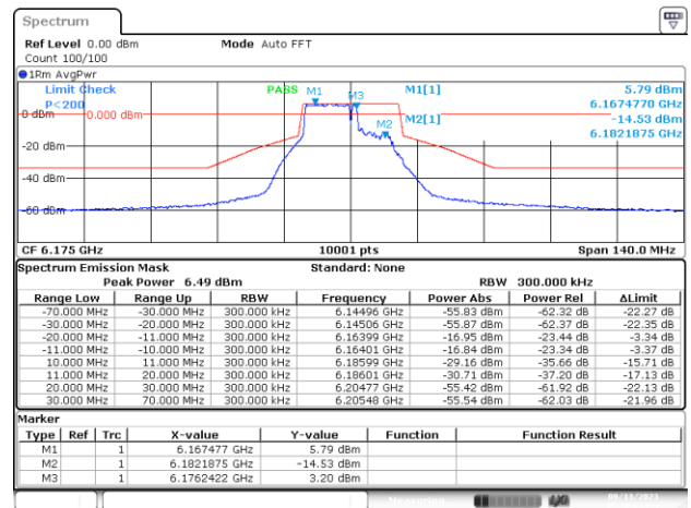
SISO-B, 802.11ax/be20-MCS0, Ch45-10m-82
