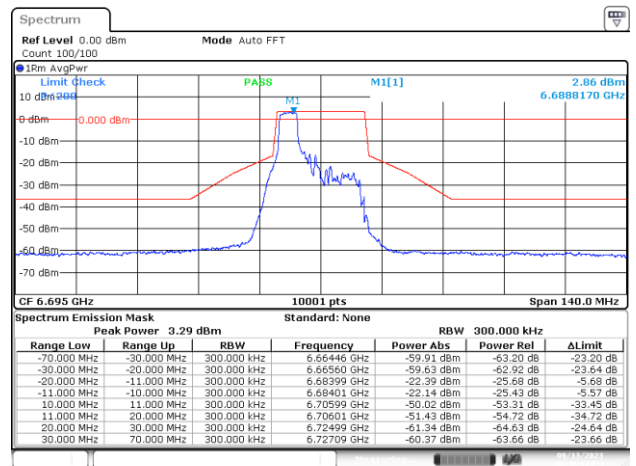
MIMO-B, 802.11ax/be20-MCS0, Ch149-4m-37
