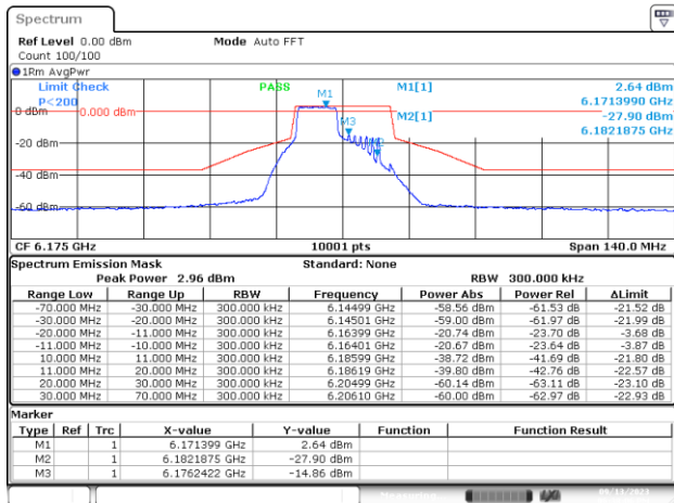
MIMO-B, 802.11ax/be20-MCS0, Ch45-8m-53
