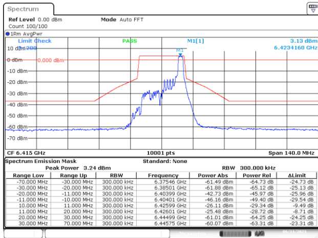
MIMO-A, 802.11ax/be20-MCS0, Ch93-2m-0
