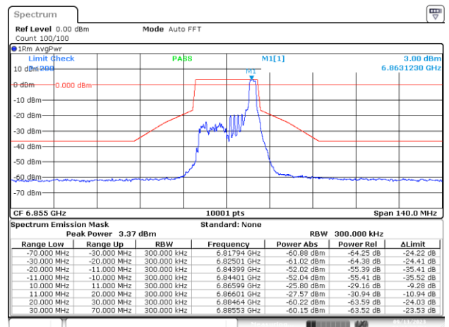
MIMO-A, 802.11ax/be20-MCS0, Ch181-2m-0
