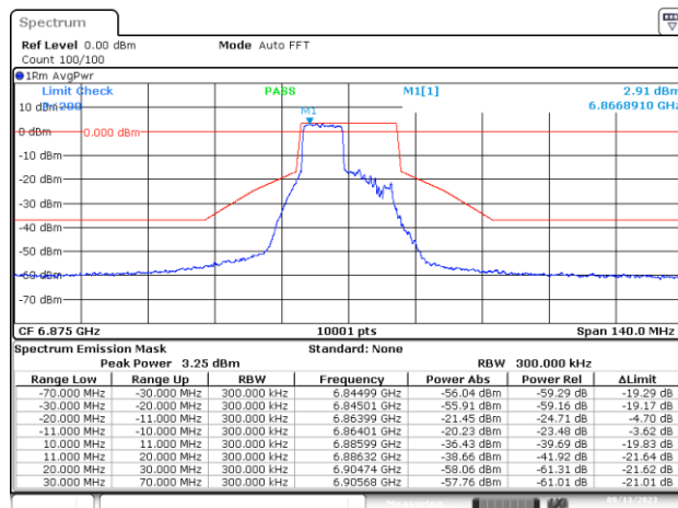
MIMO-A, 802.11ax/be20-MCS0, Ch185-8m-53
