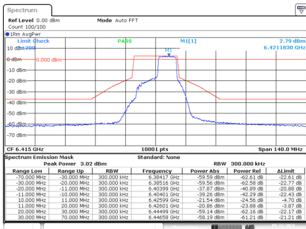
MIMO-B, 802.11ax/be20-MCS0, Ch93-8m-53
