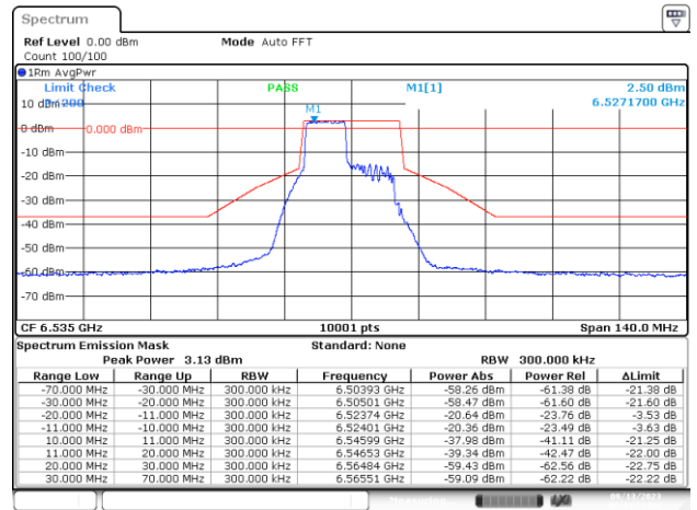
MIMO-B, 802.11ax/be20-MCS0, Ch117-8m-53
