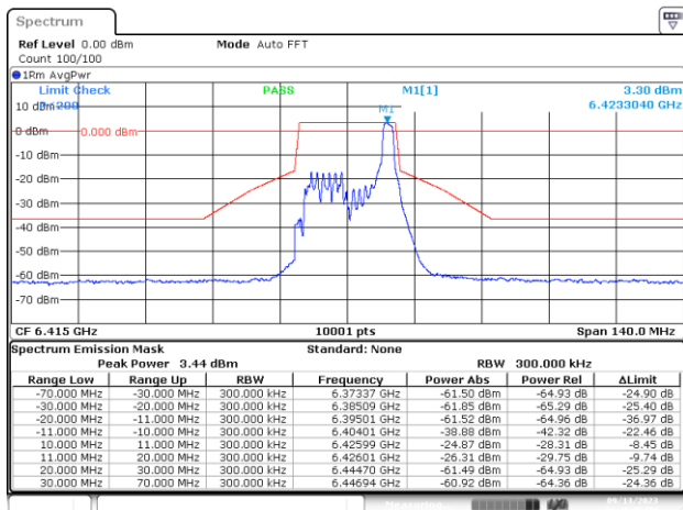
MIMO-B, 802.11ax/be20-MCS0, Ch93-2m-0
