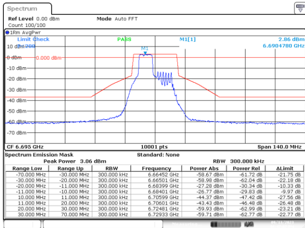
MIMO-B, 802.11ax/be20-MCS0, Ch149-6m-70
