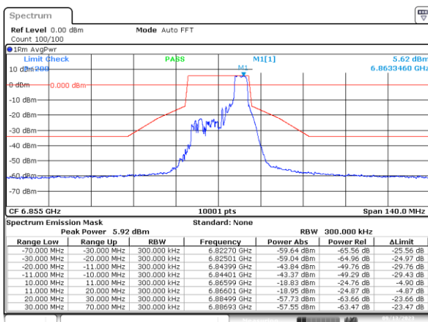
SISO-B, 802.11ax/be20-MCS0, Ch181-4m-37
