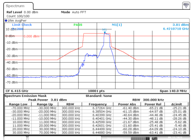
MIMO-B, 802.11ax/be20-MCS0, Ch93-4m-37
