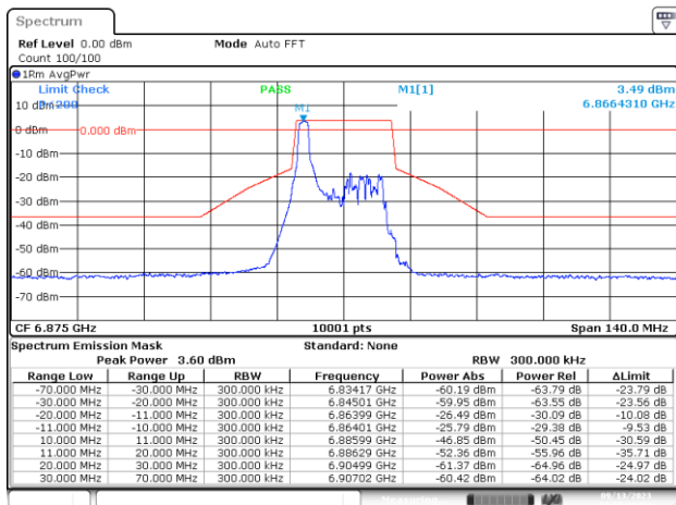
MIMO-A, 802.11ax/be20-MCS0, Ch185-2m-0
