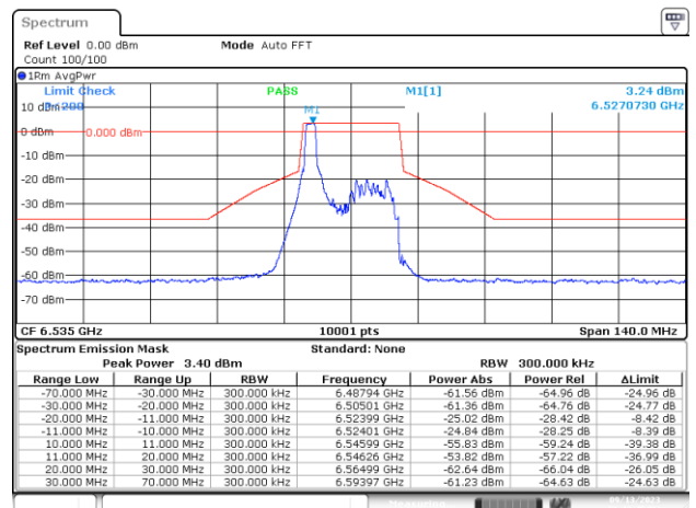
MIMO-B, 802.11ax/be20-MCS0, Ch117-2m-0
