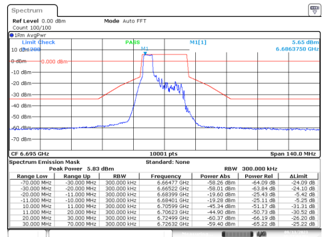
SISO-B, 802.11ax/be20-MCS0, Ch149-4m-37
