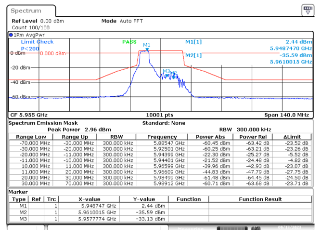
MIMO-A, 802.11ax/be20-MCS0, Ch1-4m-37
