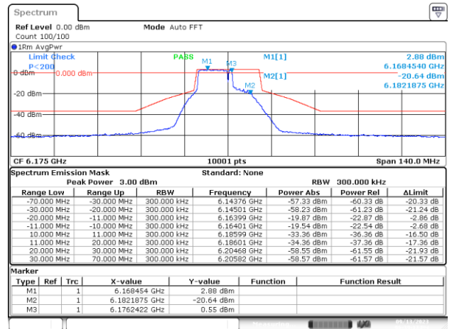
MIMO-B, 802.11ax/be20-MCS0, Ch45-10m-82
