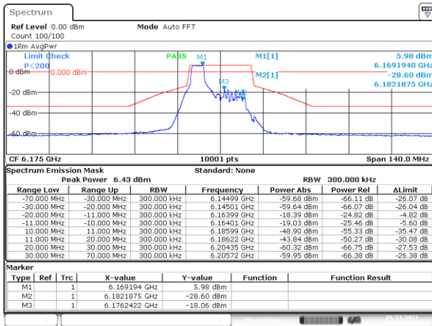
SISO-B, 802.11ax/be20-MCS0, Ch45-4m-37
