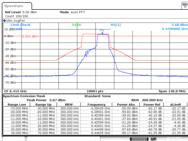
MIMO-A, 802.11ax/be20-MCS0, Ch93-8m-53
