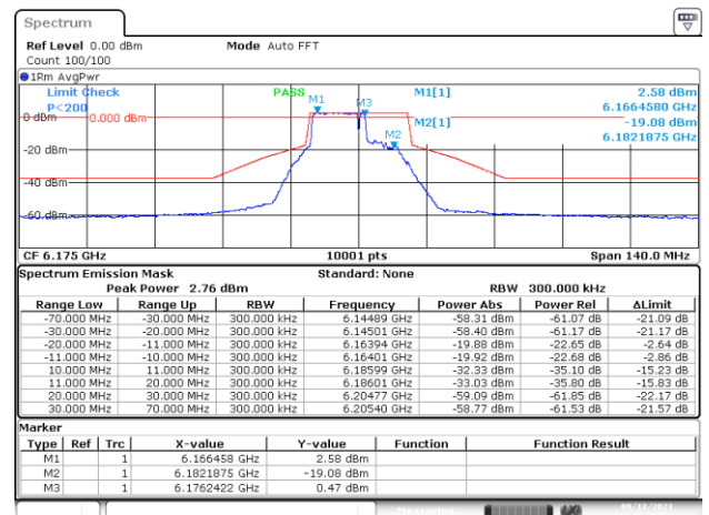
MIMO-A, 802.11ax/be20-MCS0, Ch45-10m-82
