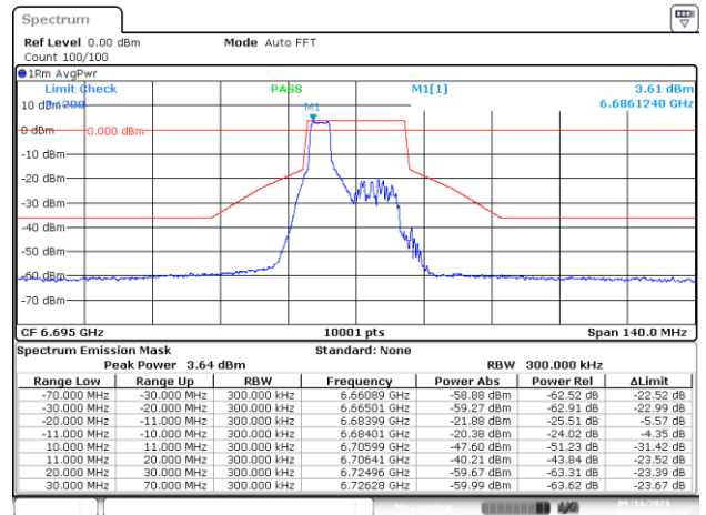
MIMO-A, 802.11ax/be20-MCS0, Ch149-4m-37
