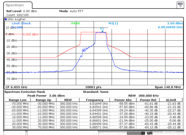
MIMO-A, 802.11ax/be20-MCS0, Ch181-8m-53
