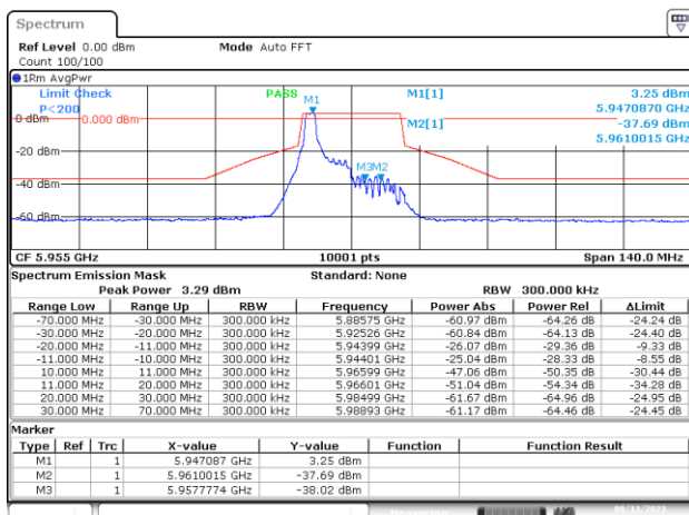
MIMO-A, 802.11ax/be20-MCS0, Ch1-2m-0
