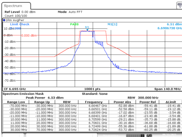
SISO-B, 802.11ax/be20-MCS0, Ch149-10m-82
