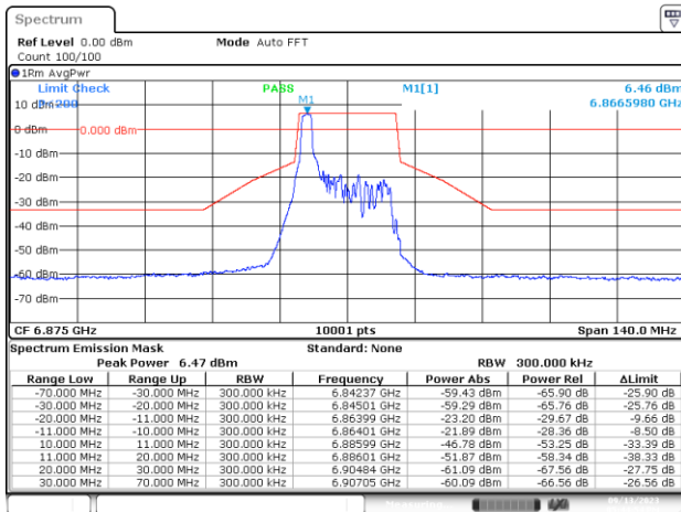
SISO-B, 802.11ax/be20-MCS0, Ch185-2m-0
