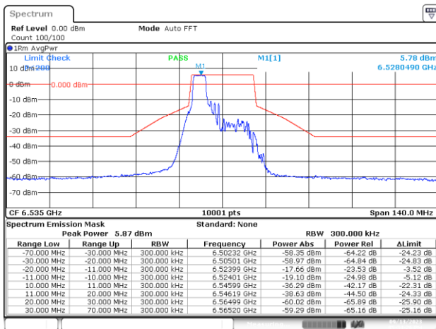
SISO-B, 802.11ax/be20-MCS0, Ch117-4m-37
