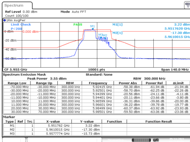
MIMO-A, 802.11ax/be20-MCS0, Ch1-8m-53
