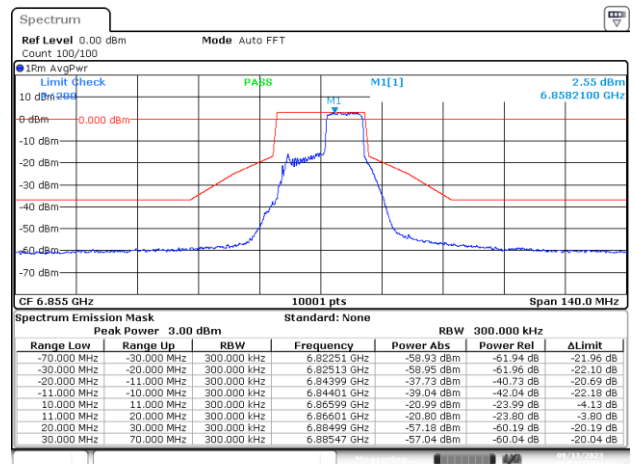
MIMO-B, 802.11ax/be20-MCS0, Ch181-8m-53
