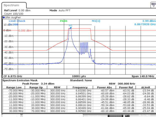
MIMO-B, 802.11ax/be20-MCS0, Ch185-2m-0
