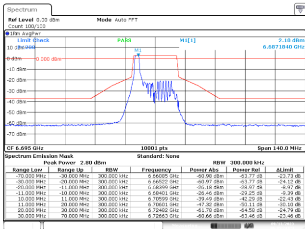
MIMO-B, 802.11ax/be20-MCS0, Ch149-2m-0
