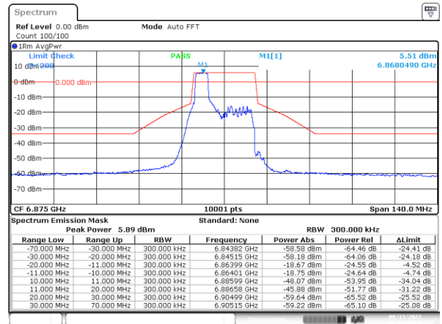
SISO-B, 802.11ax/be20-MCS0, Ch185-4m-37
