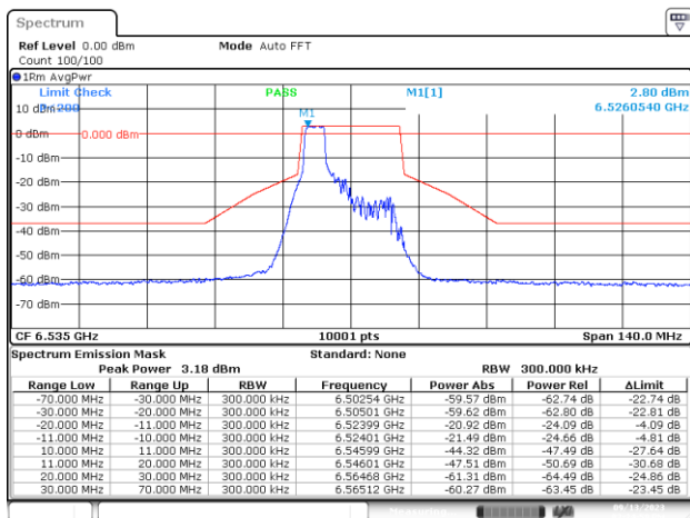
MIMO-A, 802.11ax/be20-MCS0, Ch117-4m-37
