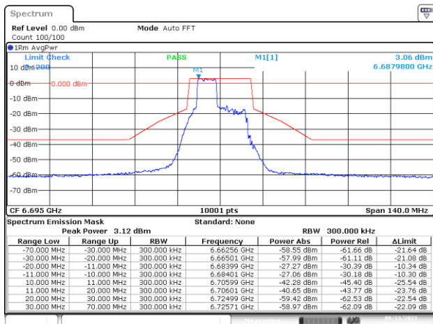
MIMO-A, 802.11ax/be20-MCS0, Ch149-6m-70
