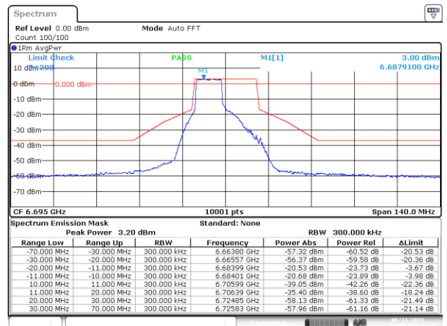
MIMO-A, 802.11ax/be20-MCS0, Ch149-8m-53
