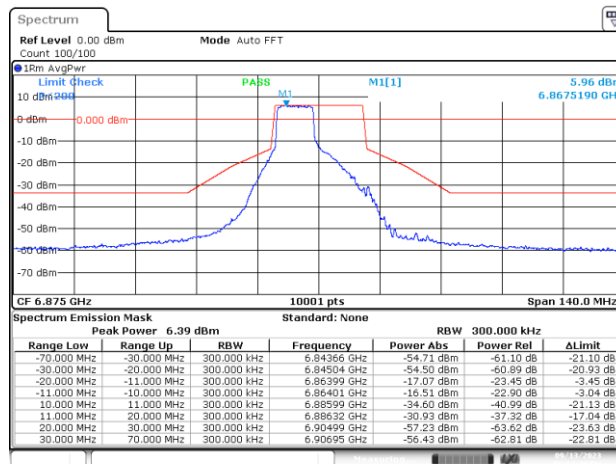
SISO-B, 802.11ax/be20-MCS0, Ch185-8m-53
