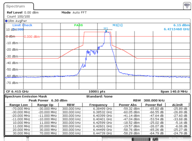
SISO-B, 802.11ax/be20-MCS0, Ch93-4m-37
