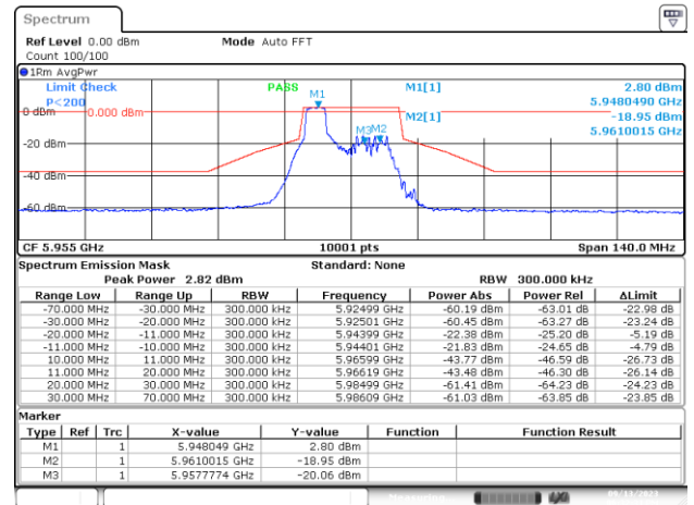
MIMO-B, 802.11ax/be20-MCS0, Ch1-4m-37
