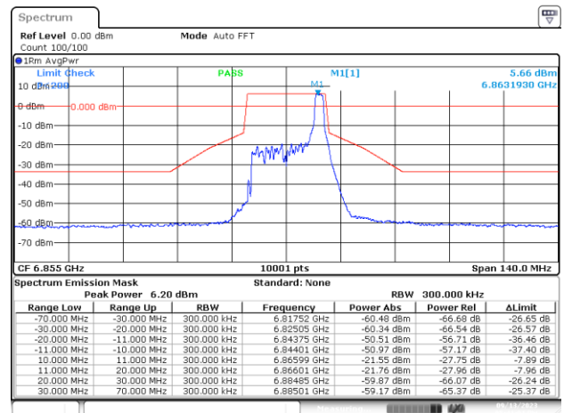
SISO-B, 802.11ax/be20-MCS0, Ch181-2m-0
