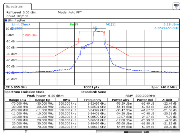
SISO-B, 802.11ax/be20-MCS0, Ch181-8m-53
