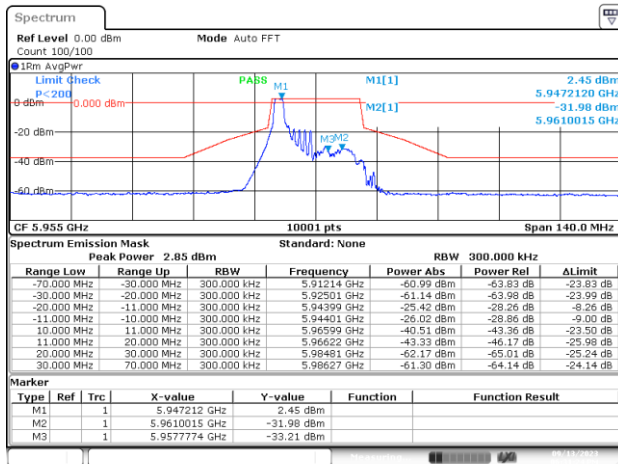
MIMO-B, 802.11ax/be20-MCS0, Ch1-2m-0
