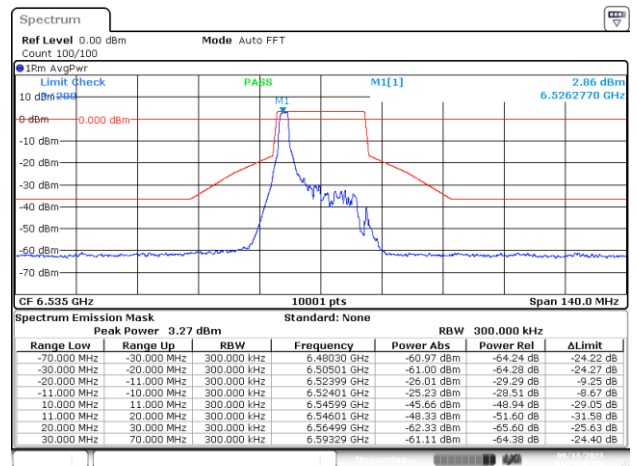
MIMO-A, 802.11ax/be20-MCS0, Ch117-2m-0
