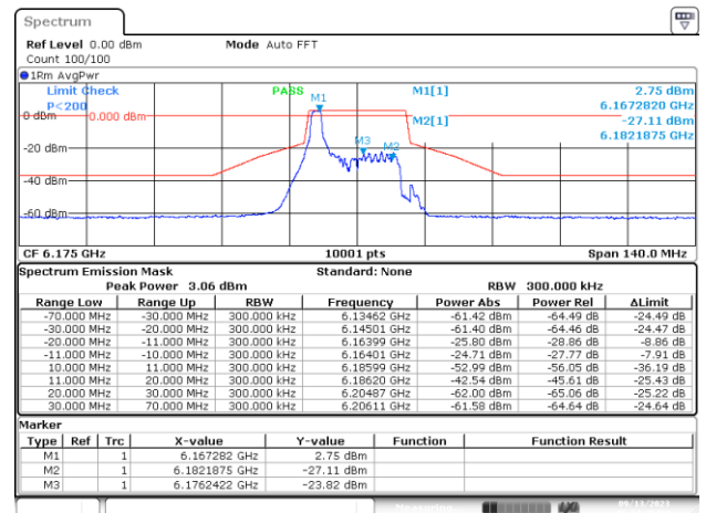
MIMO-B, 802.11ax/be20-MCS0, Ch45-2m-0
