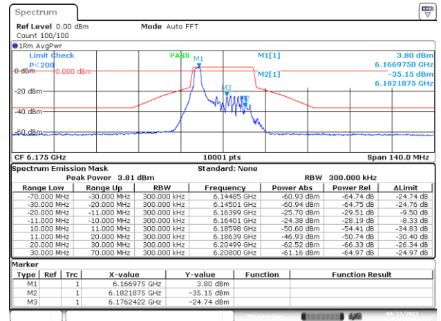
MIMO-A, 802.11ax/be20-MCS0, Ch45-2m-0
