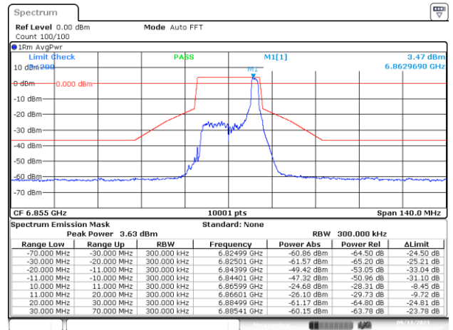
MIMO-B, 802.11ax/be20-MCS0, Ch181-2m-0
