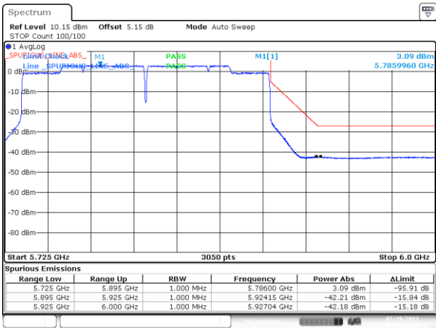
BE-NR-HIGH, SISO-A, 802.11ax/be160-MCS0, Ch163
