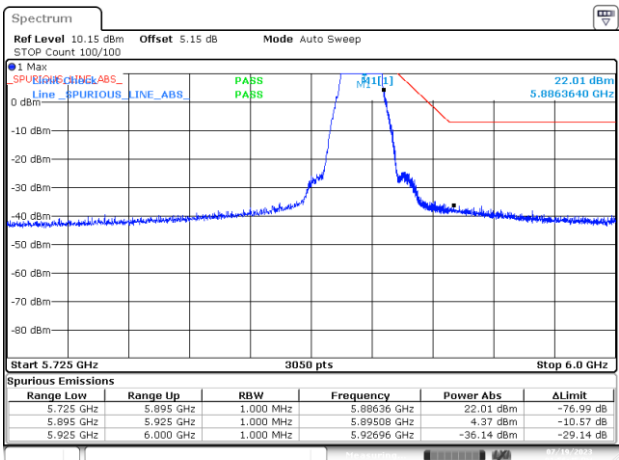
BE-NR-HIGH-PEAK, SISO-A, 802.11n20-HT0, Ch177
