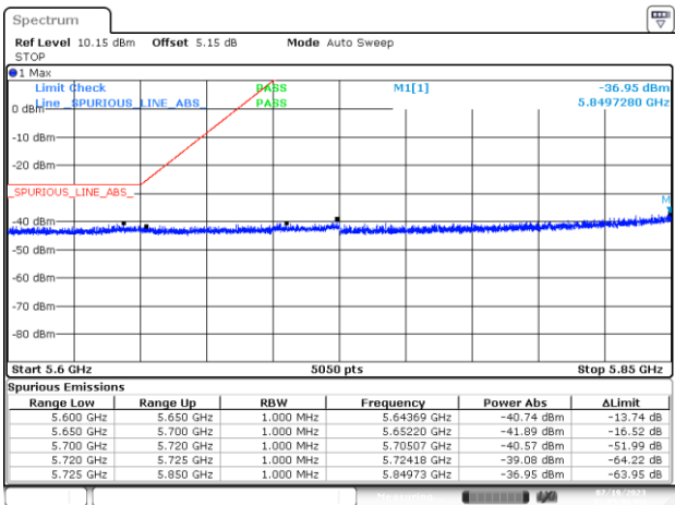
BE-NR-LOW, SISO-A, 802.11ax/be20-MCS0, Ch177
