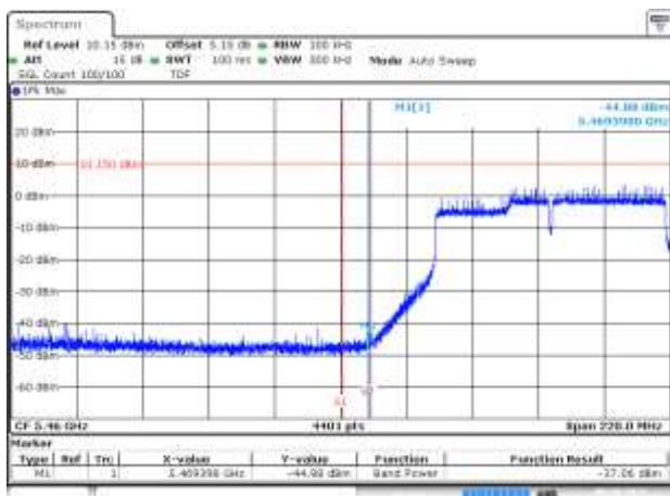
BE-NR-LOW, MIMO-A, 802.11ac160-VHT0, Ch114
