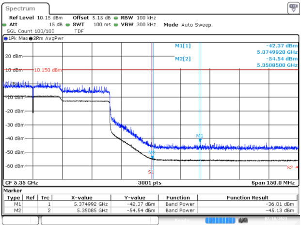
BE-R-HIGH, MIMO-B, 802.11ax/be160-MCS0, Ch50
