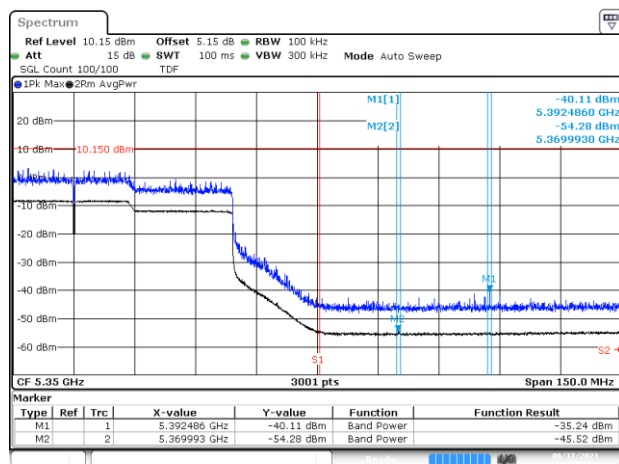
BE-R-HIGH, MIMO-A, 802.11ax/be160-MCS0, Ch50
